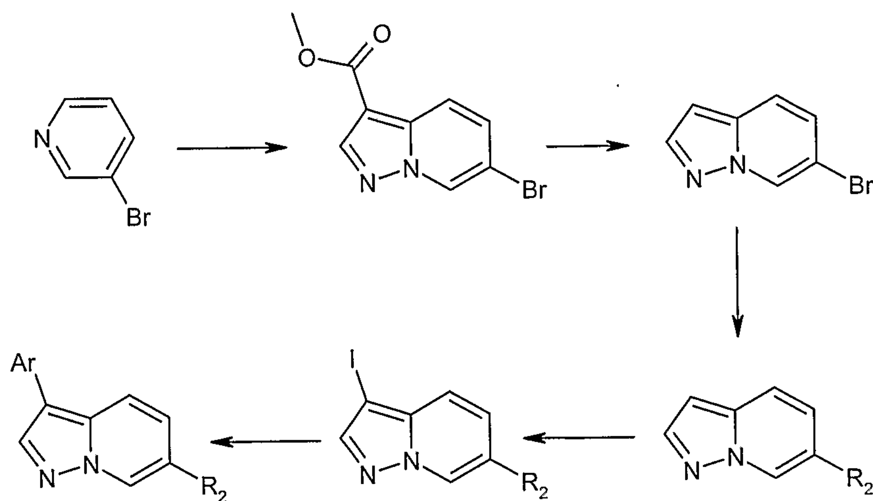
Scheme 7
