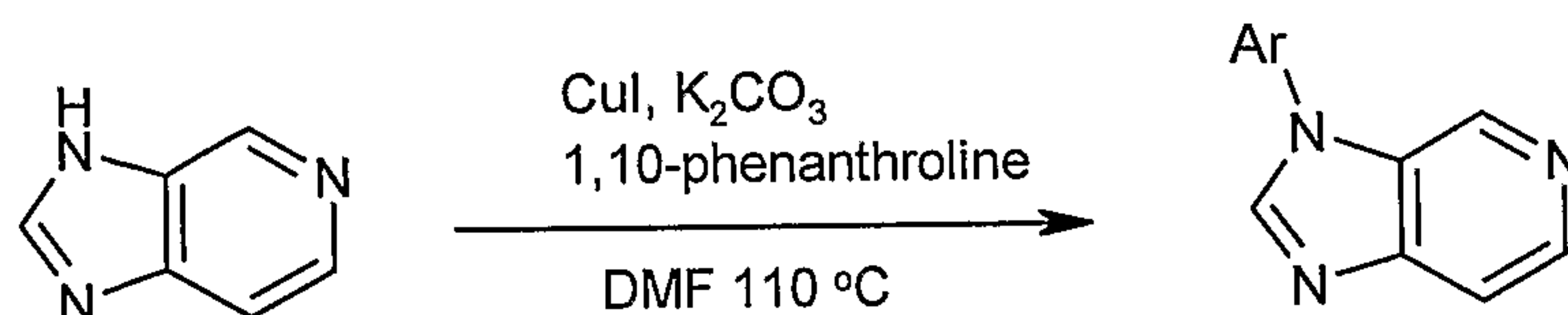
Scheme 10
