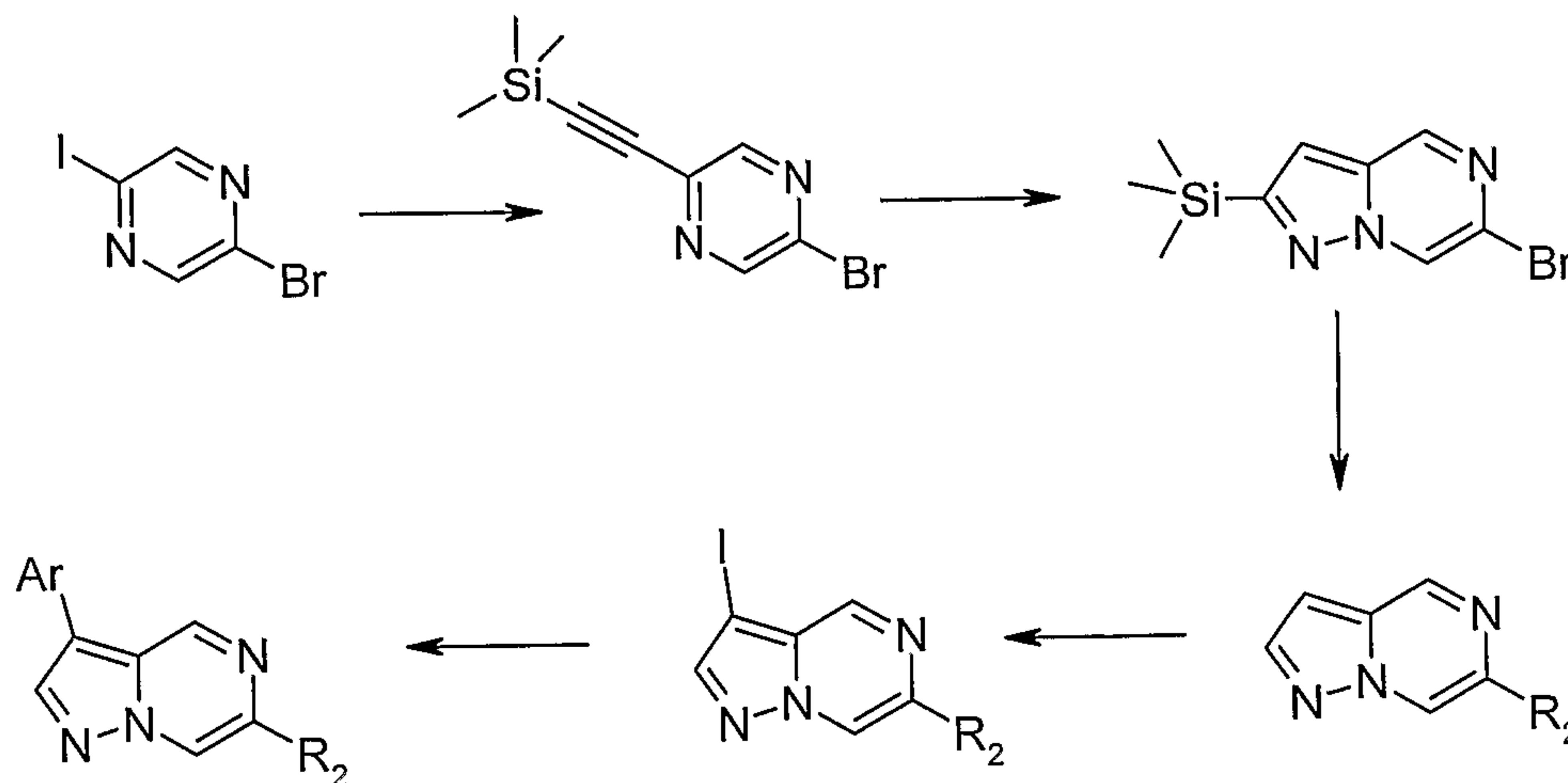
Scheme 6
