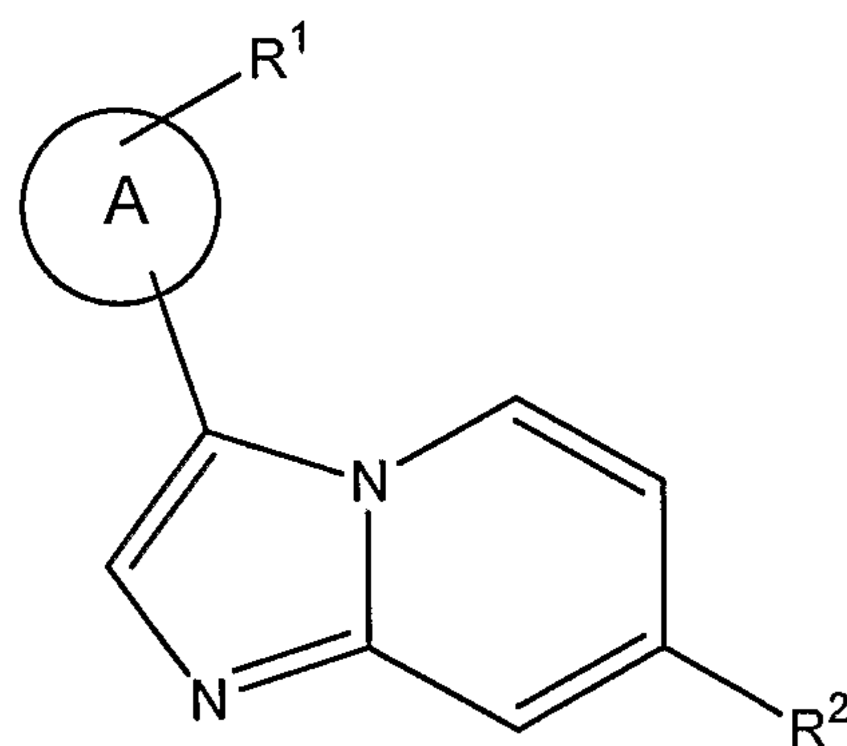
(Ic)
