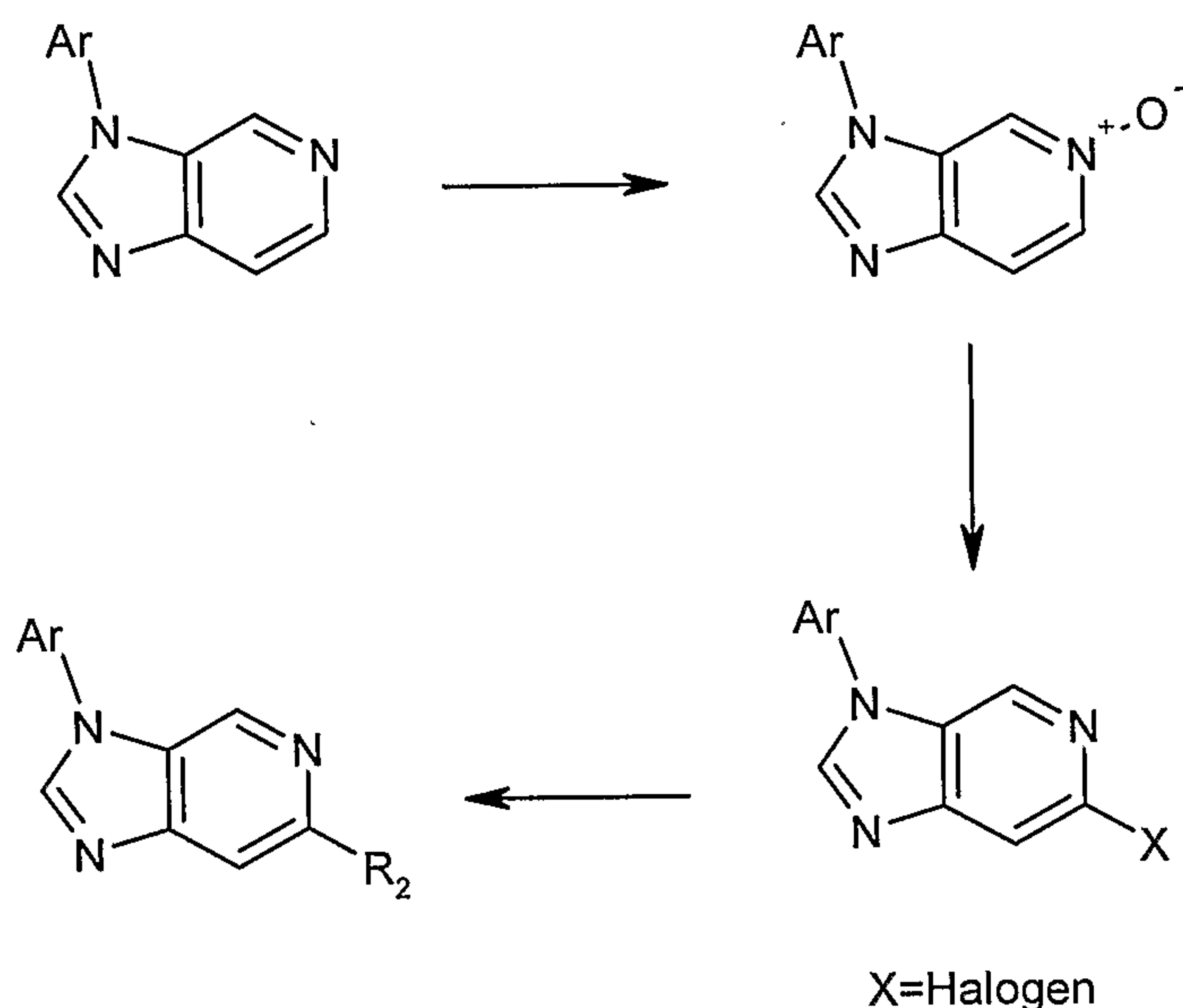
Scheme 11
