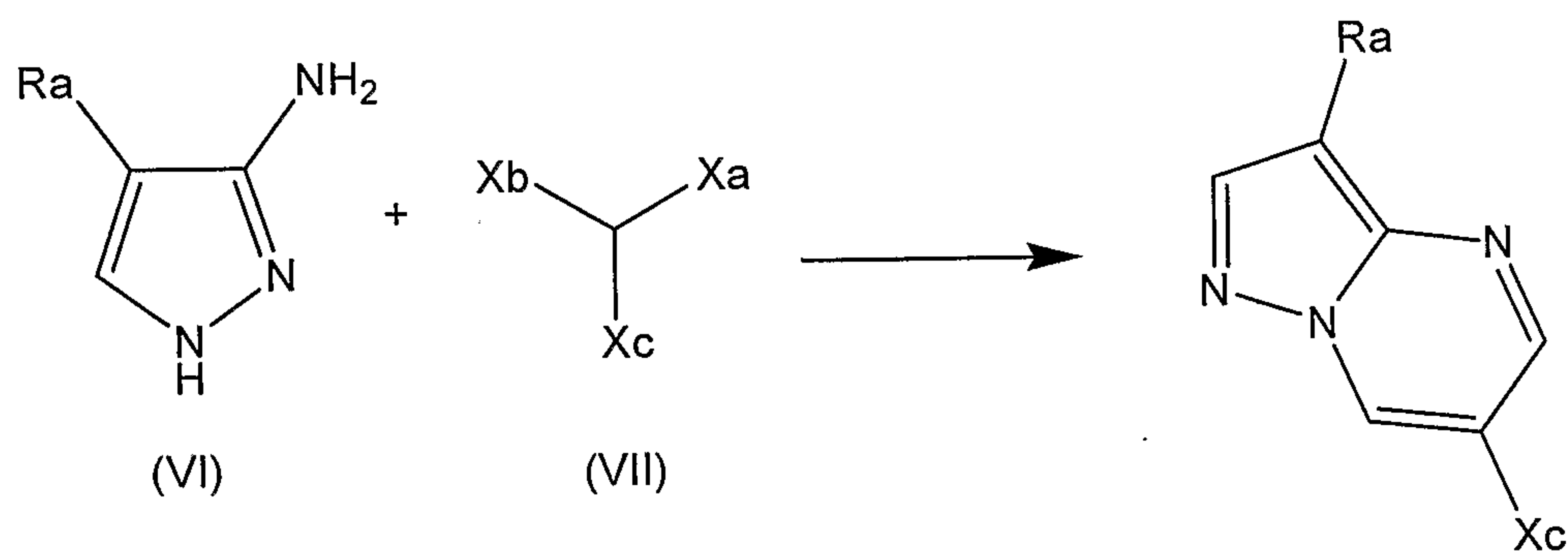
Scheme 5A
