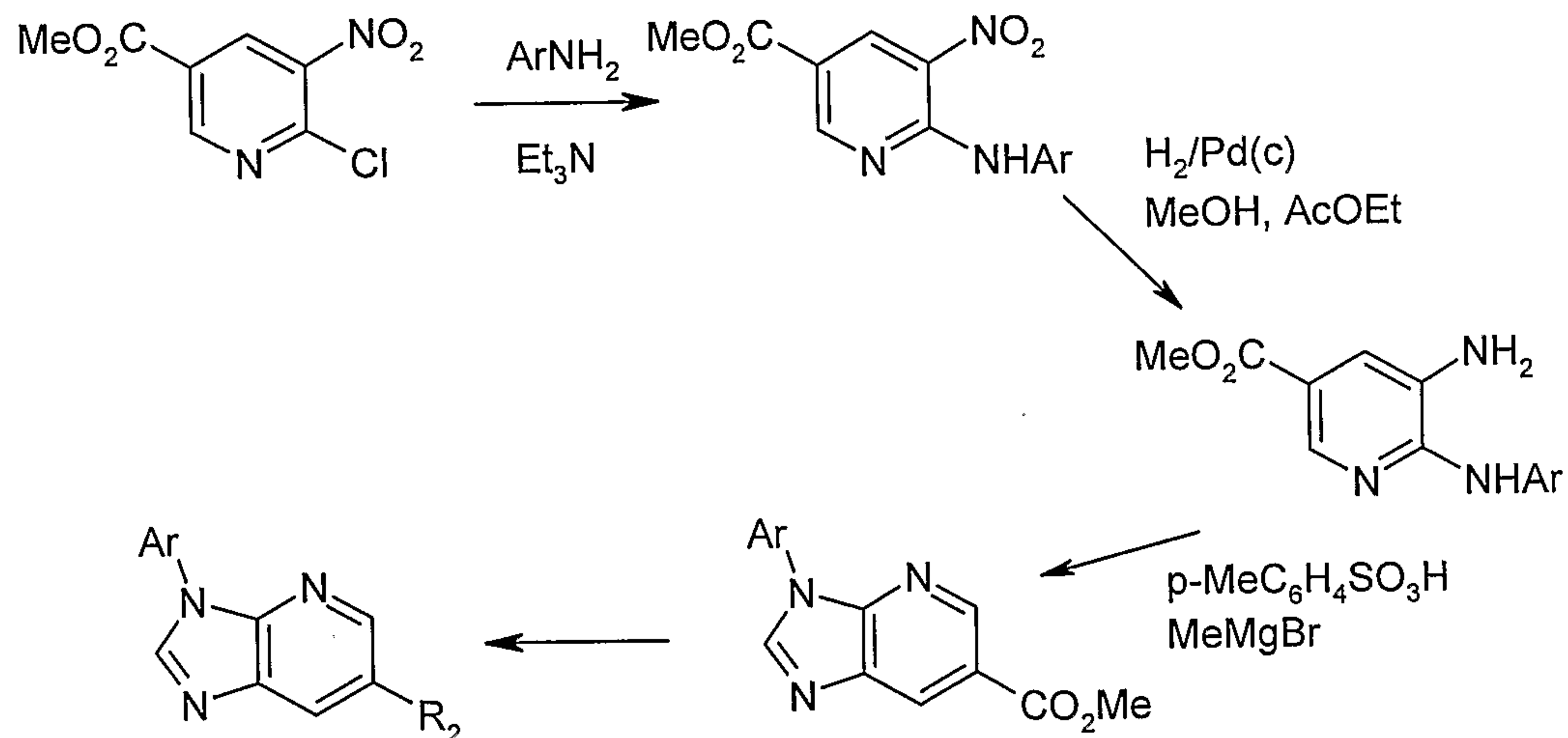
Scheme 9B
