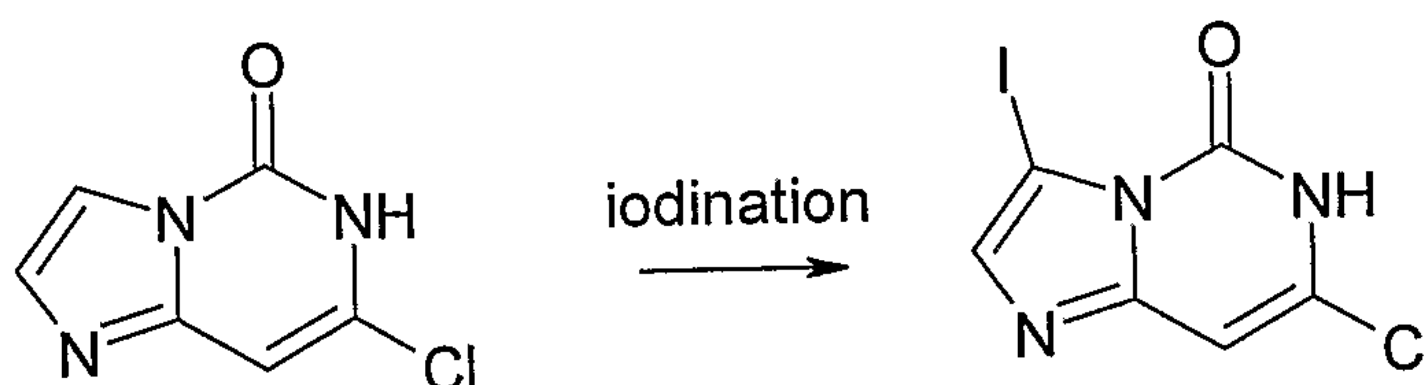
Scheme 18
