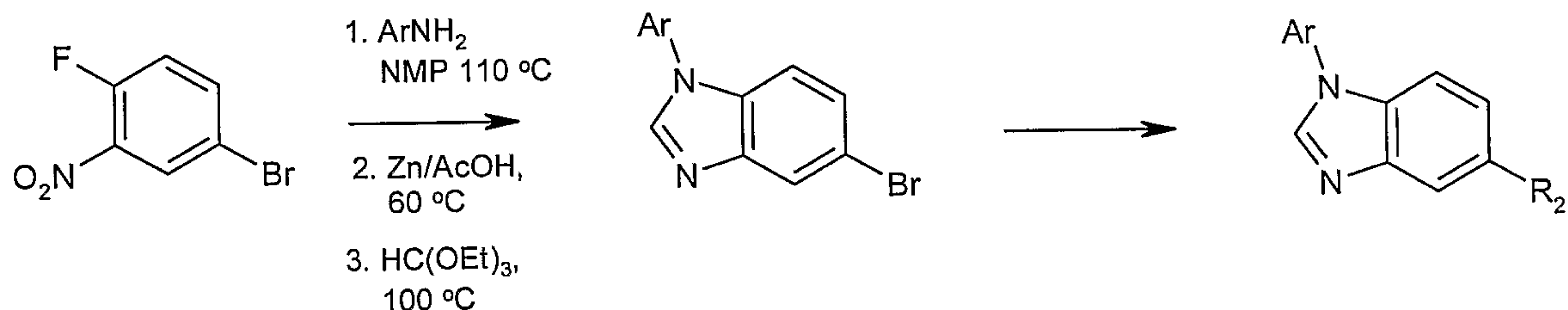
Scheme 13
