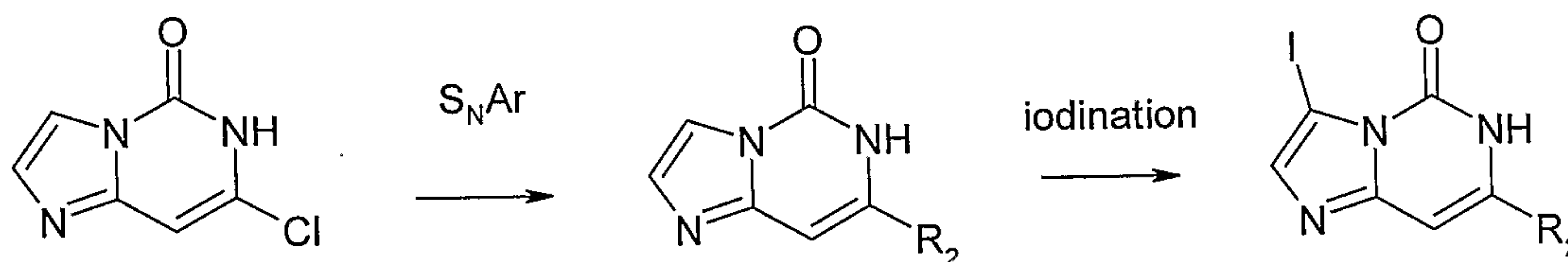
Scheme 17
