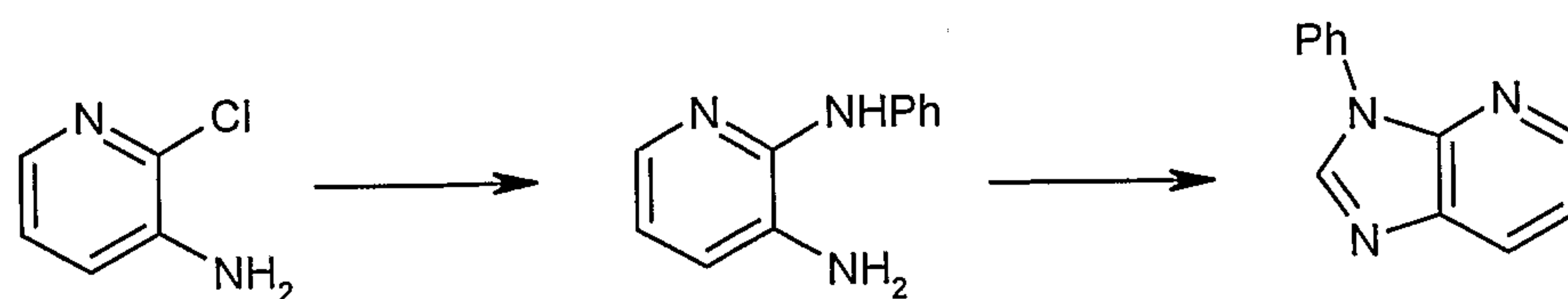
Scheme 8
