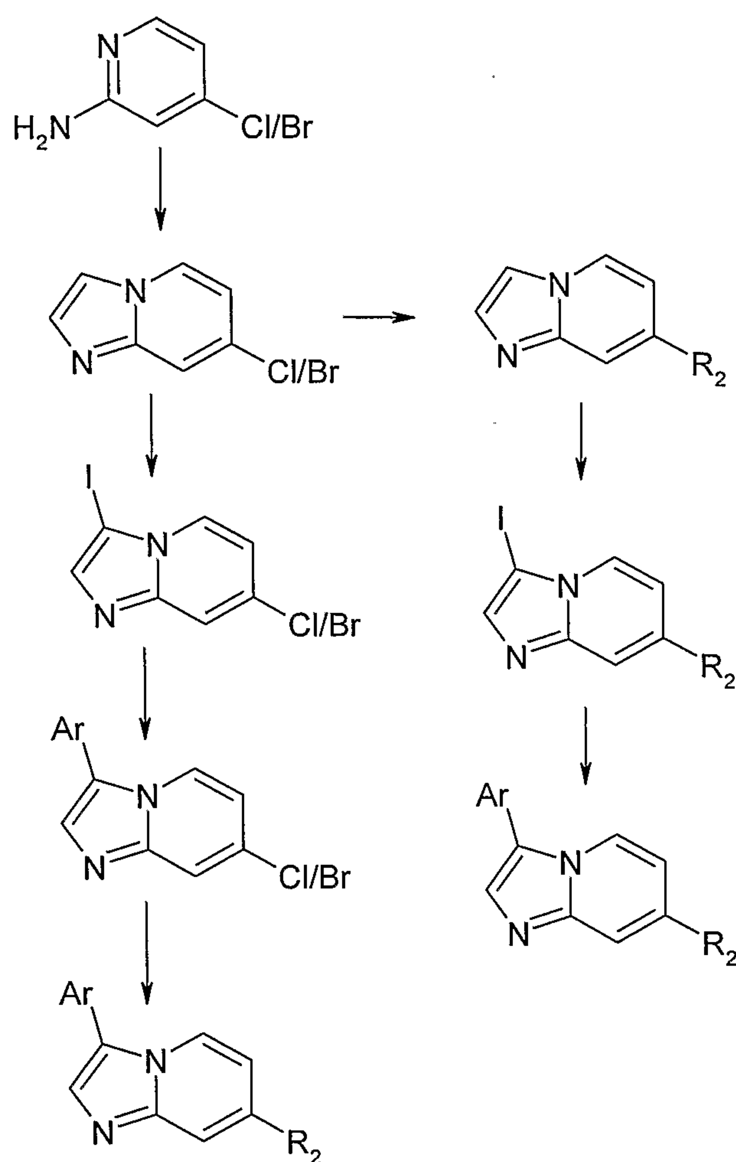
Scheme 2
