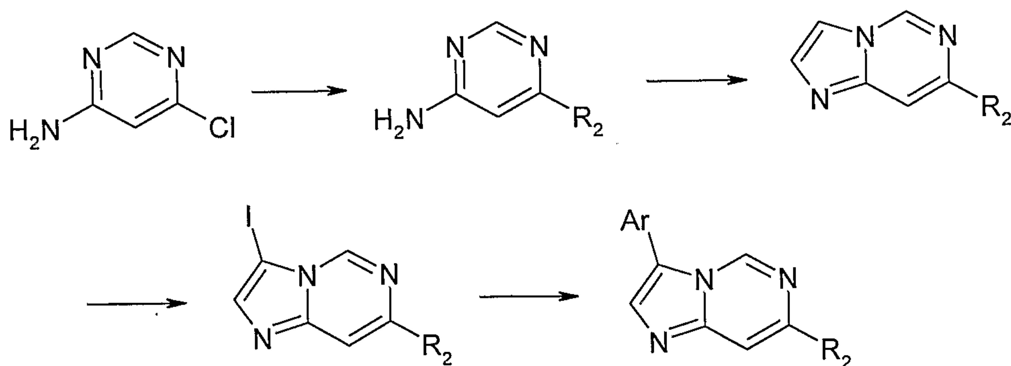
Scheme 16
