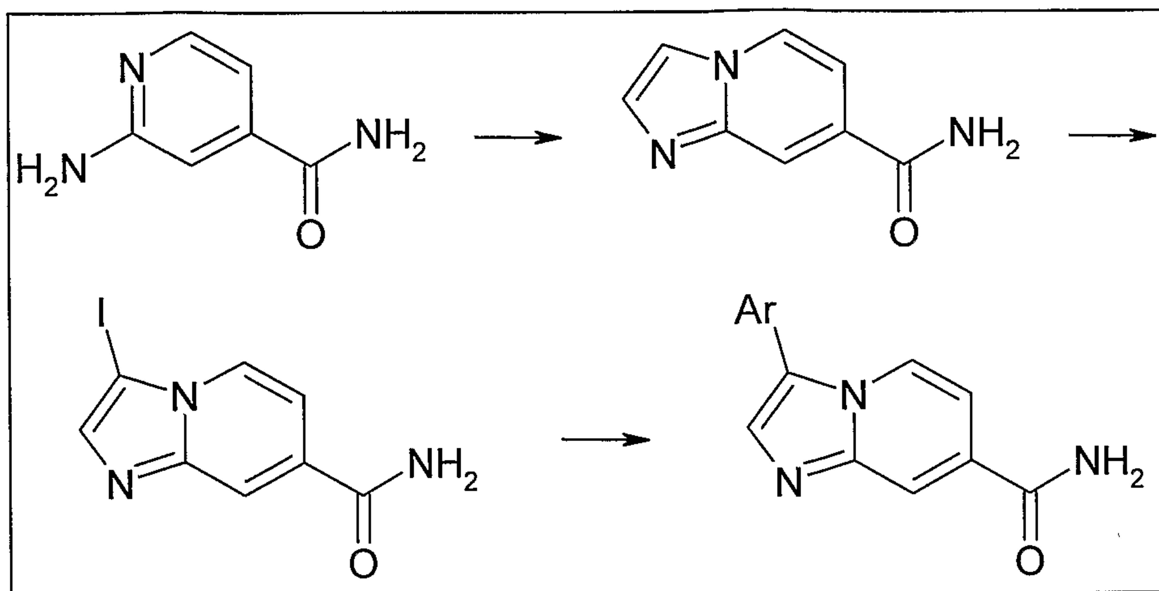
Scheme 1C
