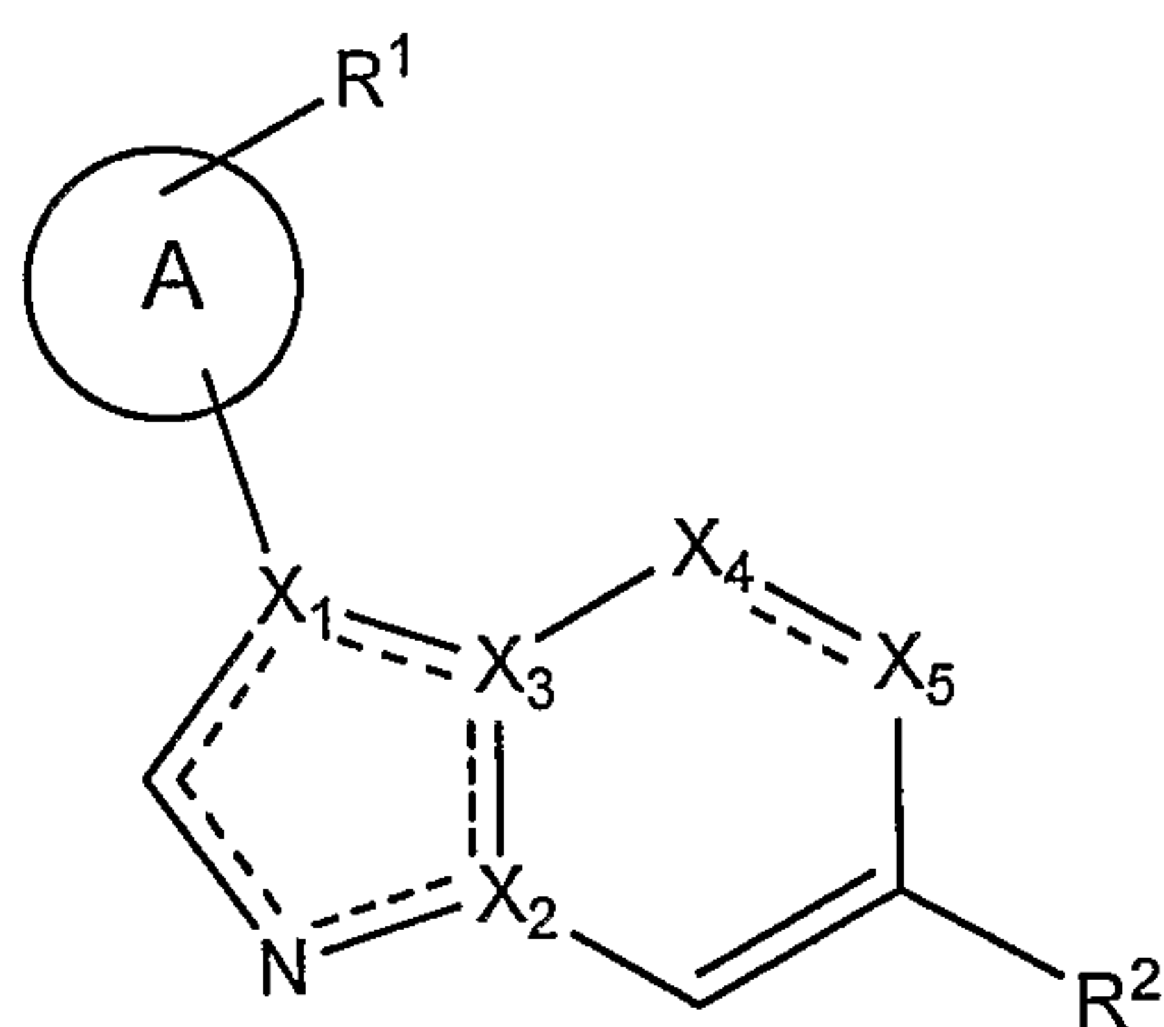
(lb)
