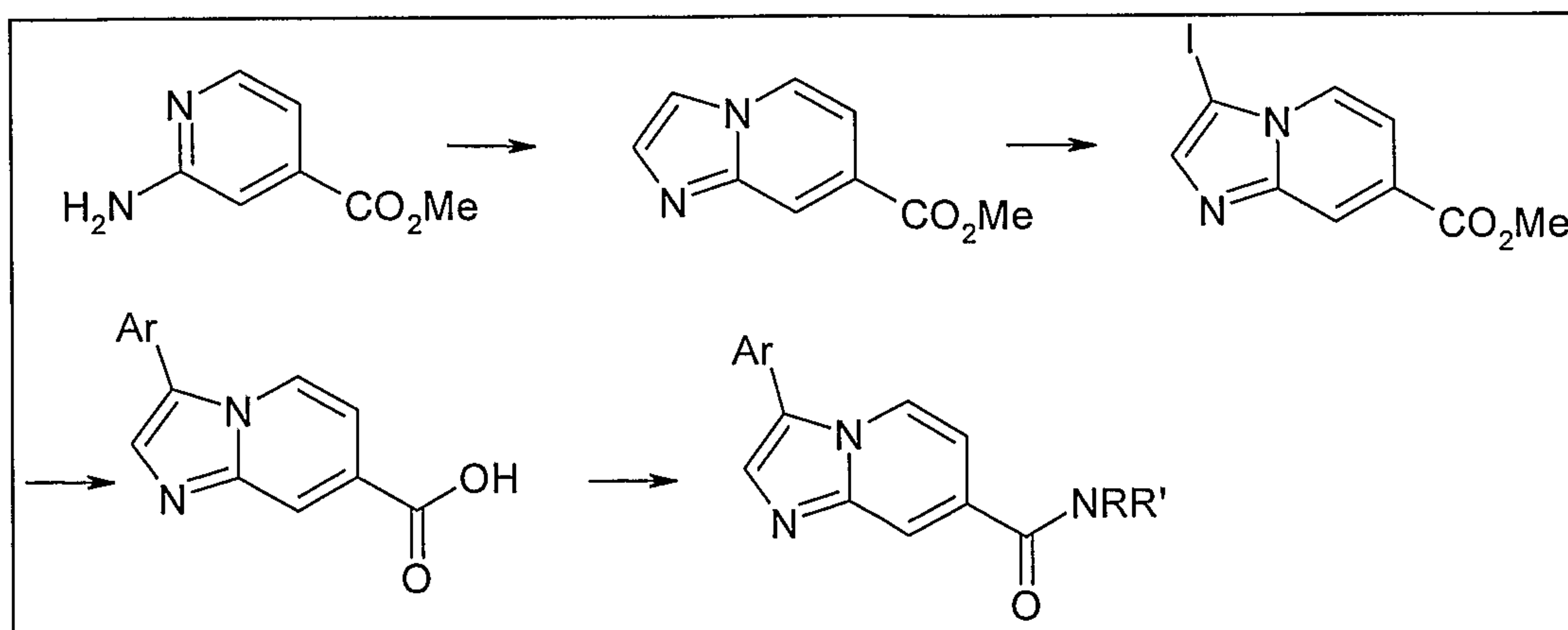
Scheme 1B
