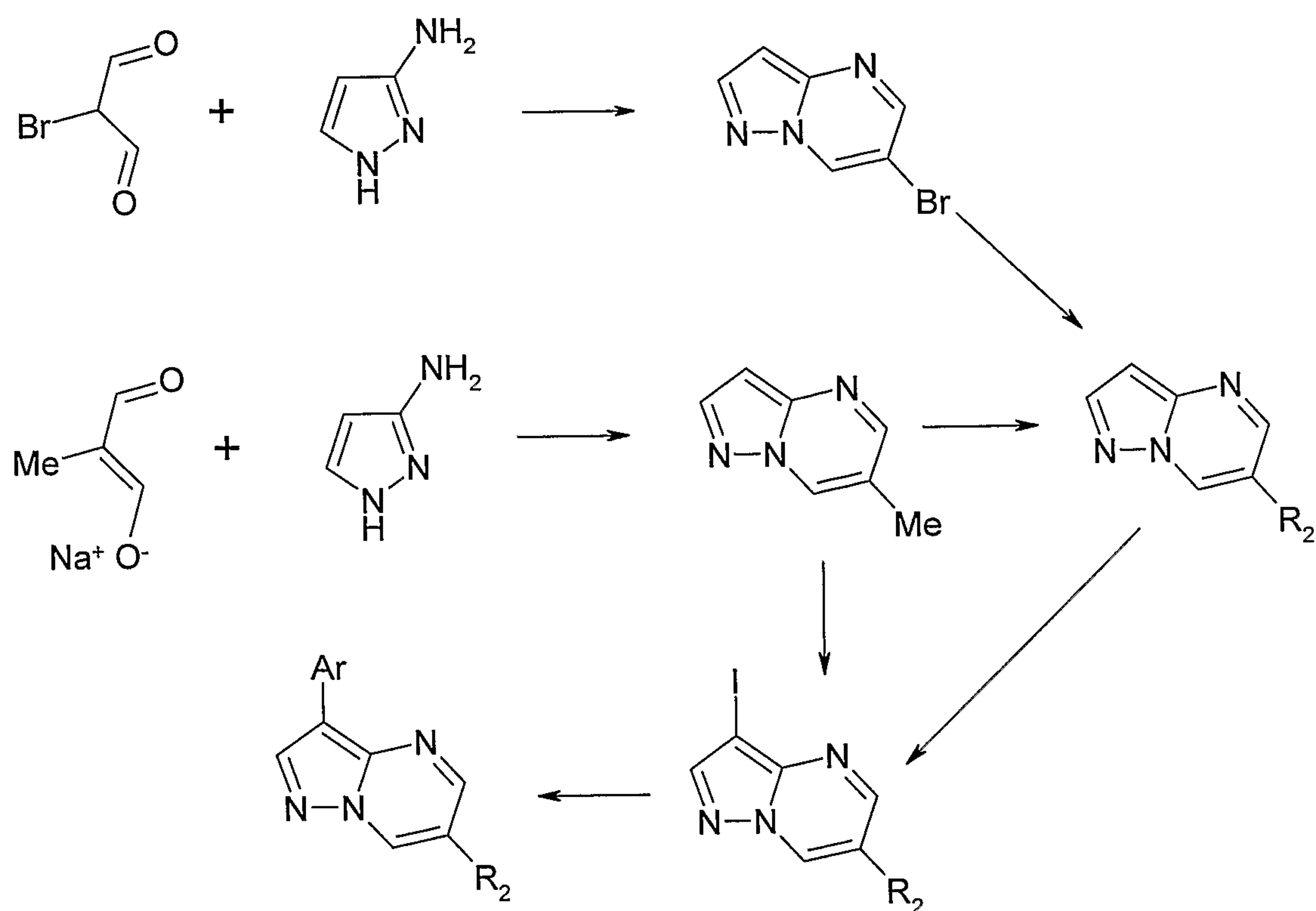
Scheme 5B
