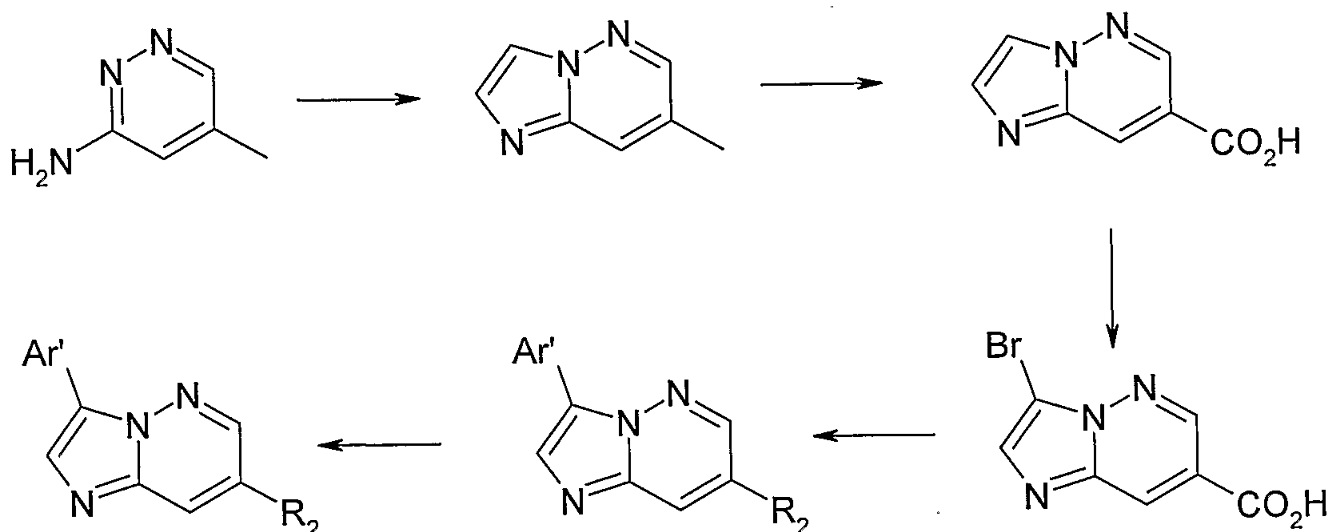
Scheme 19
