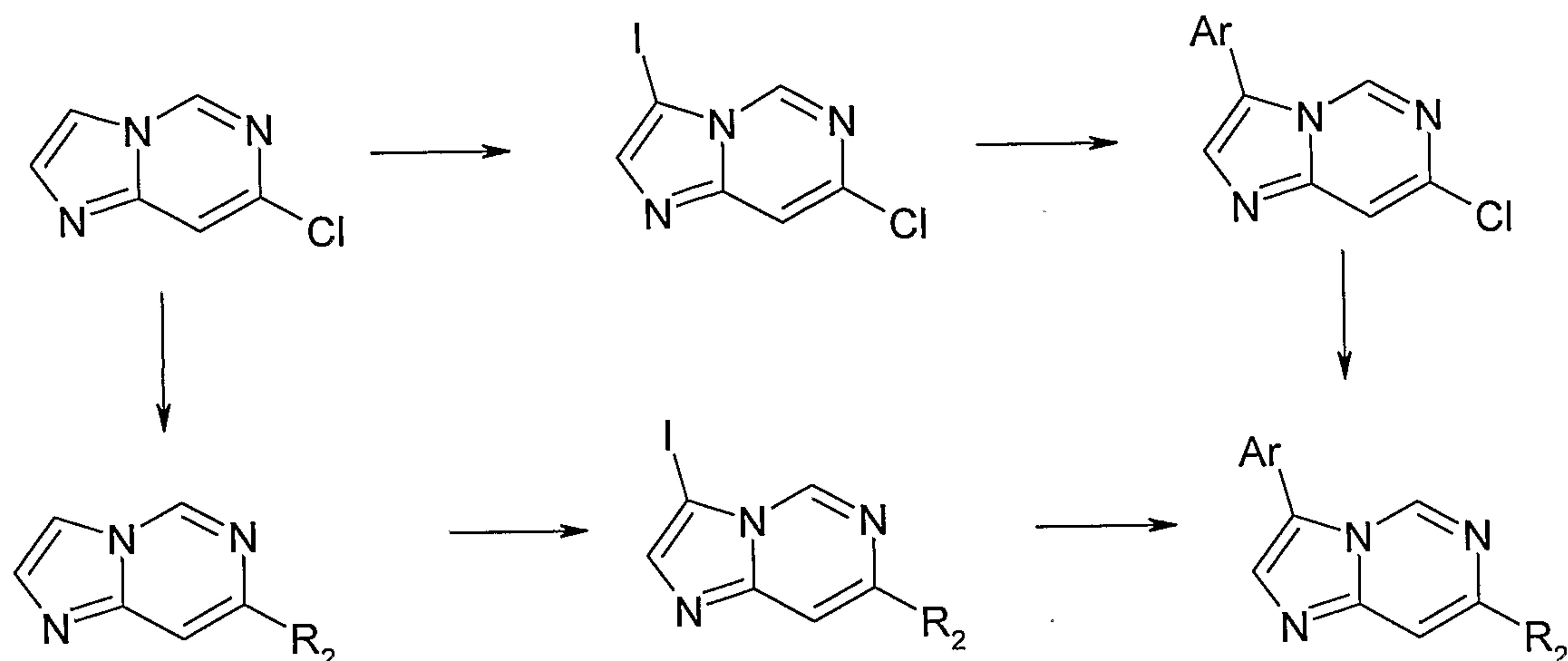
Scheme 14
