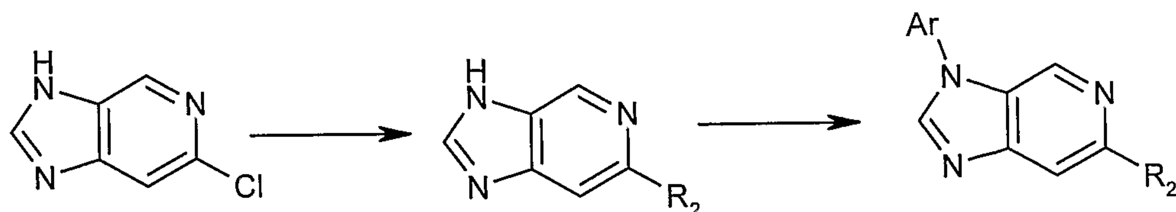
Scheme 12
