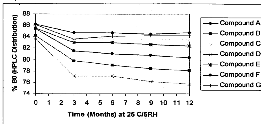
Fig. 1A. Dalbavancin Drug Product Stability Data (at 25 °C)
