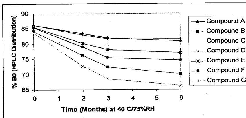
Fig. 2A. Dalbavancin Drug Product Stability Data (at 40 °C)
