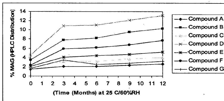
Fig. 1B. Dalbavancin Drug Product Stability Data (at 25 °C)
