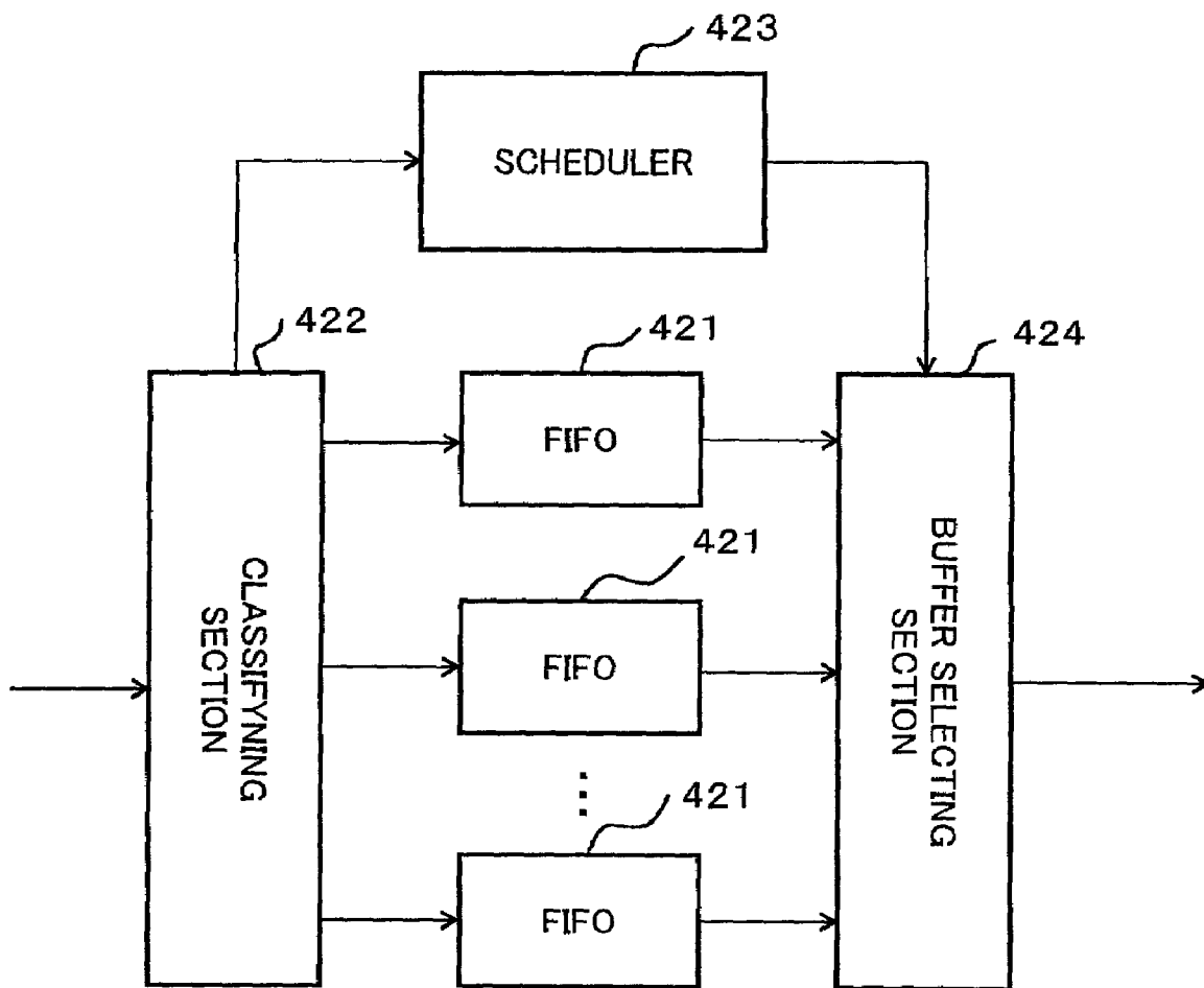
Fig.14 PRIOR ART
