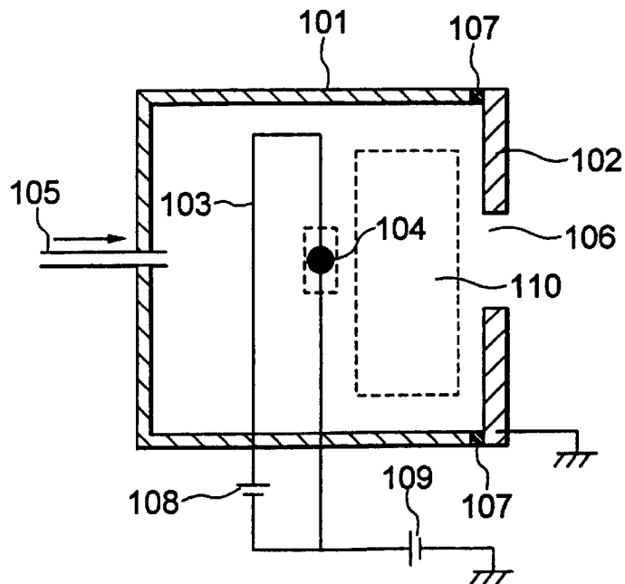
FIG. 10 RELATED ART
