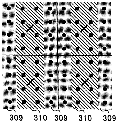
FIG. 4E DEMODULATION OF S4 IS POSSIBLE
