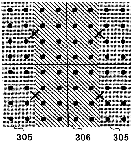
FIG. 4C DEMODULATION OF S2 IS POSSIBLE
