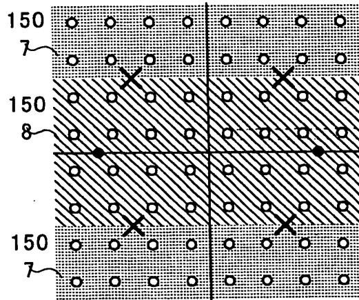
FIG. 16B DEMODULATION OF S1 IS IMPOSSIBLE
