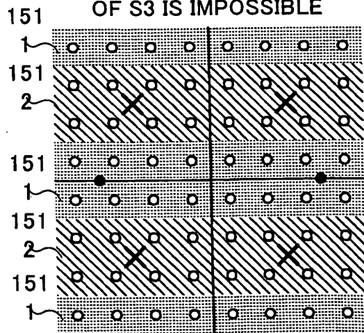
FIG. 16F DEMODULATION OF S5 IS IMPOSSIBLE
