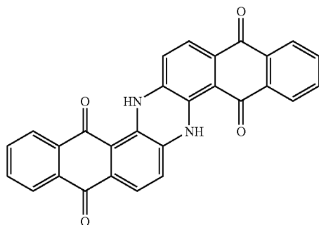
6,15-Dihydro-dinaphtho[2,3-a;2',3'-h]phenazine-5,9,14,18-tetraone
