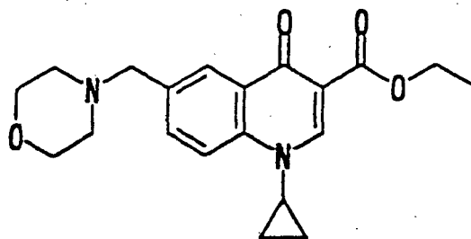
Compound [H]
