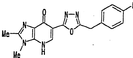
Compound [B]
