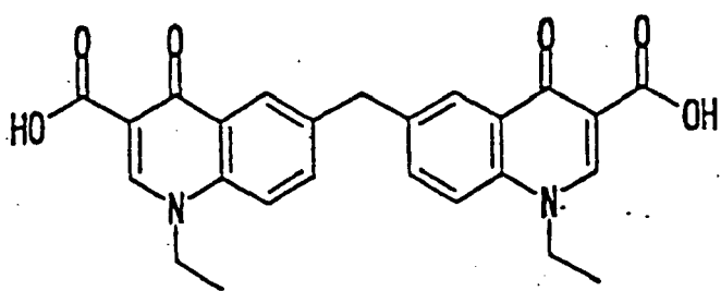
Compound [F]
