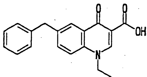
Compound [E]
