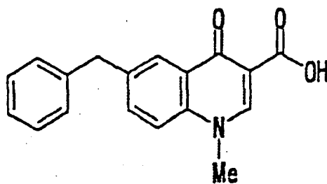
Compound [G]
