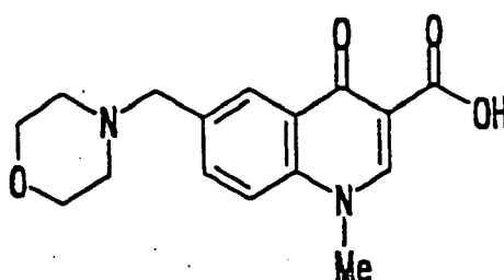
Compound [J]
