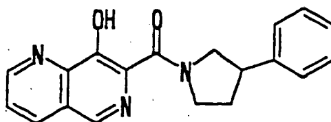
Compound [D]
