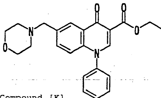
Compound [K]
