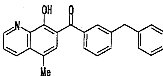
Compound [C]
