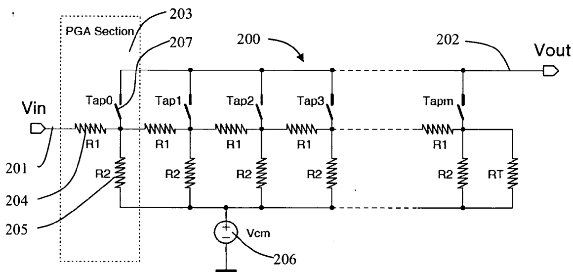
CONVENTIONAL ART FIG. 2
