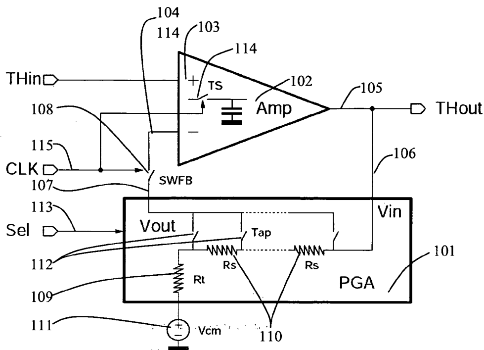
CONVENTIONAL ART FIG. 1
