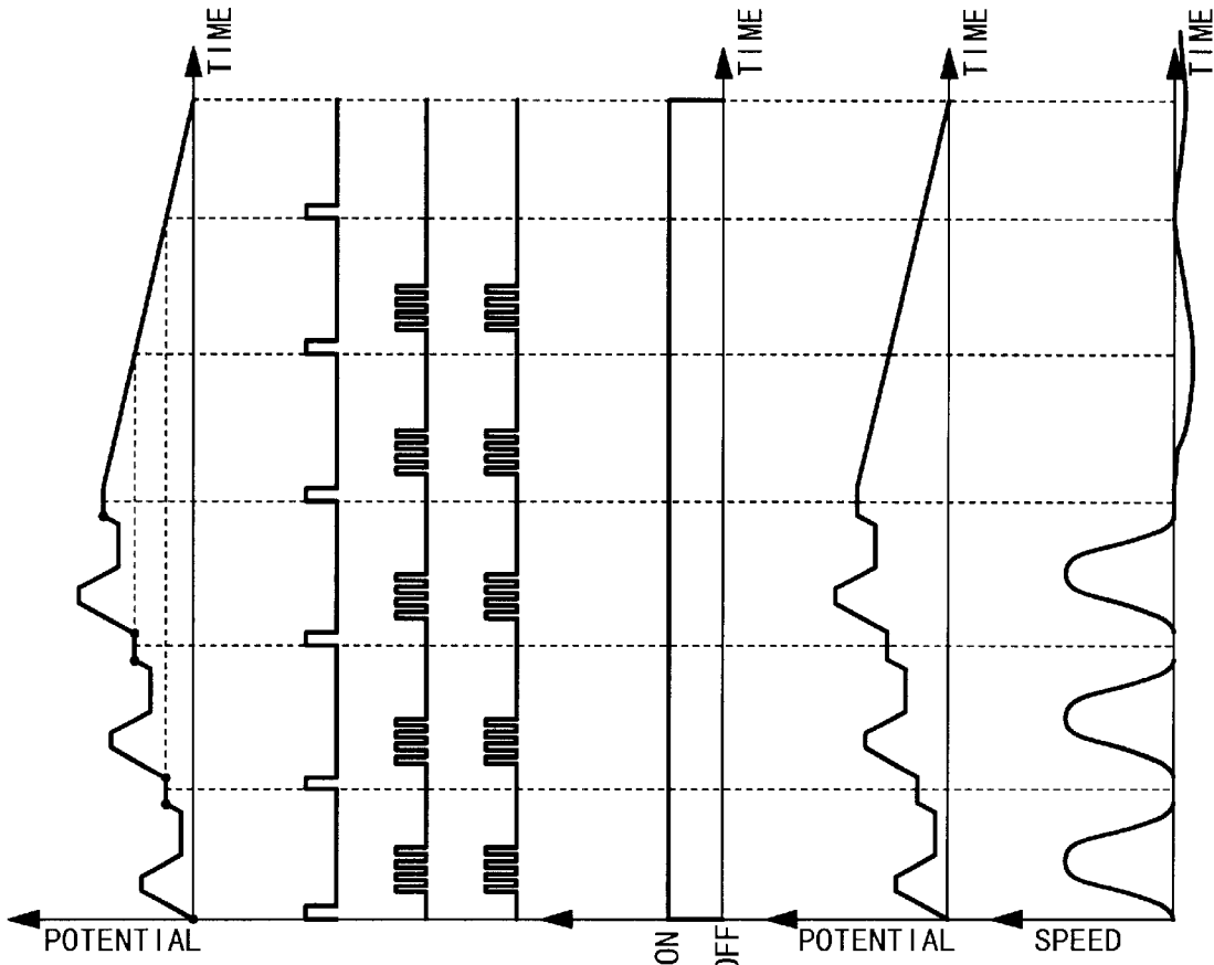
Fig. 12E WAVEFORM EXTRACTION TIMING
