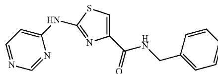
N-Benzyl-2-(pyrimidin-4-ylamino)thiazole-4-carboxamide
