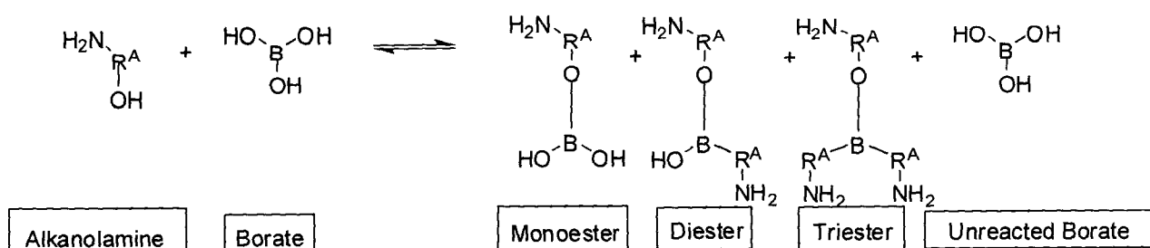
Scheme 1 – Formation of an alkanolamine/borate complex from boric acid
