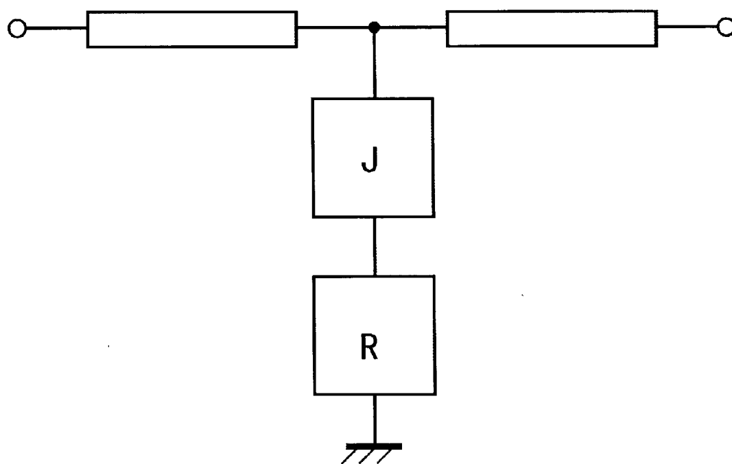
LSM 01 TRANSMISSION SYSTEM
