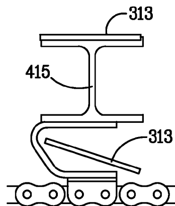
Section F-F FIG. 14
