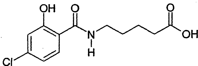
compound 1
