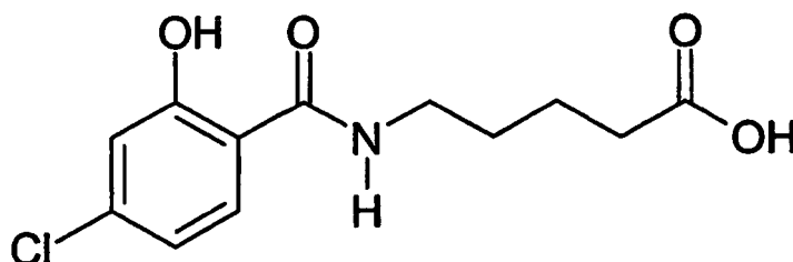
Compound 1
