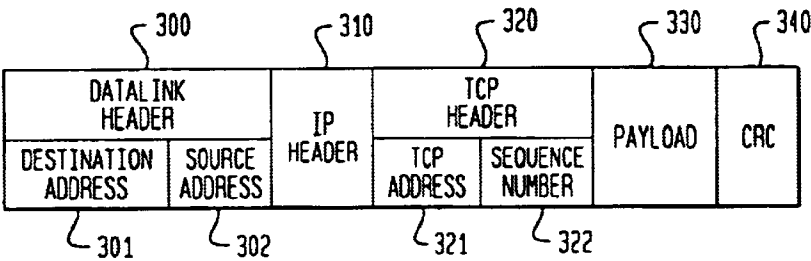
FIG. 4 (PRIOR ART)
