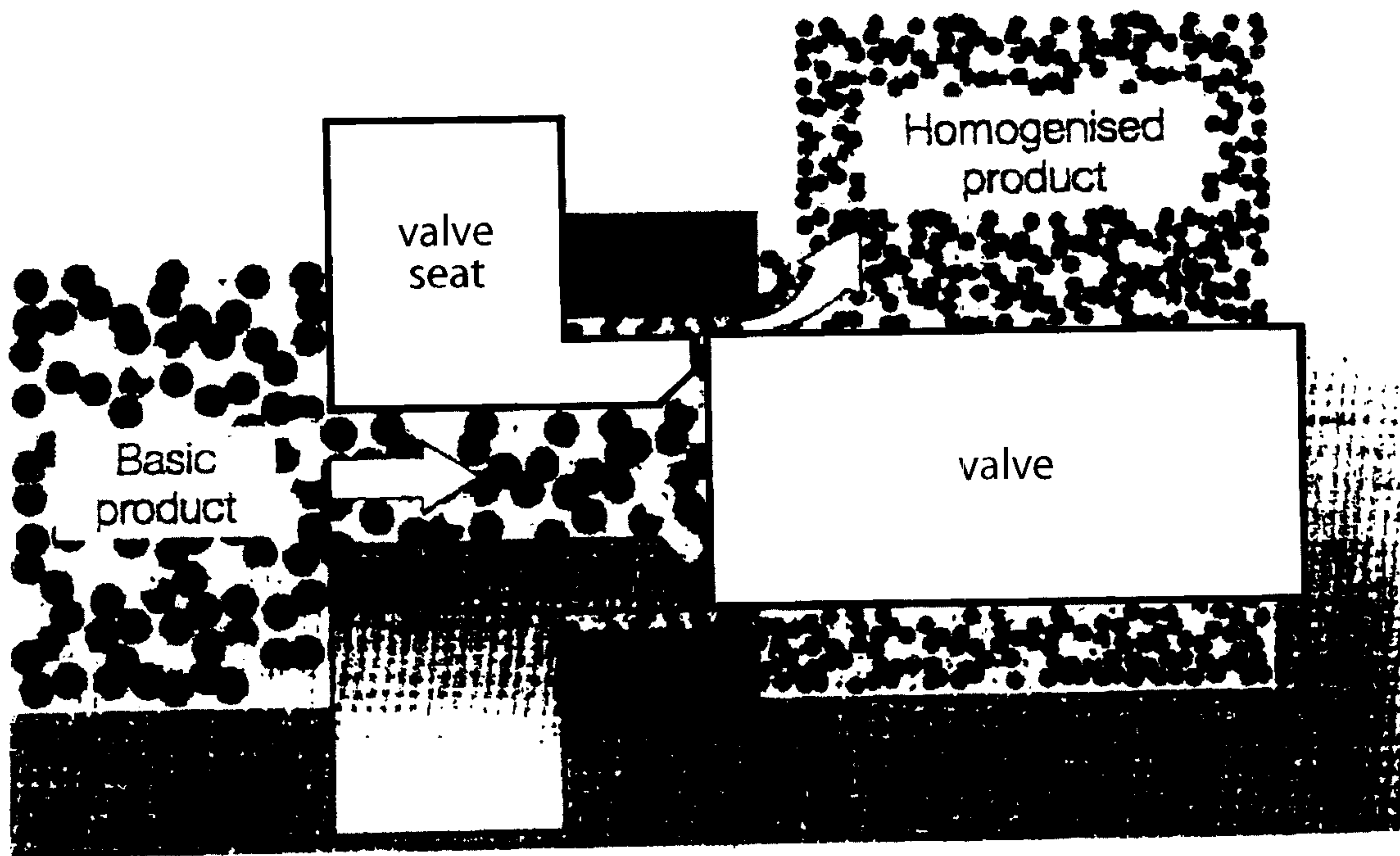
Fig. 1. Mode of functioning of the homogenizing valve.
