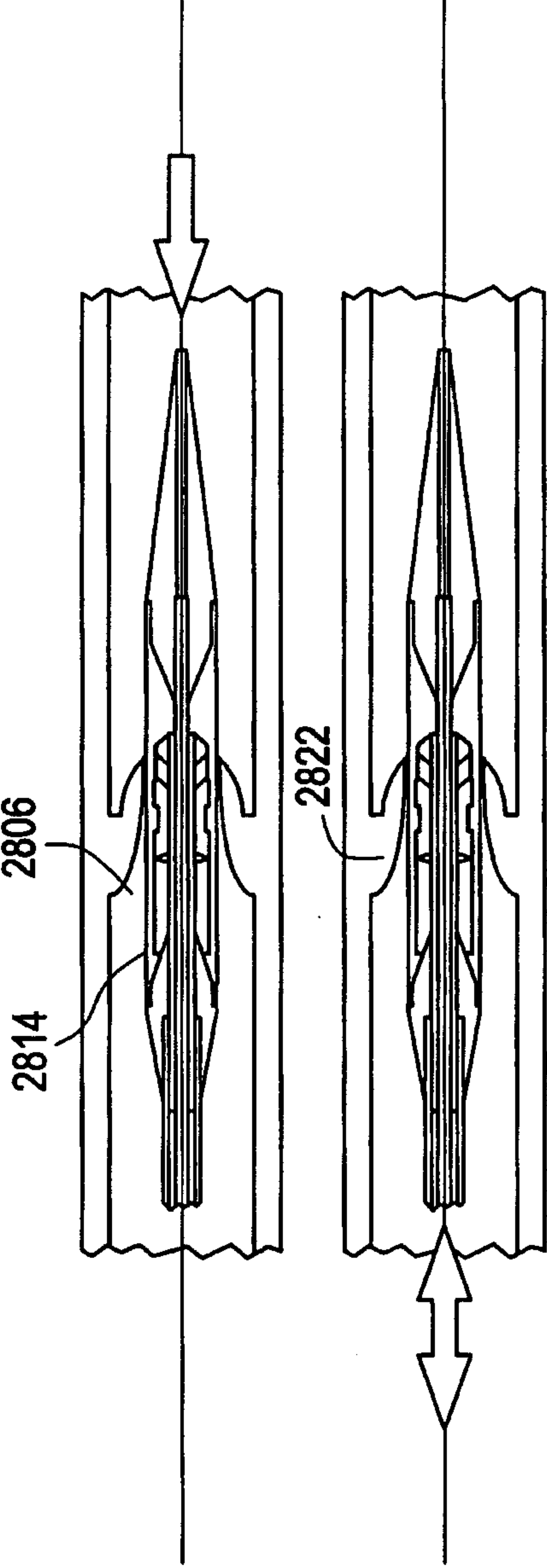
FIG. 28B Stent Recapturing/ Repositioning
