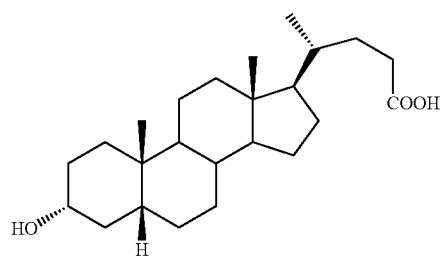
Lithocholic acid
