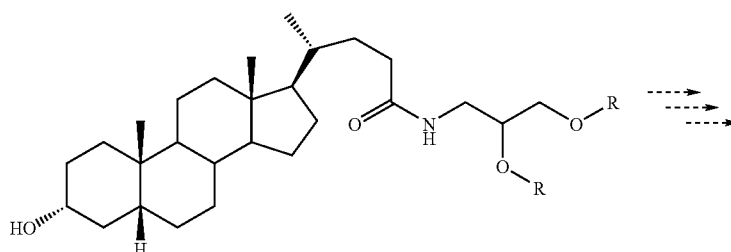
Lithocholic acid
