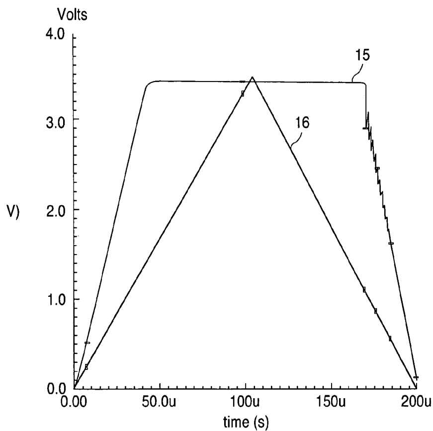
FIG. 2 (PRIOR ART)
