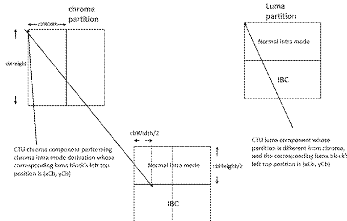
When fetch the mode of intraPredModeY[xCb + cbWidth / 2][yCb + cbHeight / 2] , it corresponds to an IBC block, where no luma intra mode is defined/available
