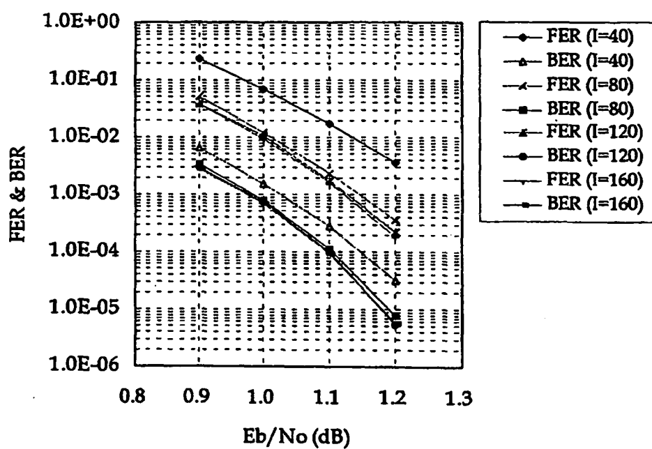
FER & BER performance ( n=7.7K , R=1/2 )
