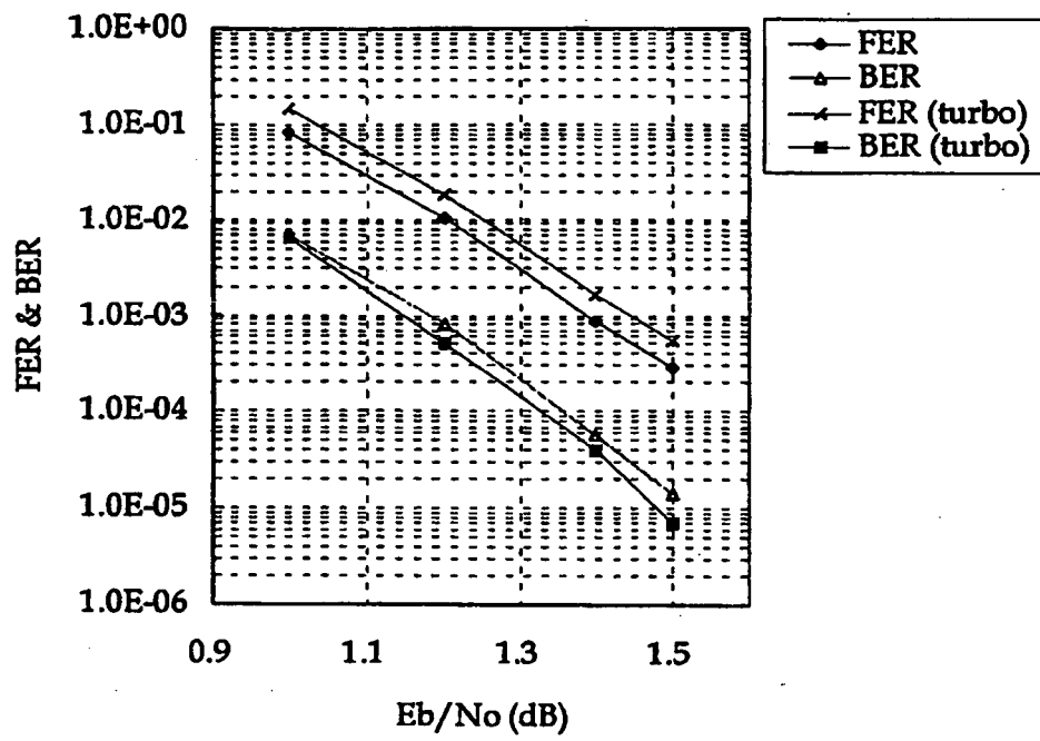
FER & BER performance ( n=3.1K , R=1/2 )
