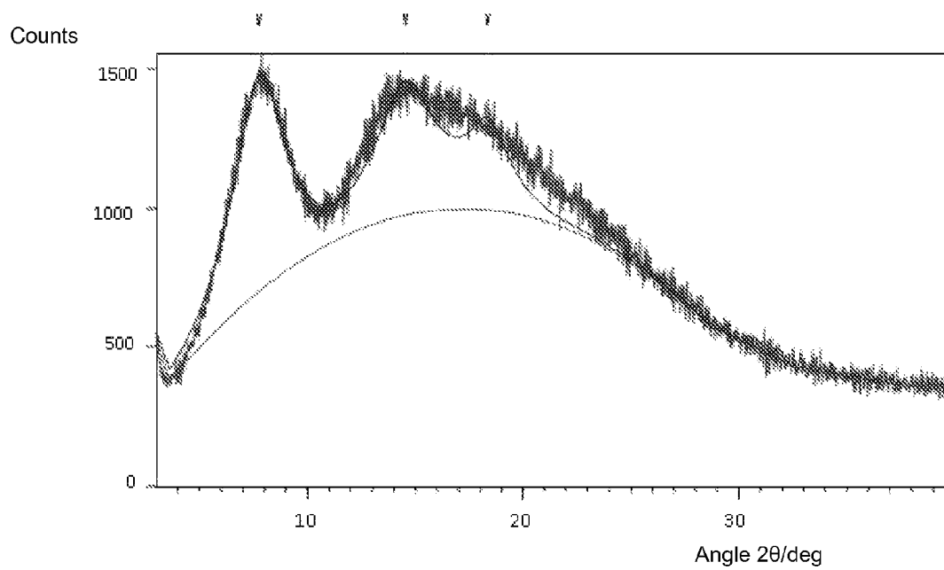
Figure 3: X-Ray diffraction spectra obtained by spray drying process .
