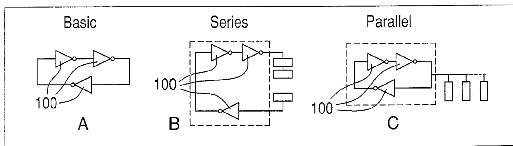
Basic Ring Oscillator and Resulting Resonant Systems
