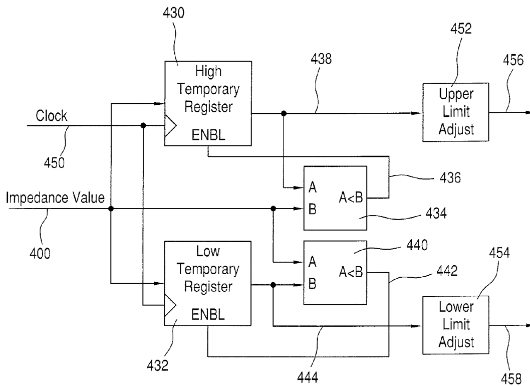
Determination of Threshold Limits Dynamically
