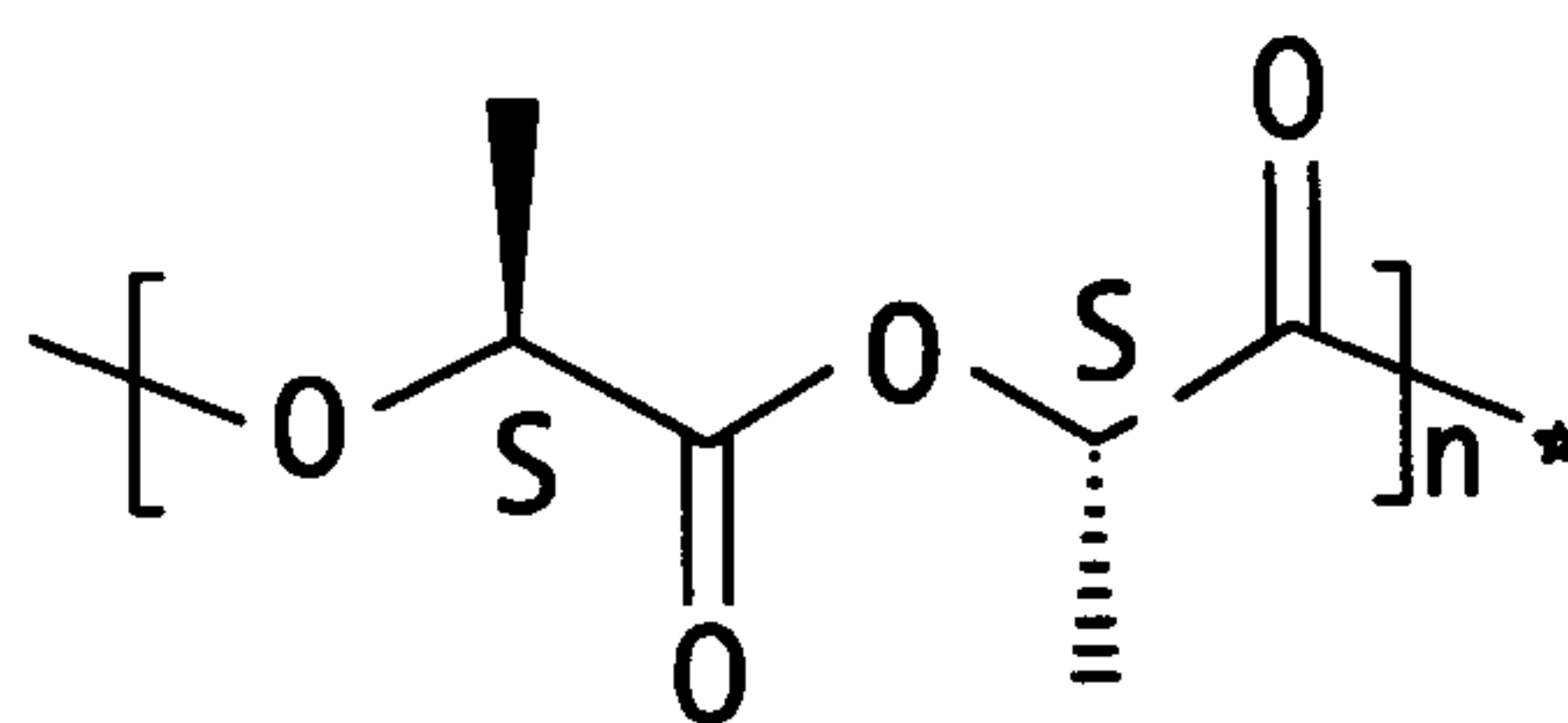
poly (L-lactide)
