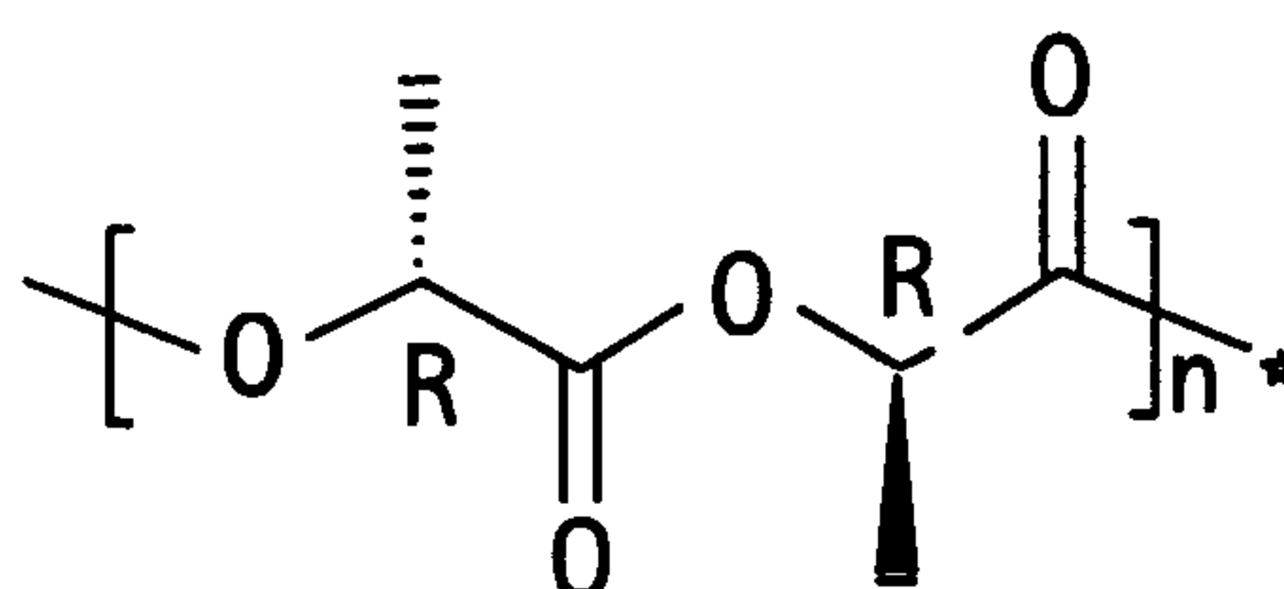
poly (D-lactide)
