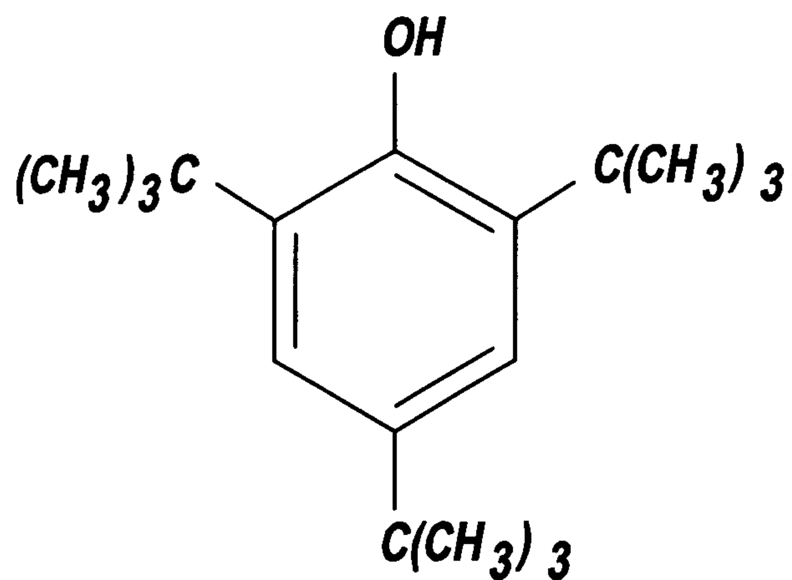
Butylated hydroxytoluene
