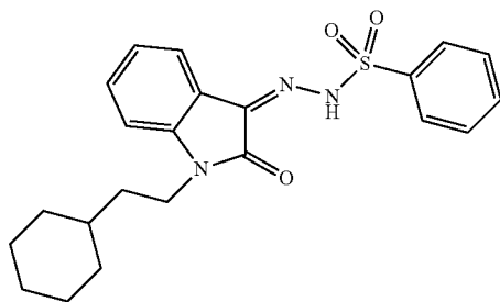
N'-[1-(2-cyclohexylethyl)-2-oxo-1,2-dihydro-3H-indol-3-ylidene]benzenesulfonohydrazide
