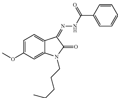
A) 1-pentyl-6-methoxy-isatin
