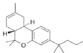
JWH133
