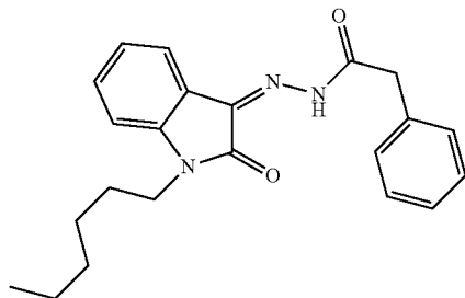
A) Phenyl-acetic acid [1-hexyl-2-oxo-1,2-dihydro-indol-3-ylidene]-hydrazide
