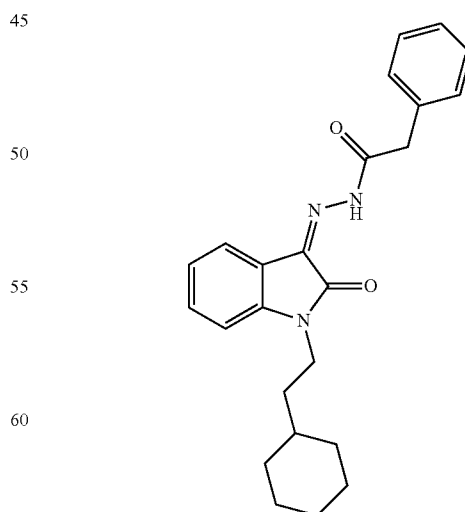
N'-[1-(2-cyclohexylethyl)-2-oxo-1,2-dihydro-3H-indol-3-ylidene]benzenesulfonohydrazide
