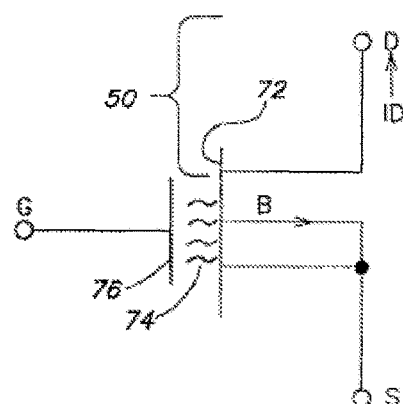
FIG. 2 (Prior Art)
