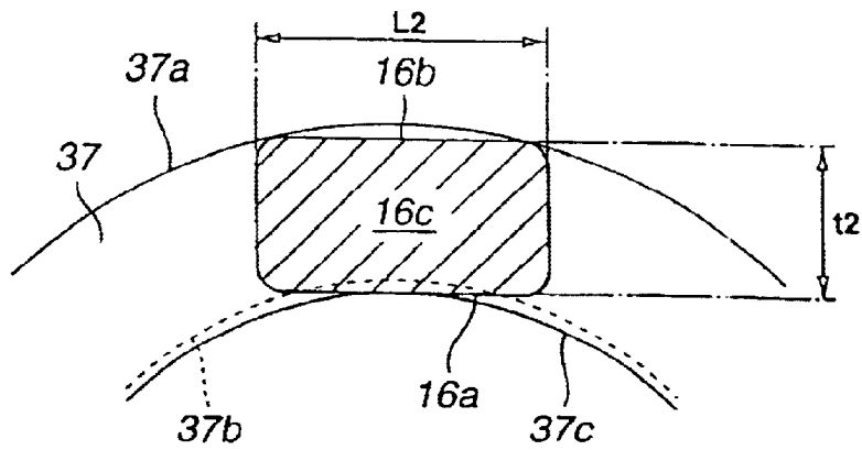
FIG.11C PRIOR ART
