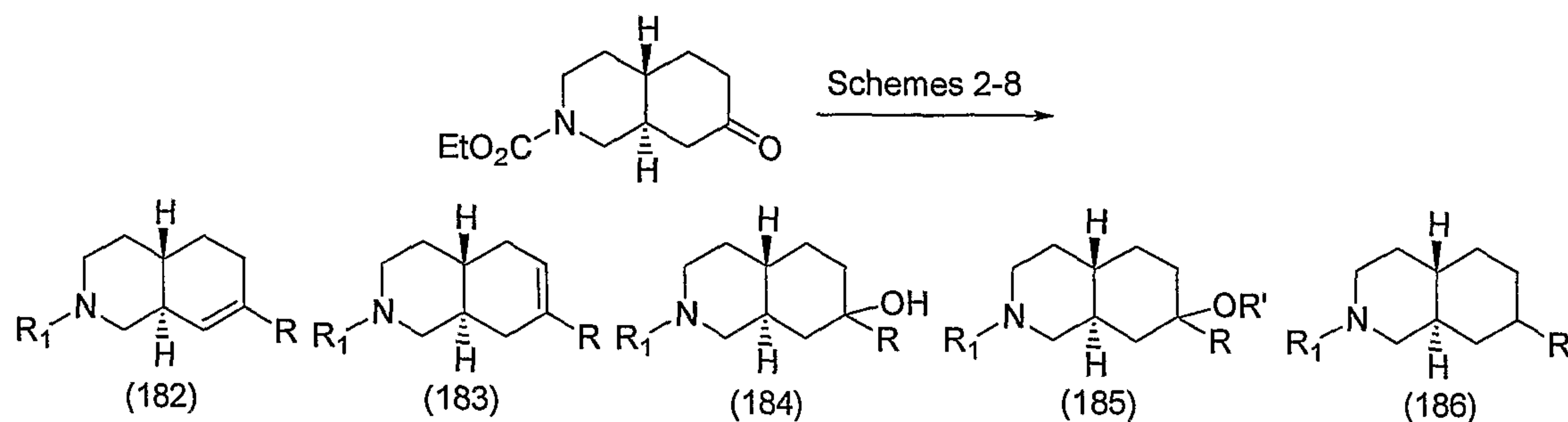
Scheme 38
