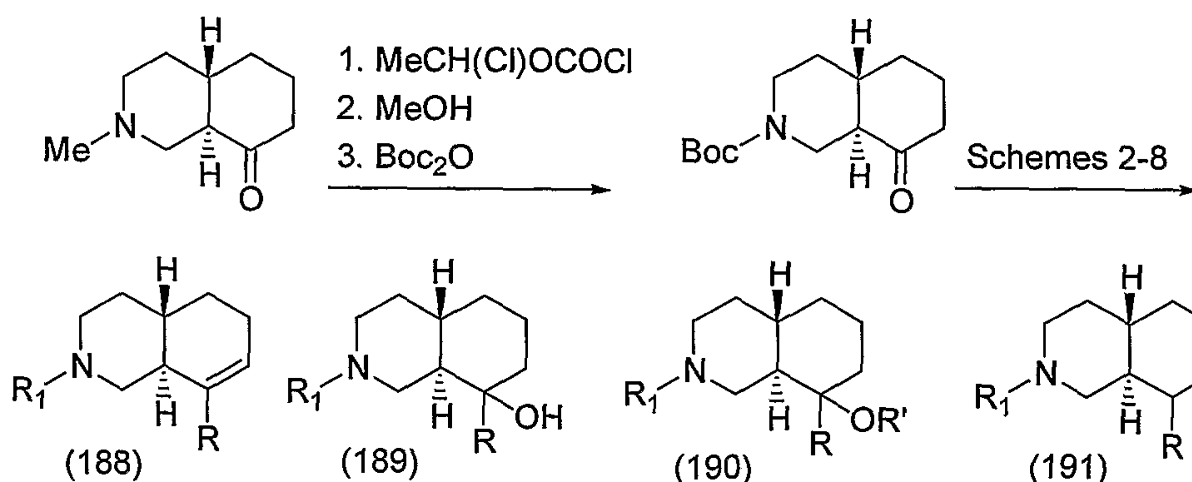
Scheme 39
