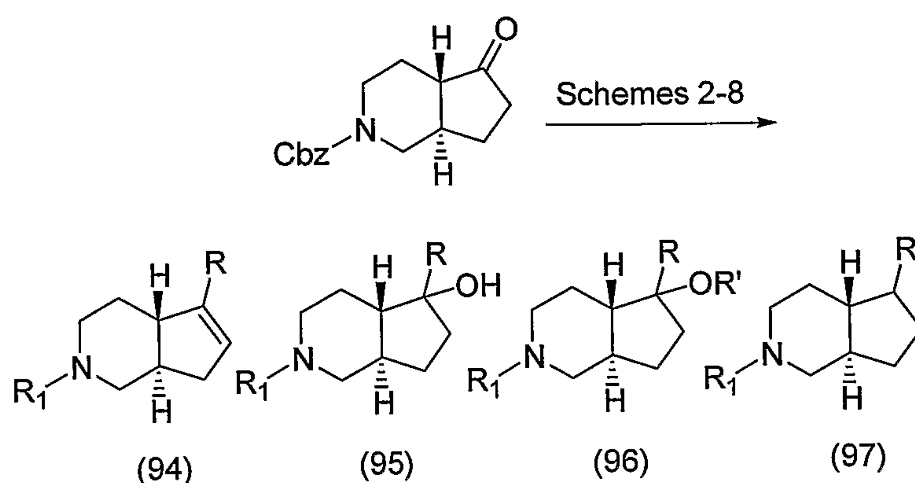
Scheme 23
