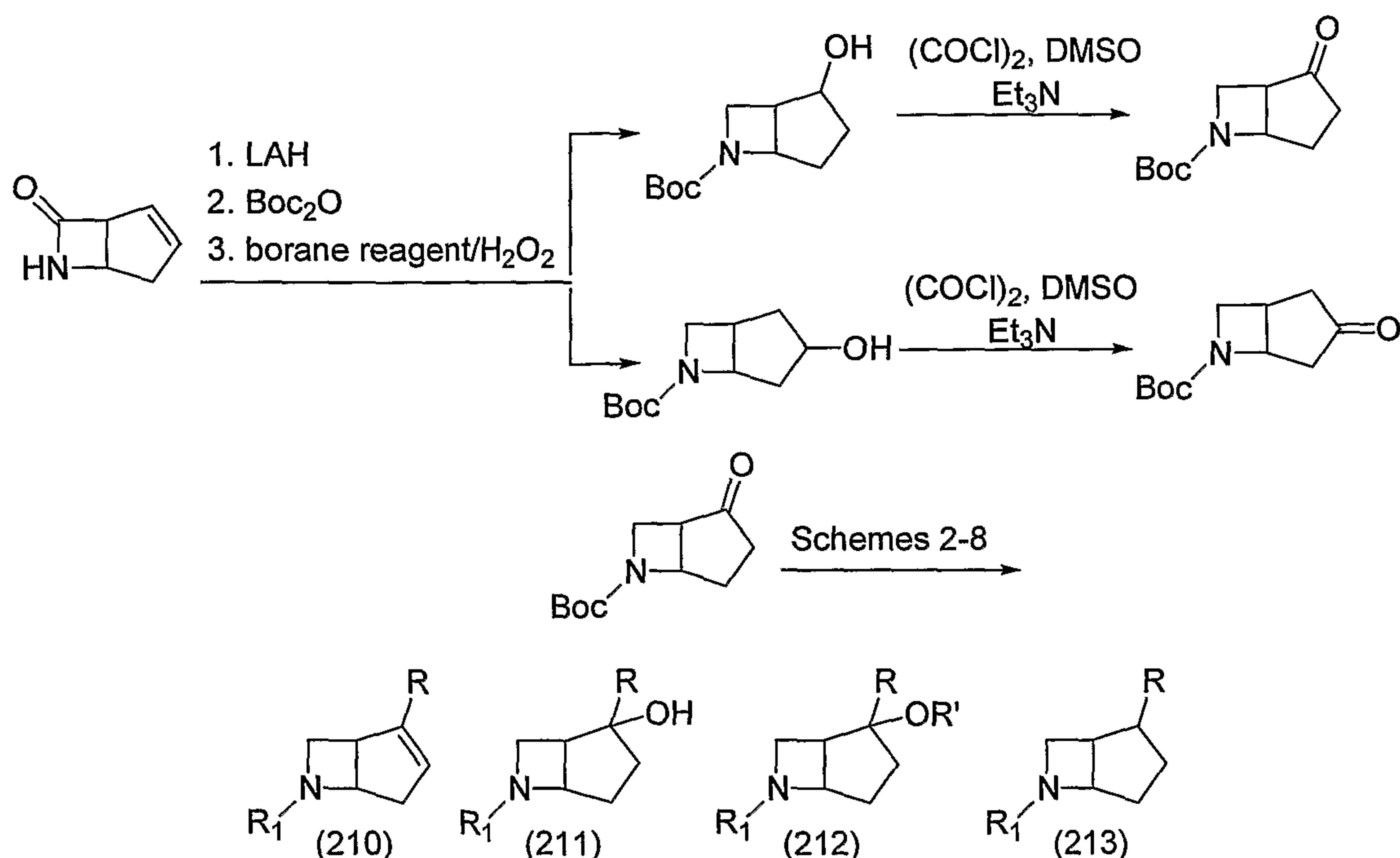
Scheme 44
