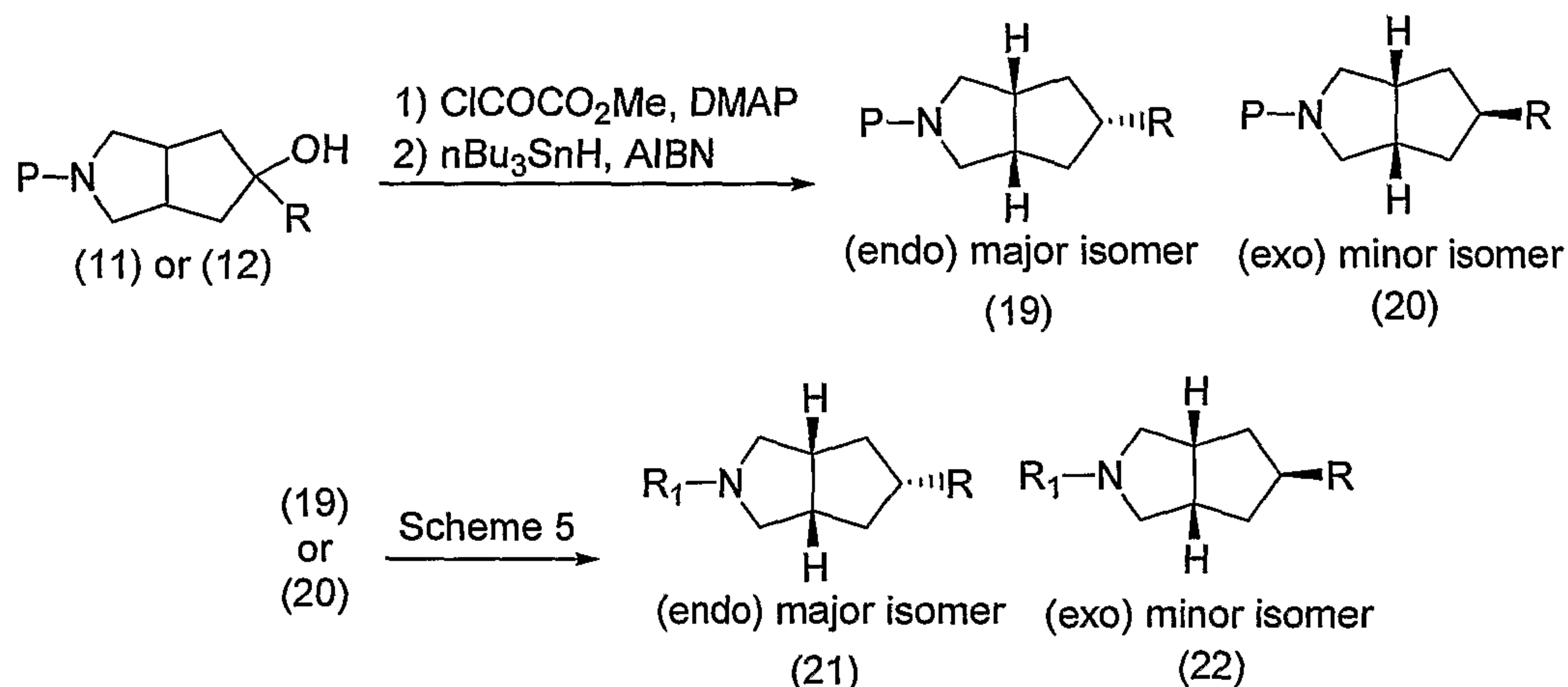
Scheme 7
