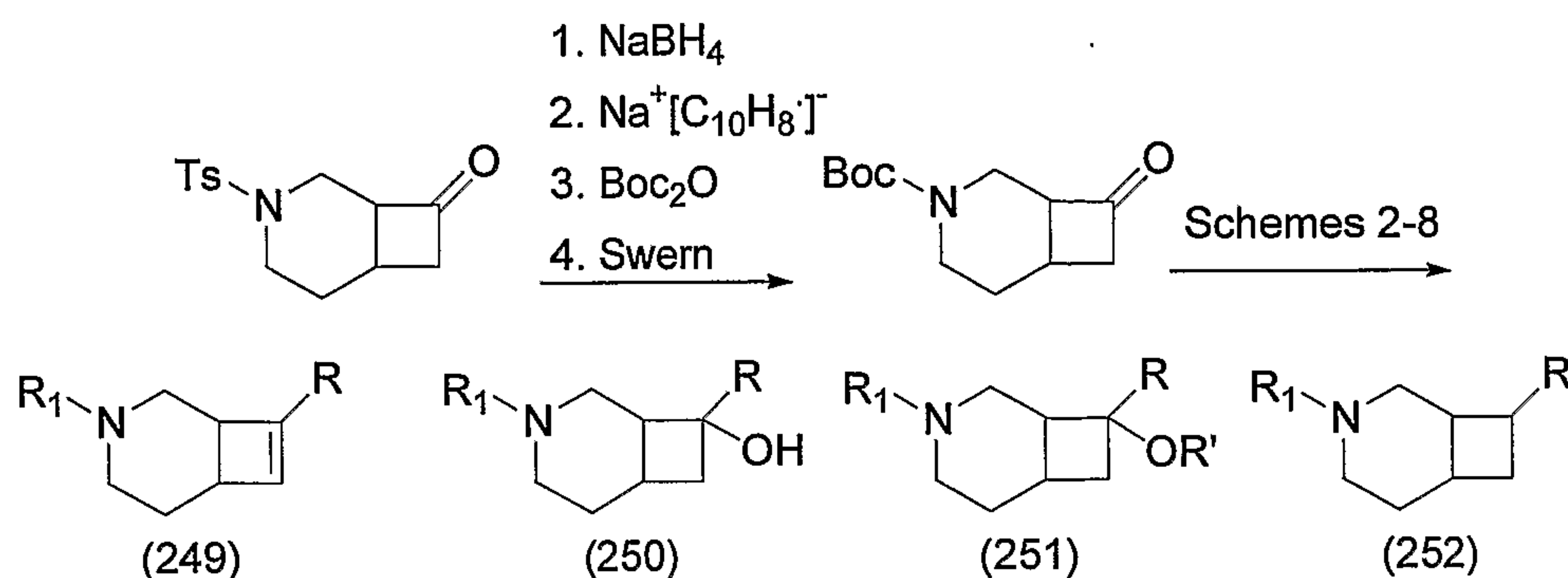
Scheme 50
