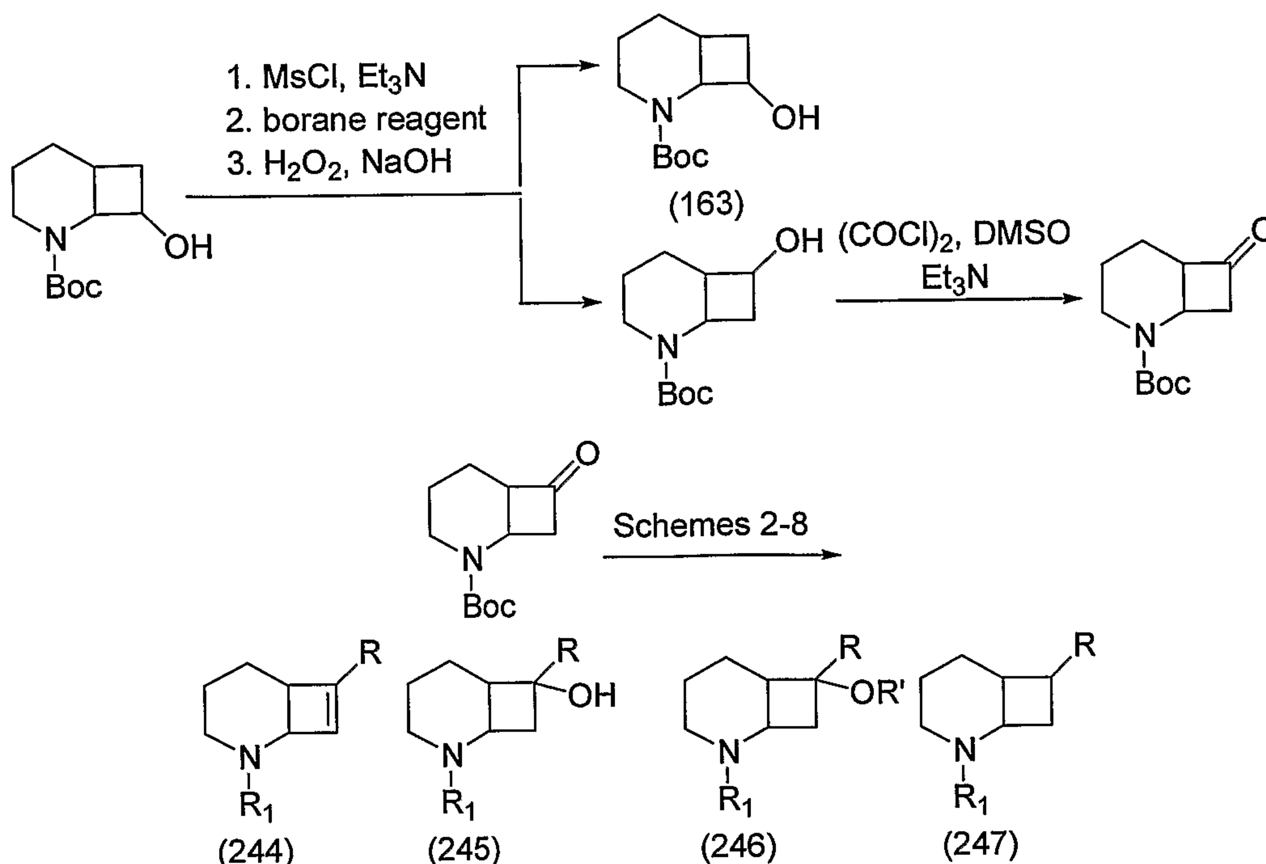
Scheme 49
