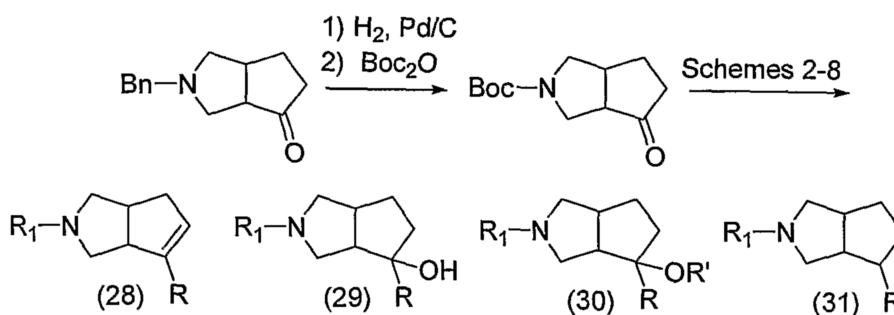
Scheme 9
