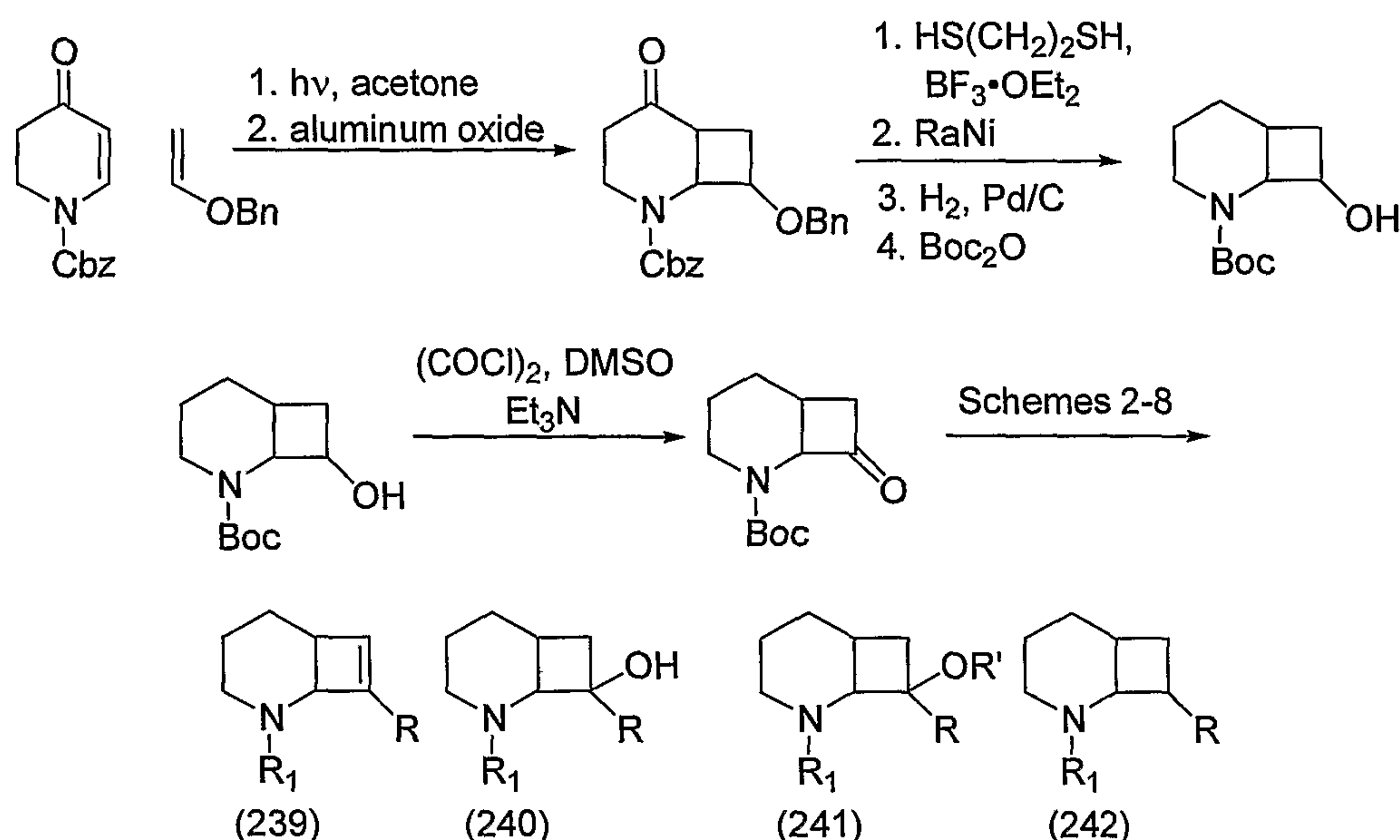
Scheme 48
