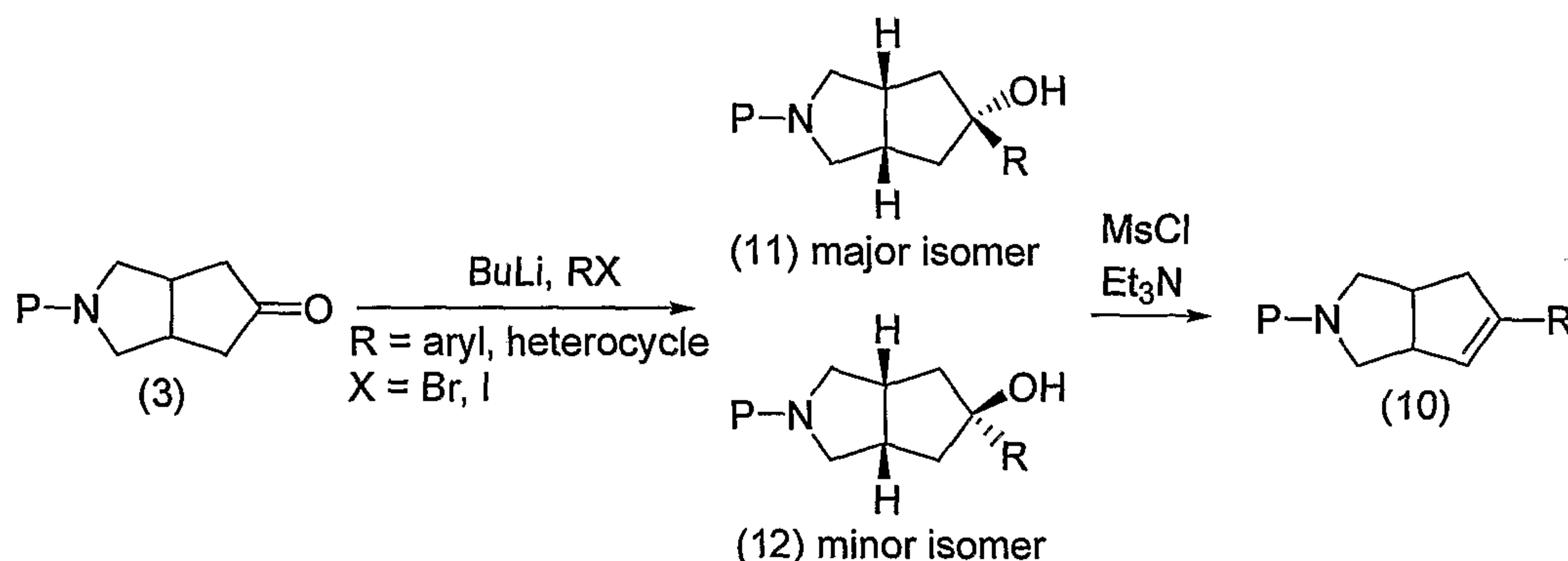
Scheme 4
