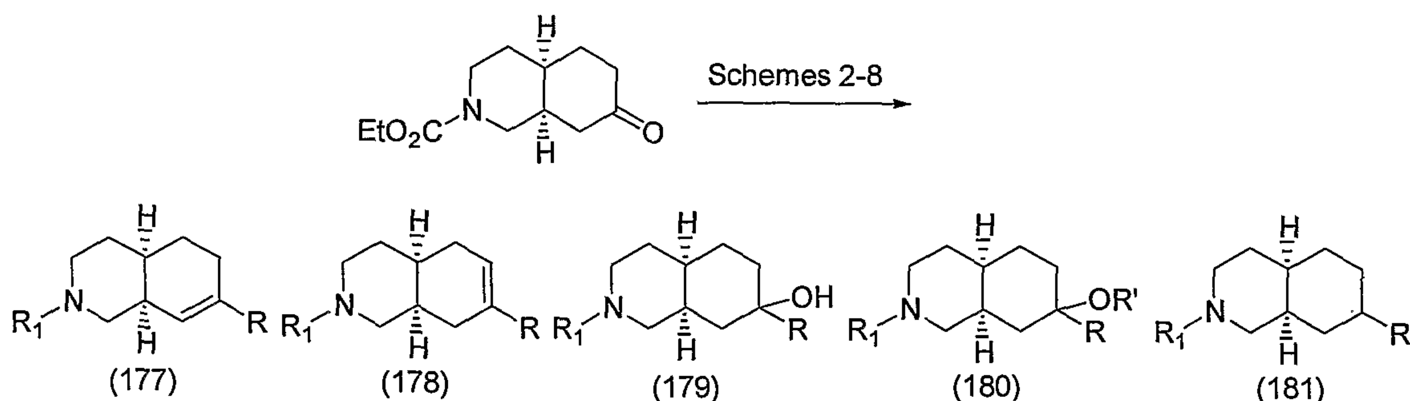
Scheme 37
