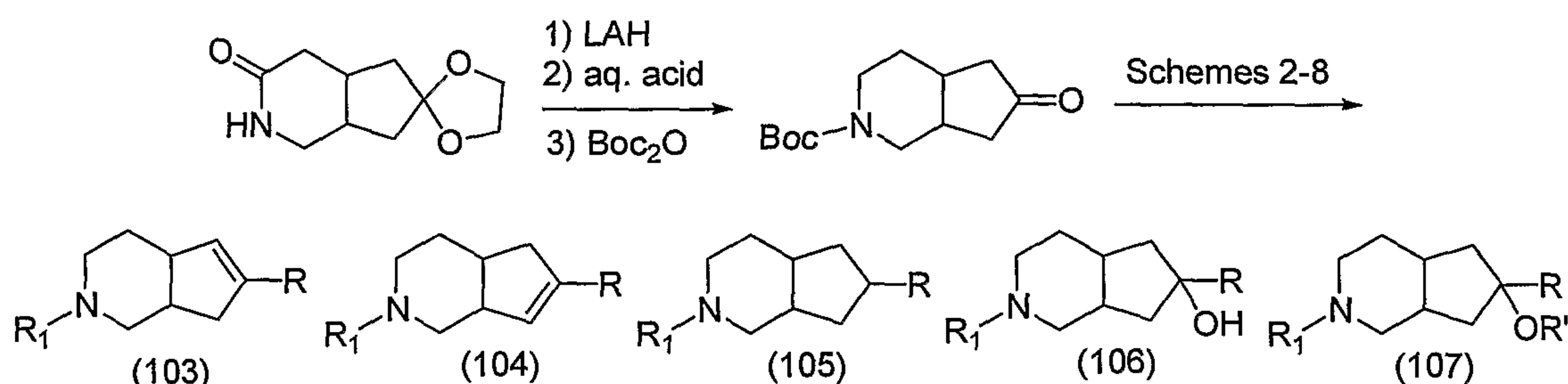
Scheme 25
