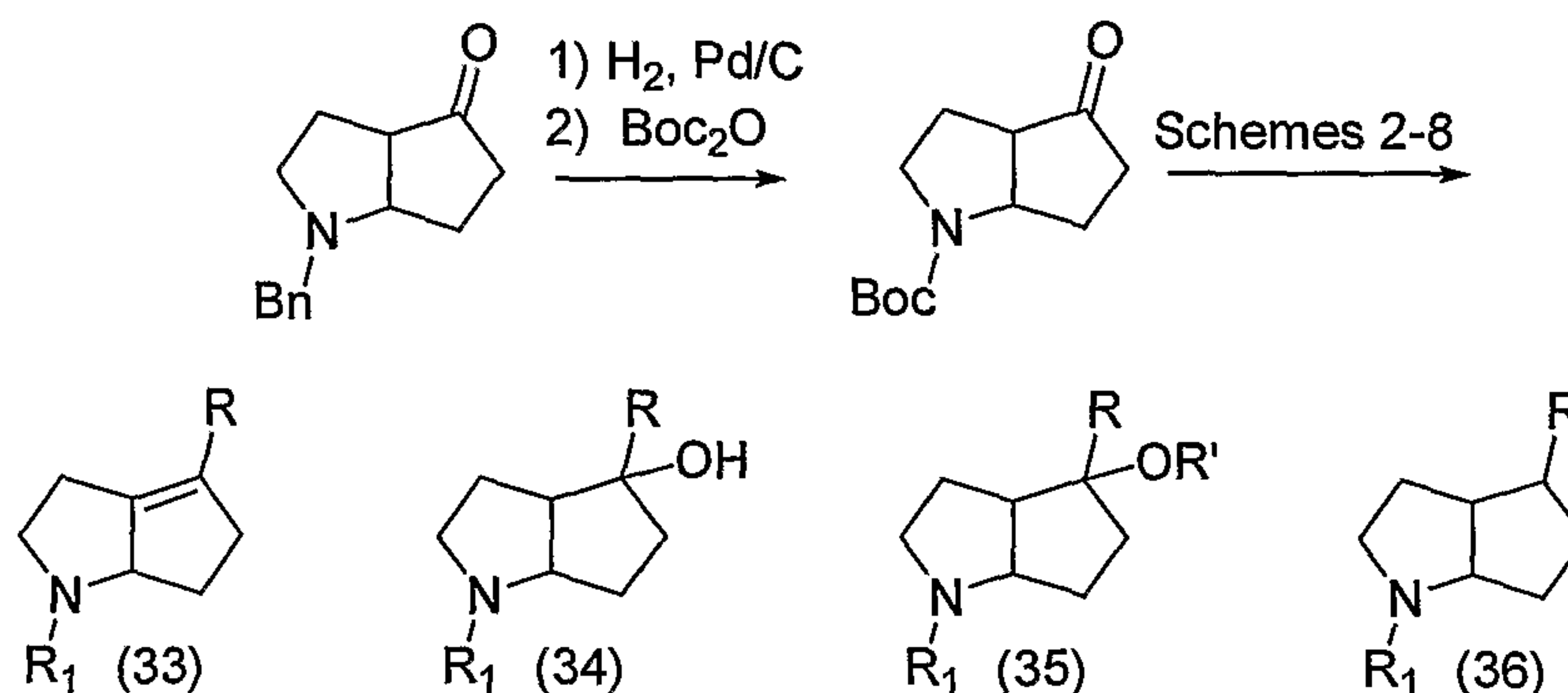
Scheme 10
