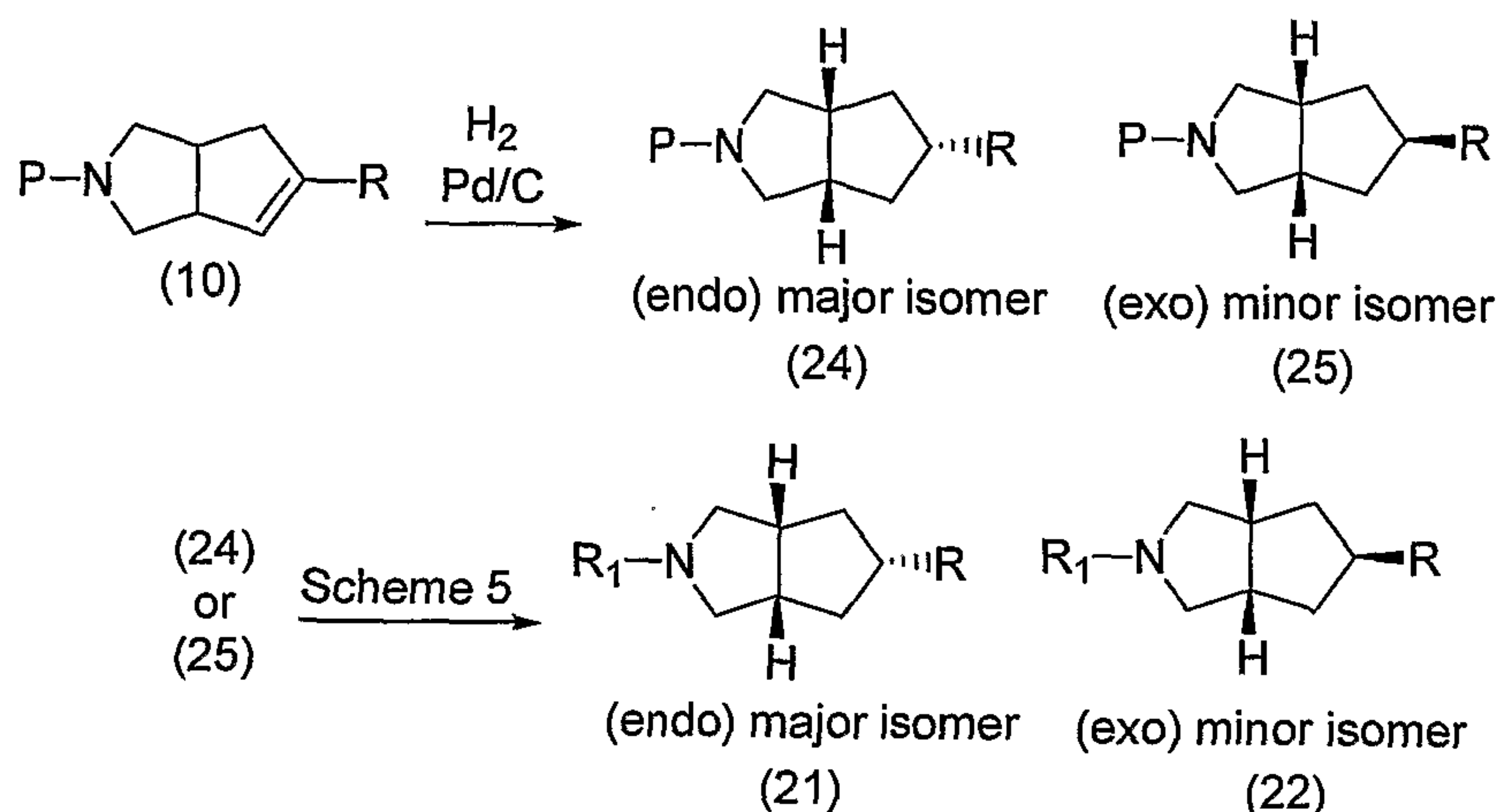
Scheme 8
