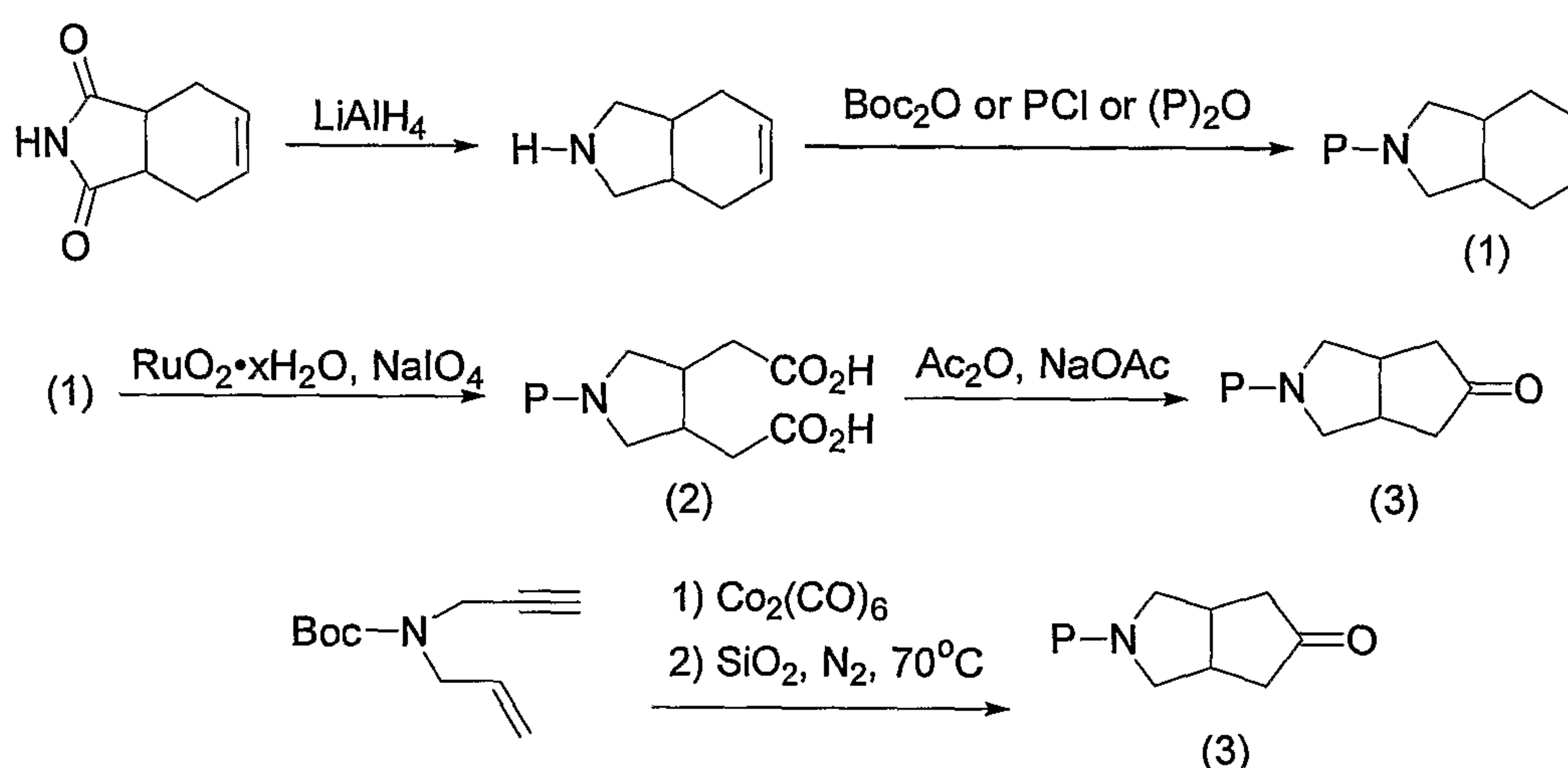
Scheme 1
