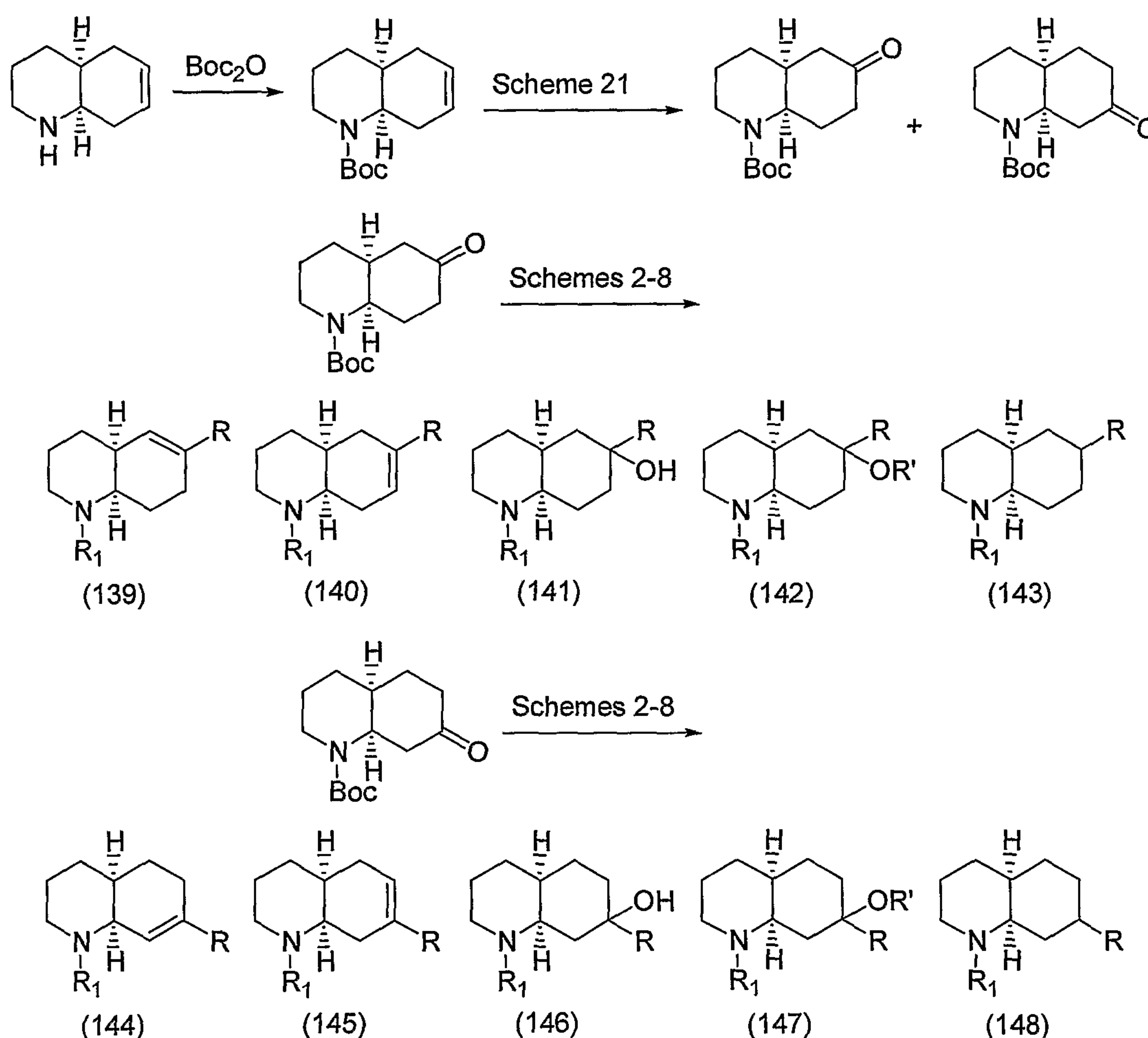
Scheme 31
