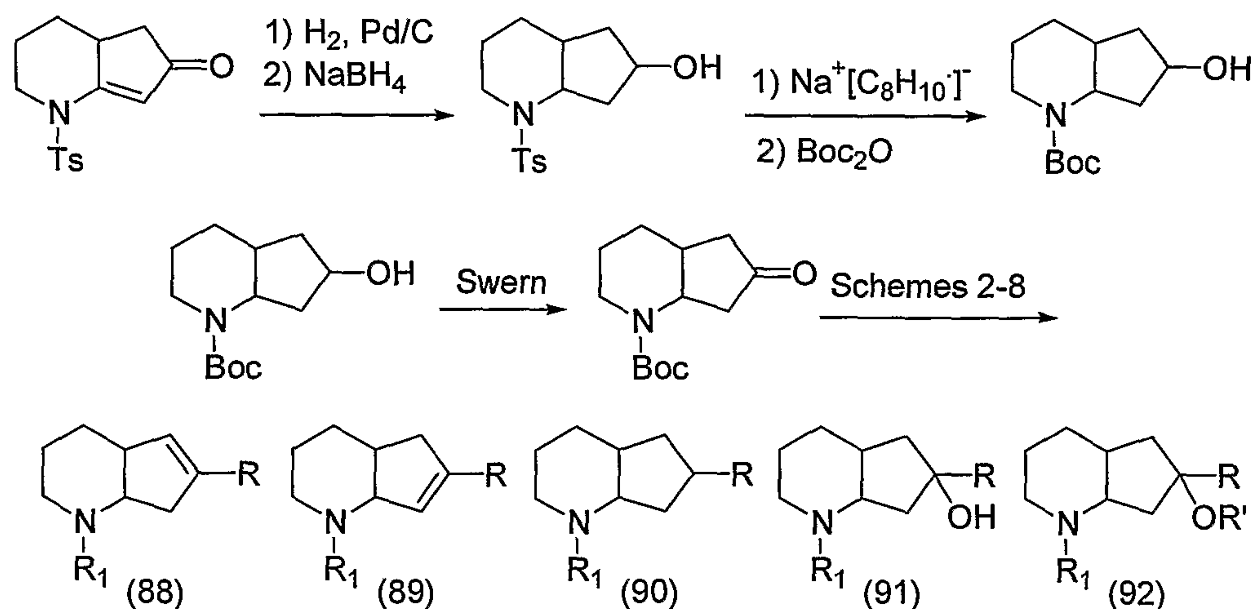
Scheme 22
