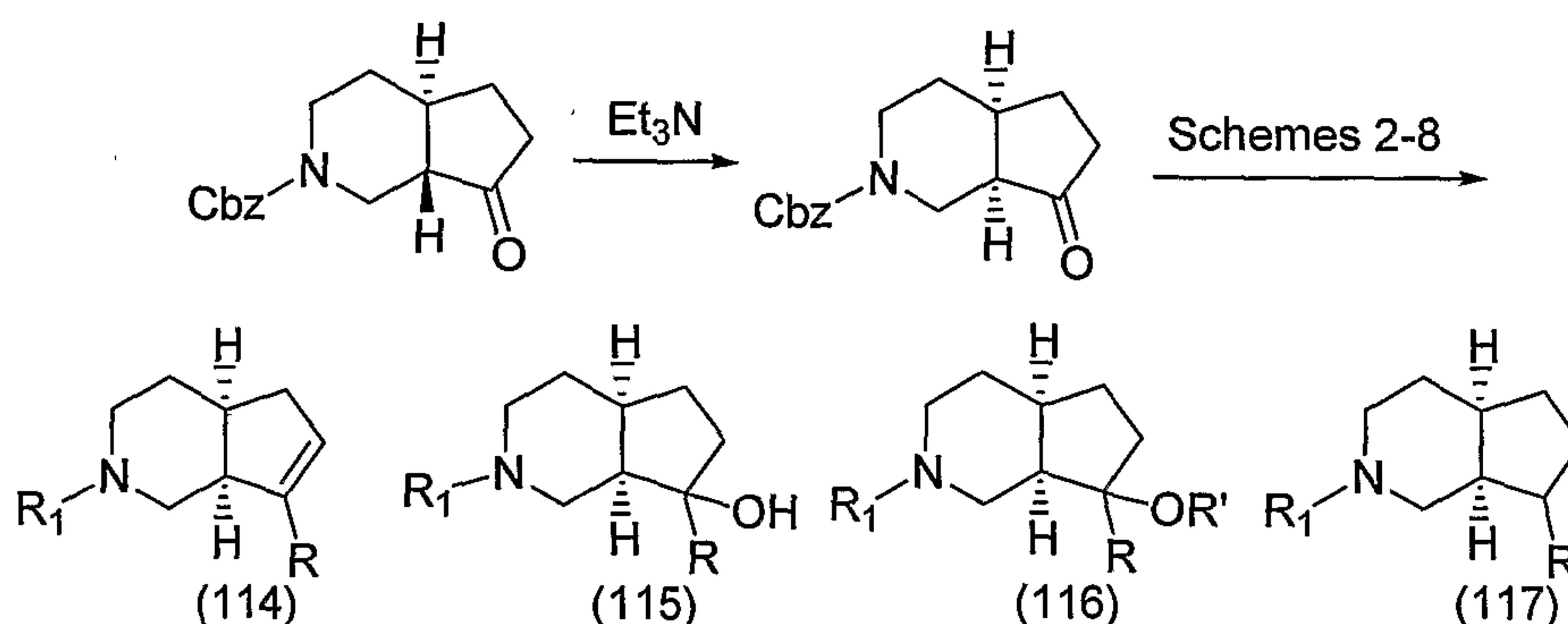
Scheme 27
