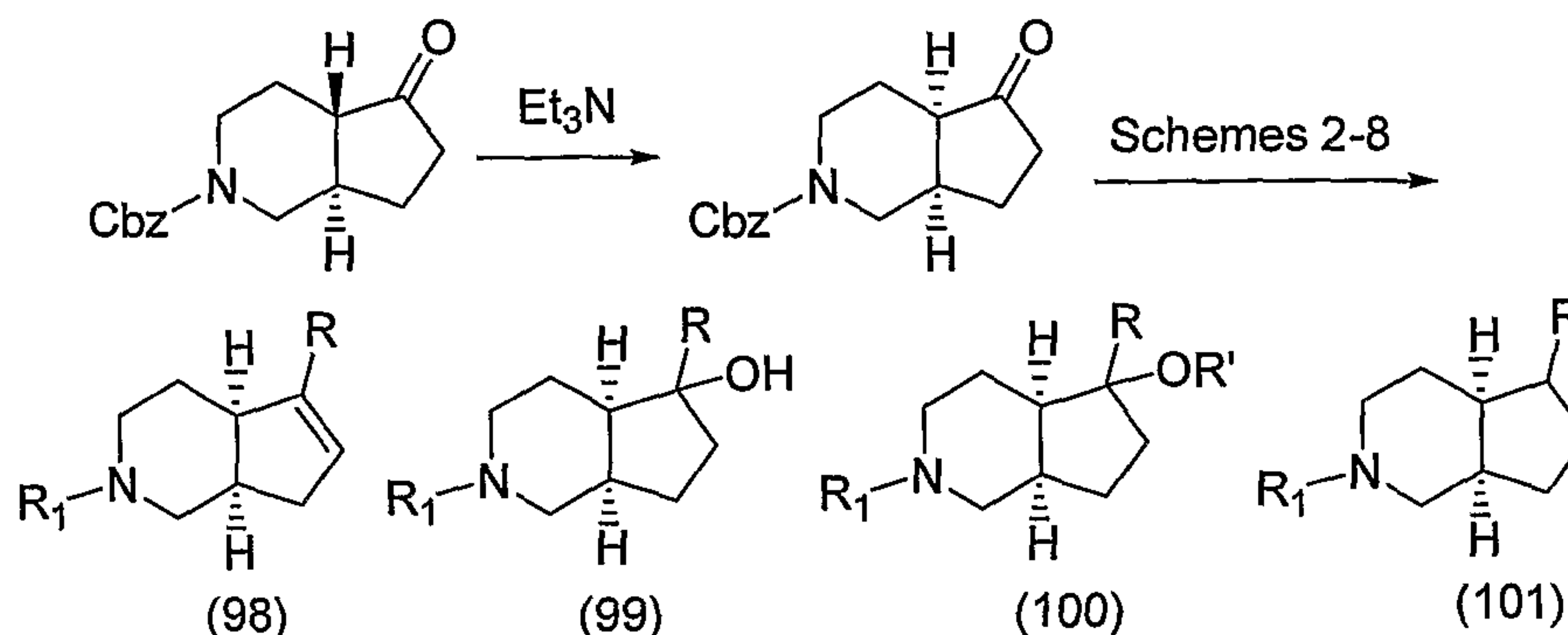
Scheme 24
