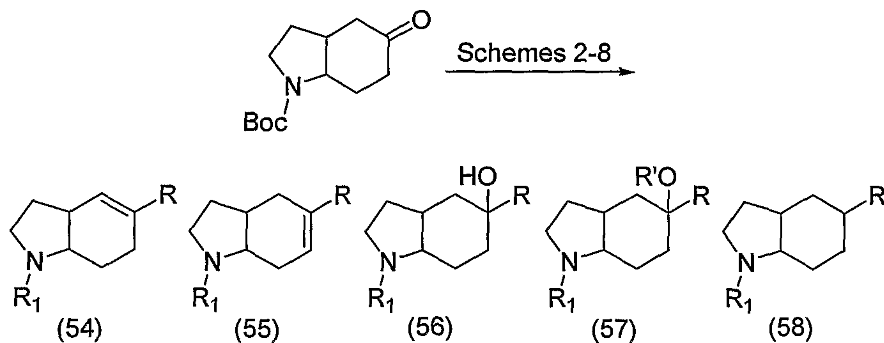
Scheme 14
