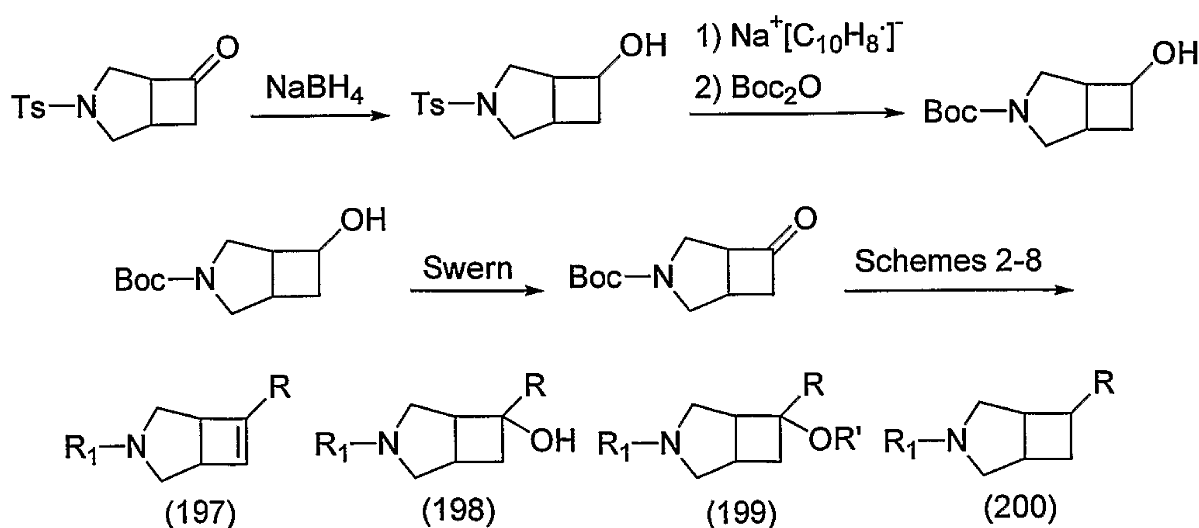
Scheme 41
