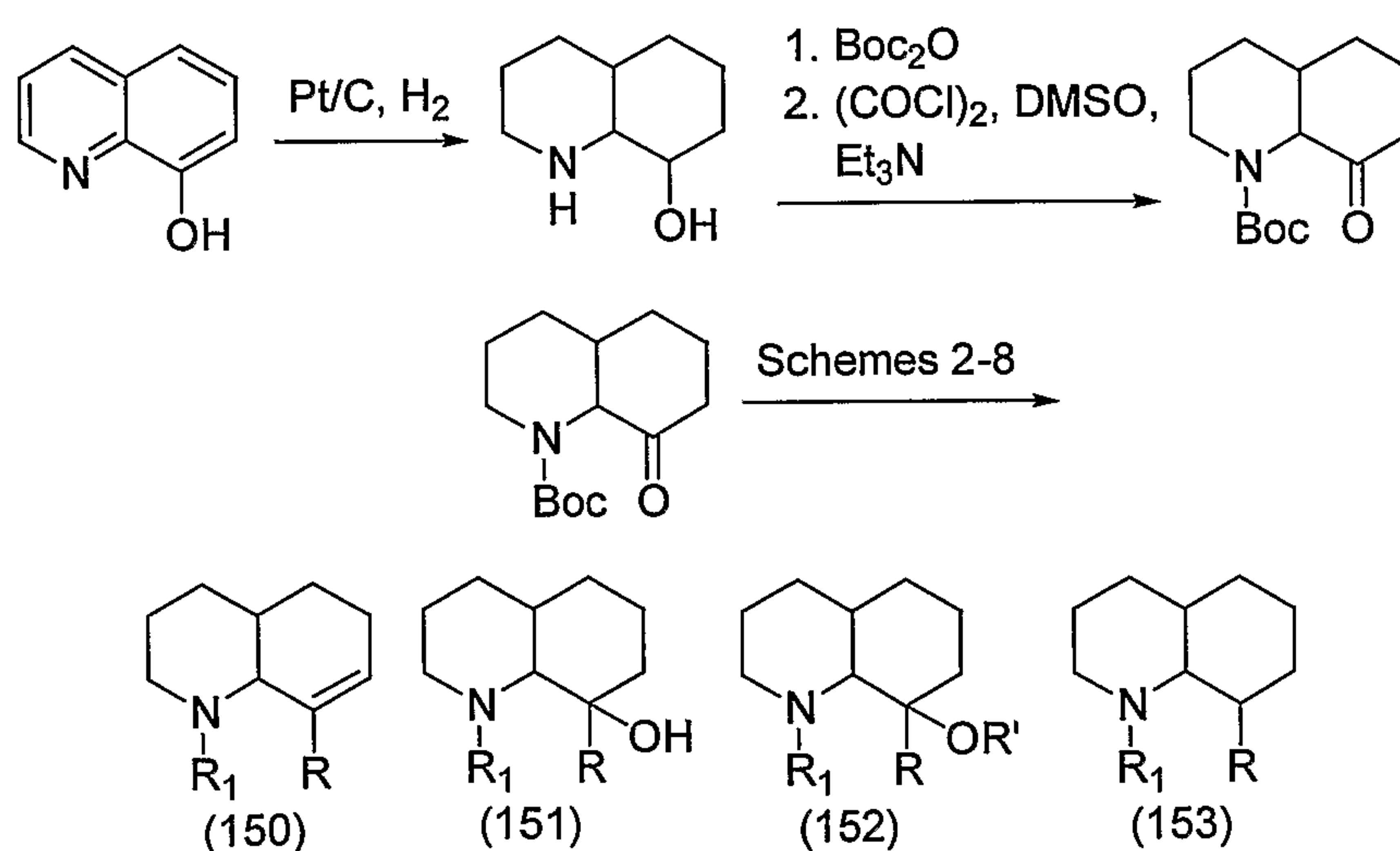
Scheme 32
