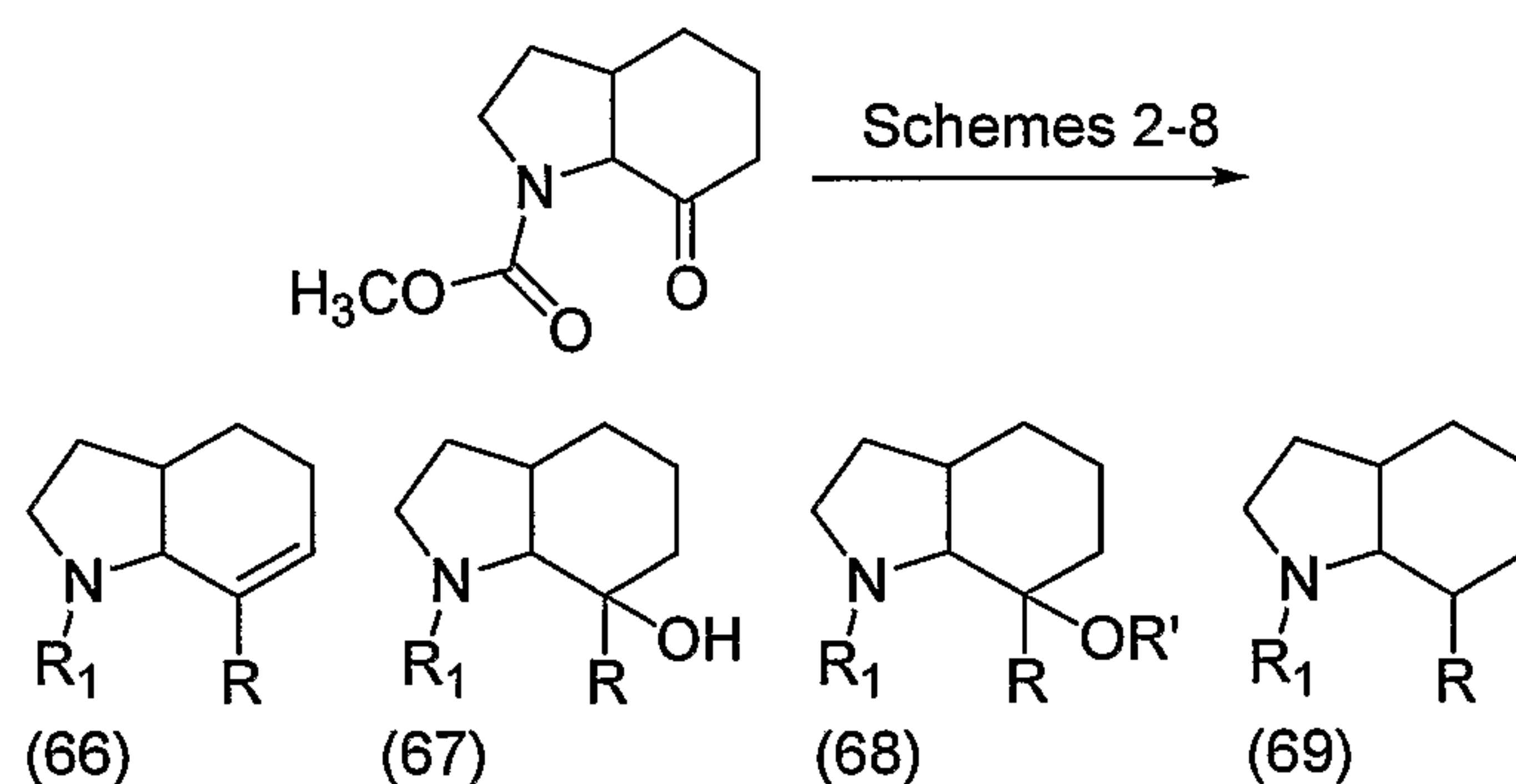
Scheme 16
