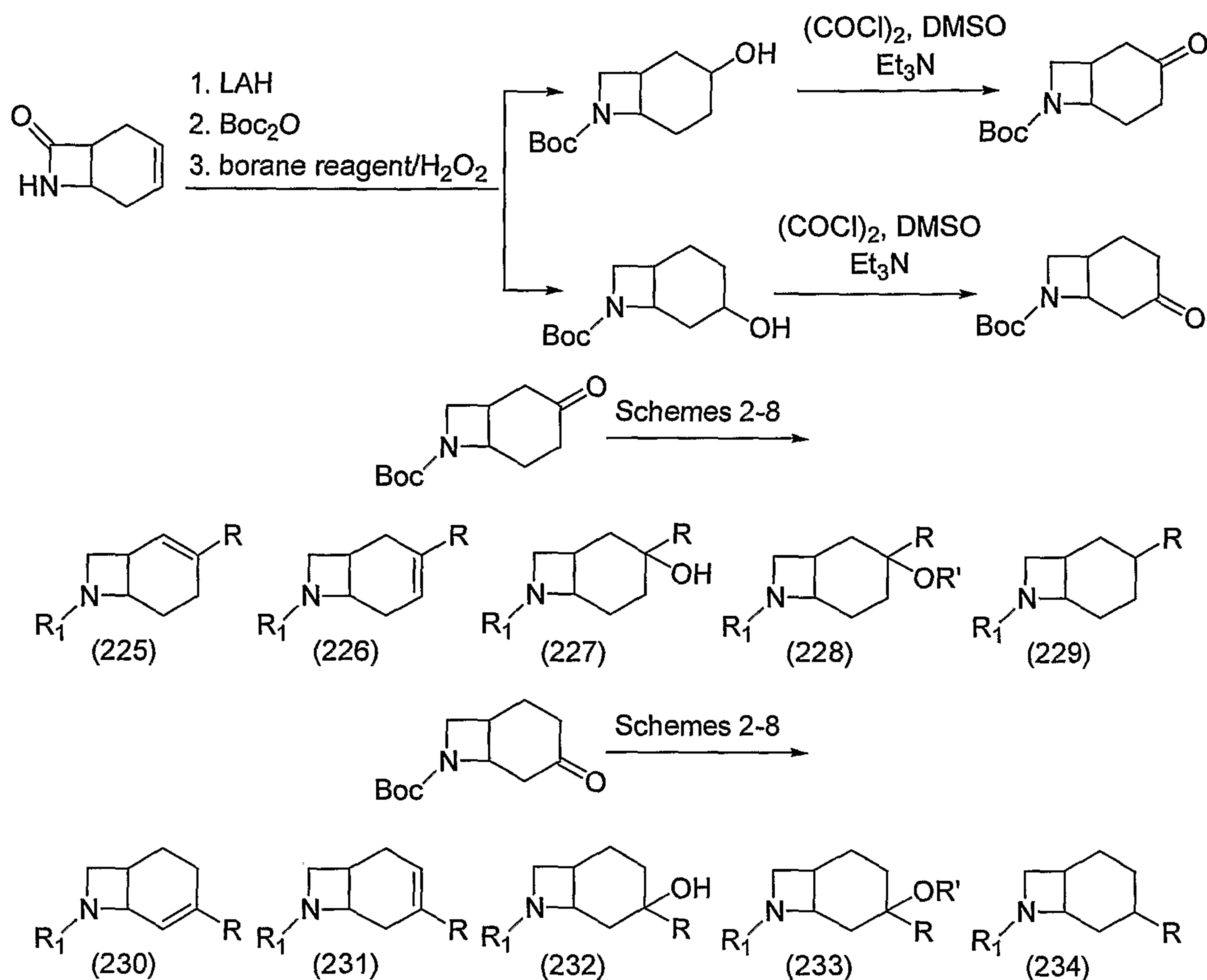
Scheme 46
