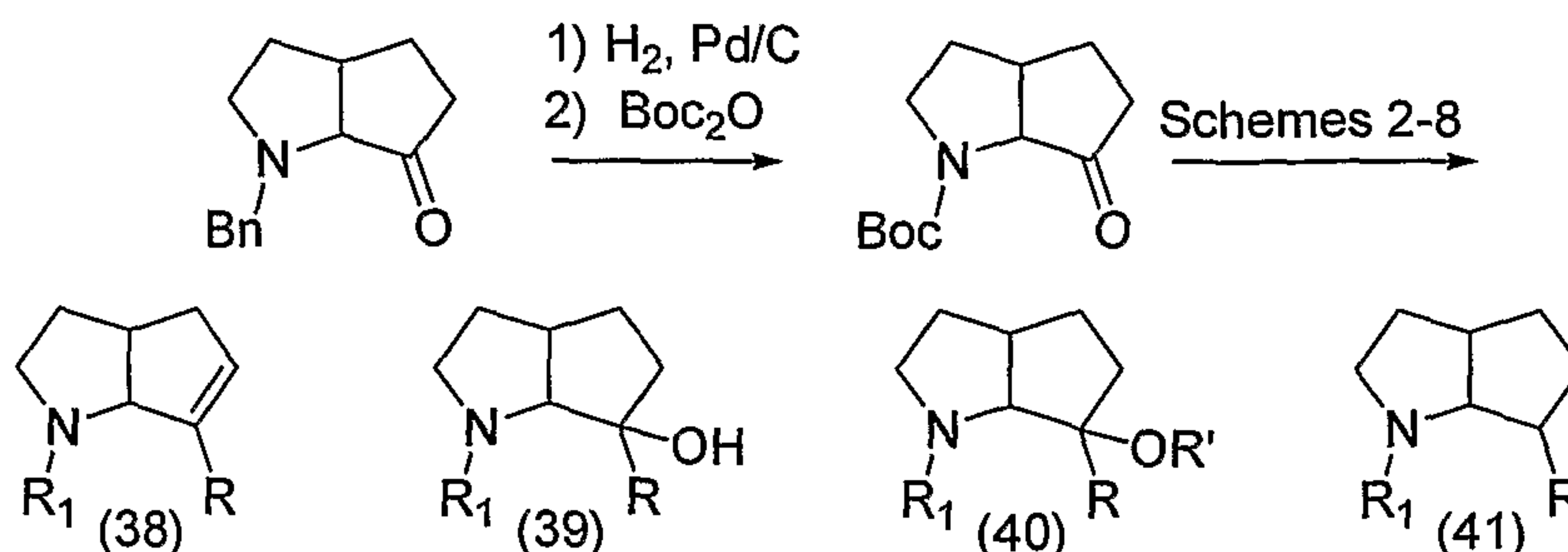
Scheme 11
