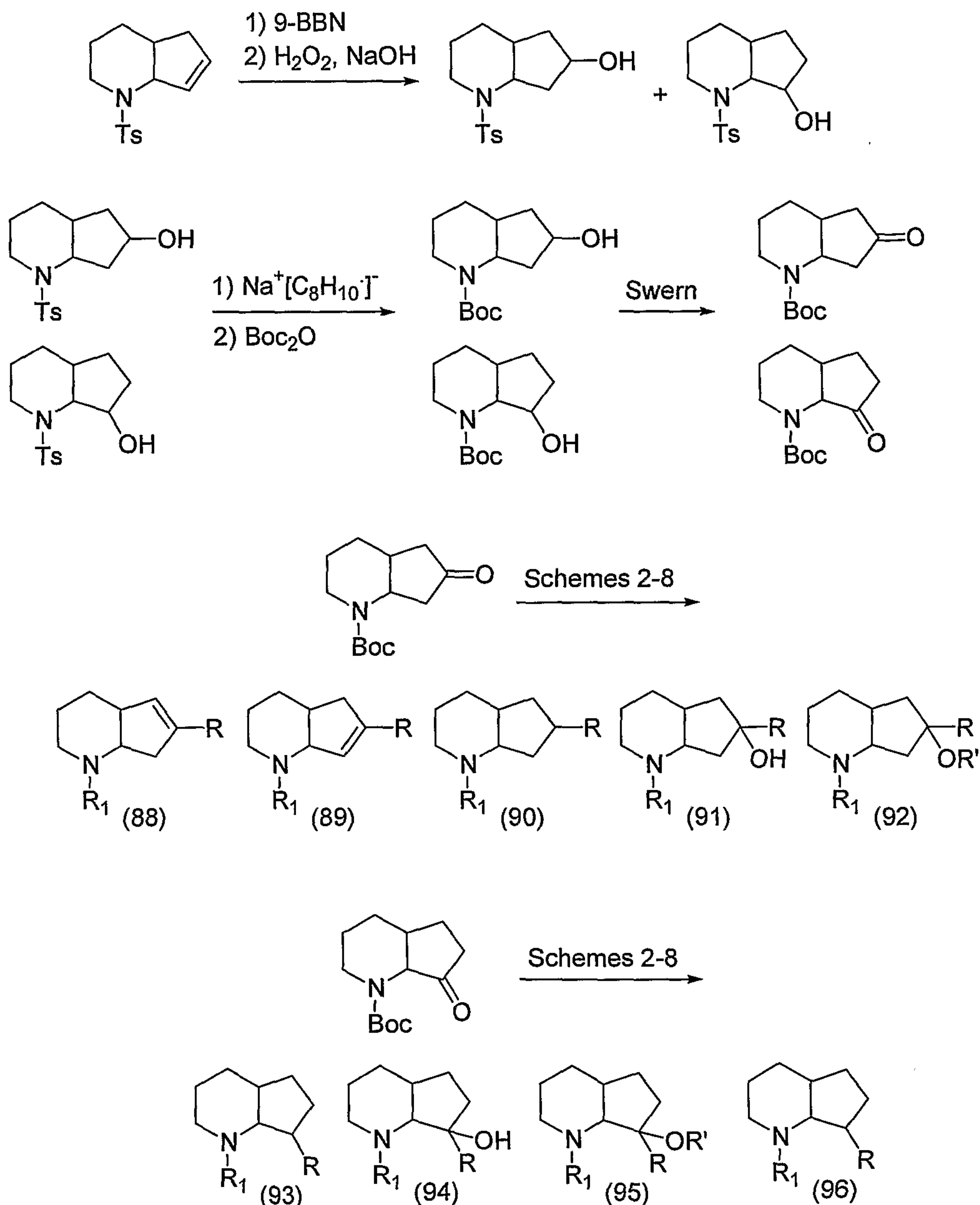
Scheme 21
