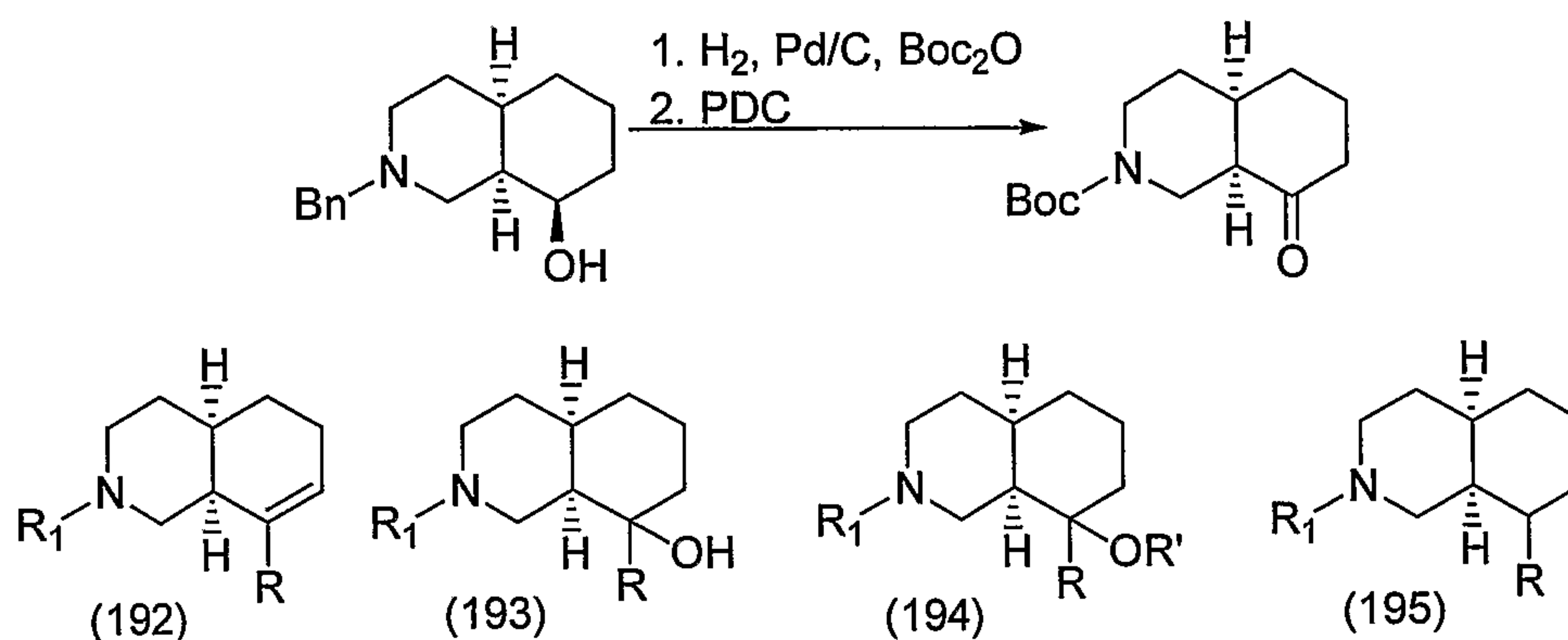
Scheme 40
