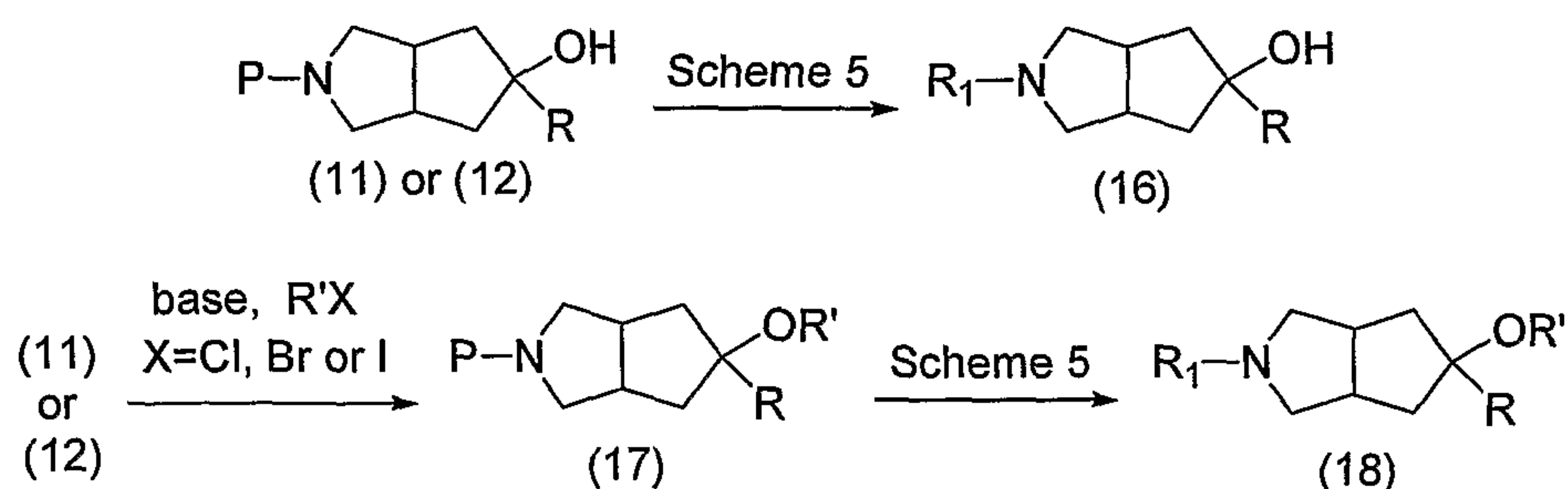
Scheme 6
