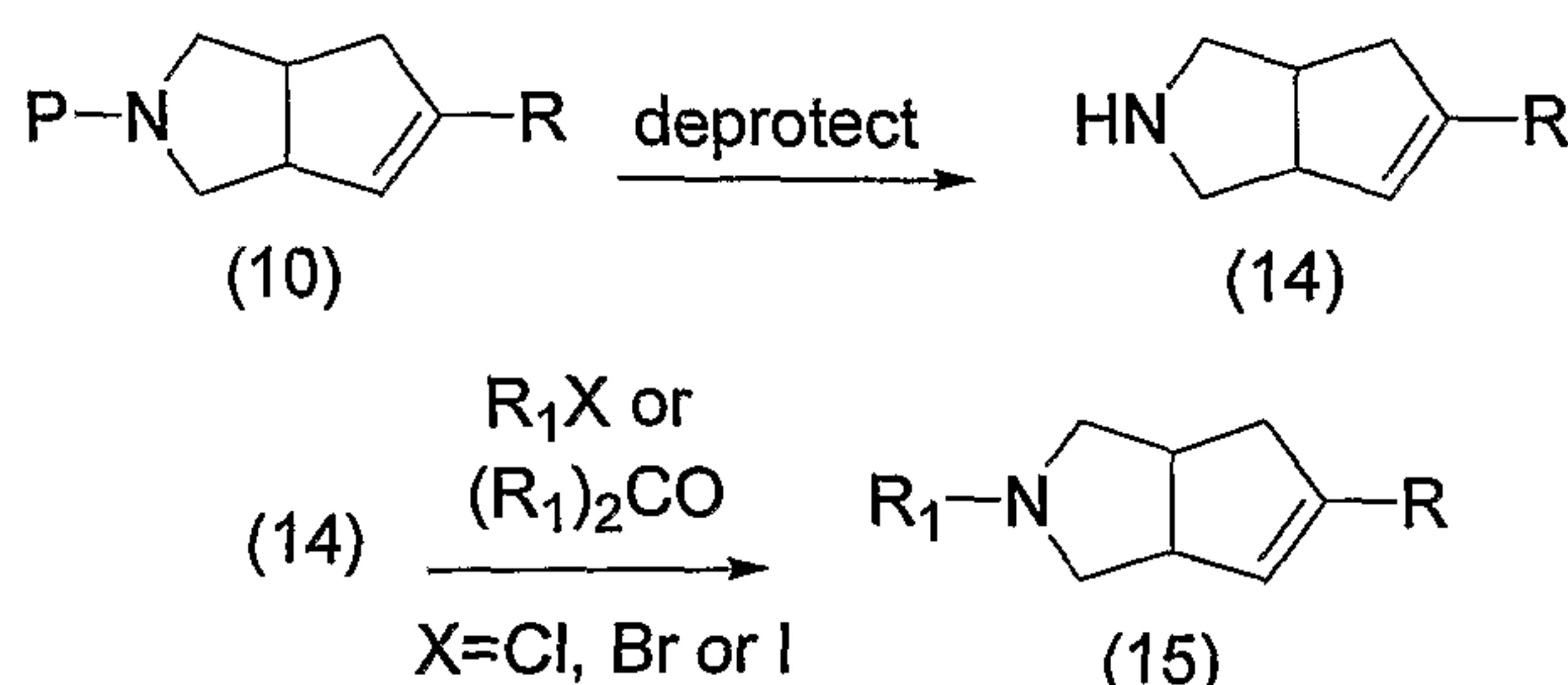
Scheme 5
