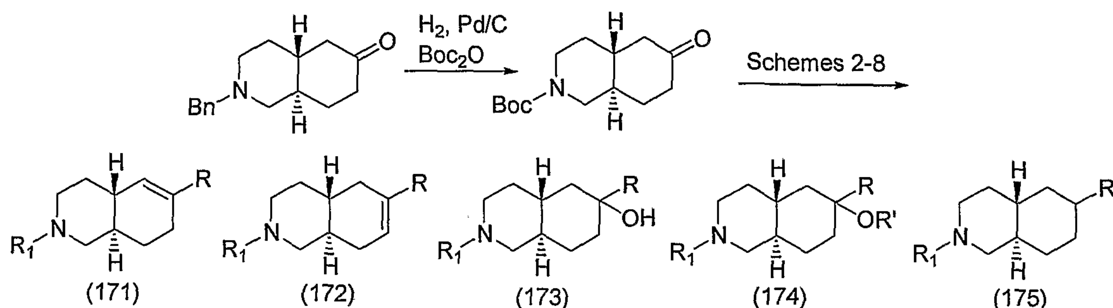
Scheme 36
