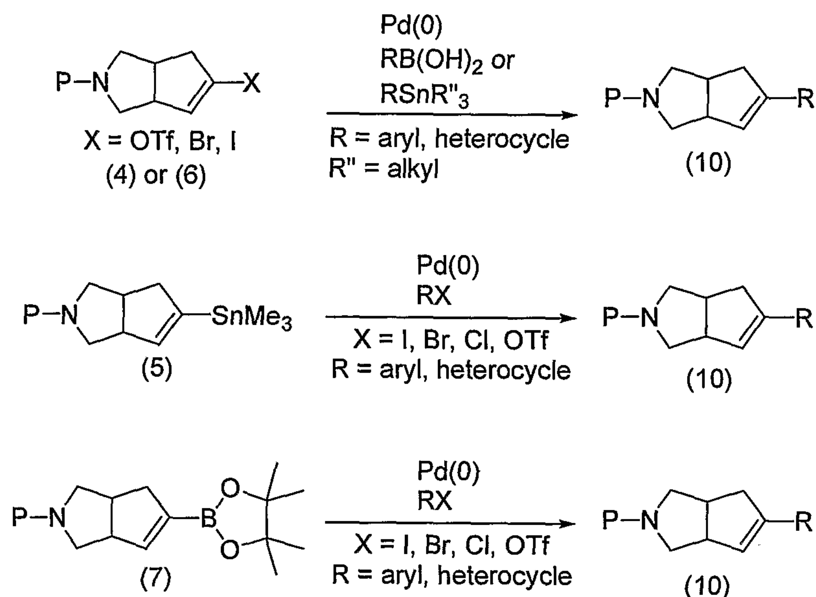
Scheme 3
