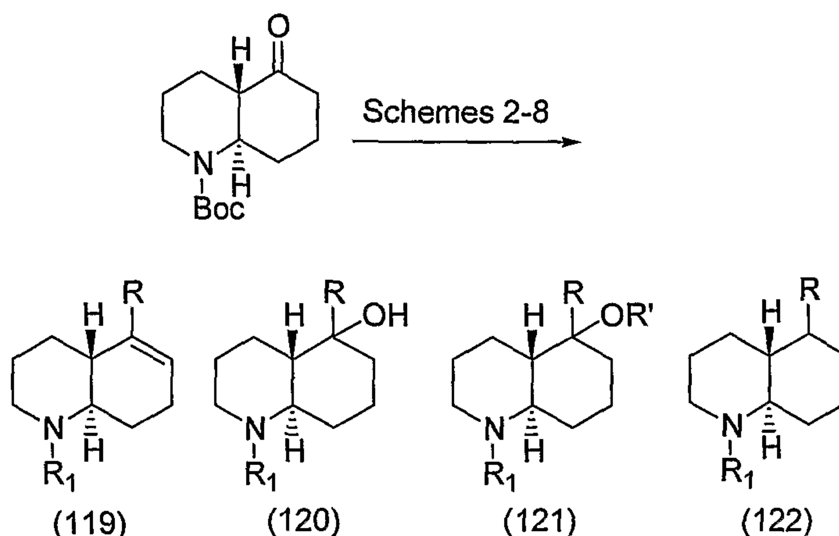
Scheme 28
