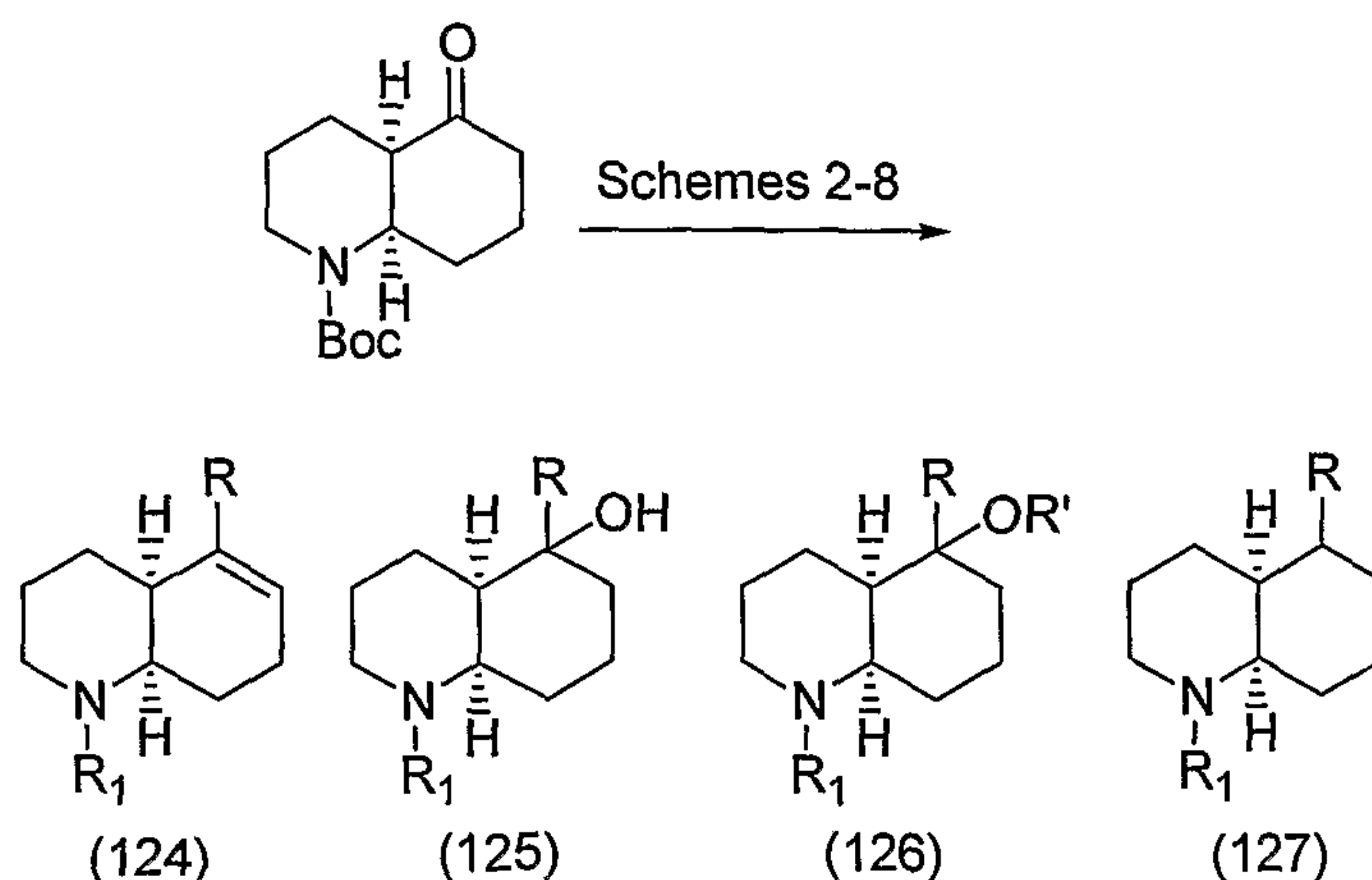
Scheme 29
