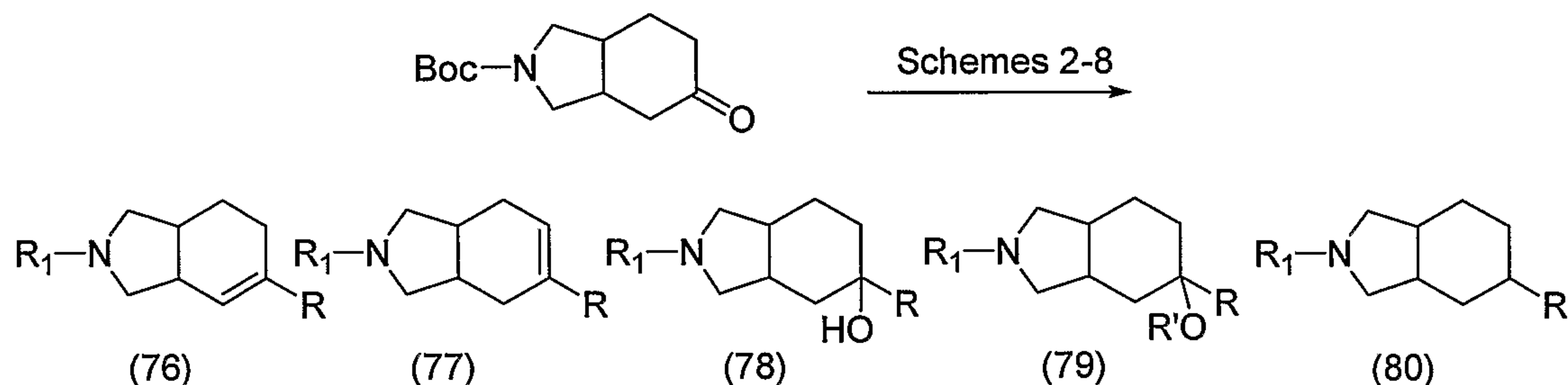
Scheme 18
