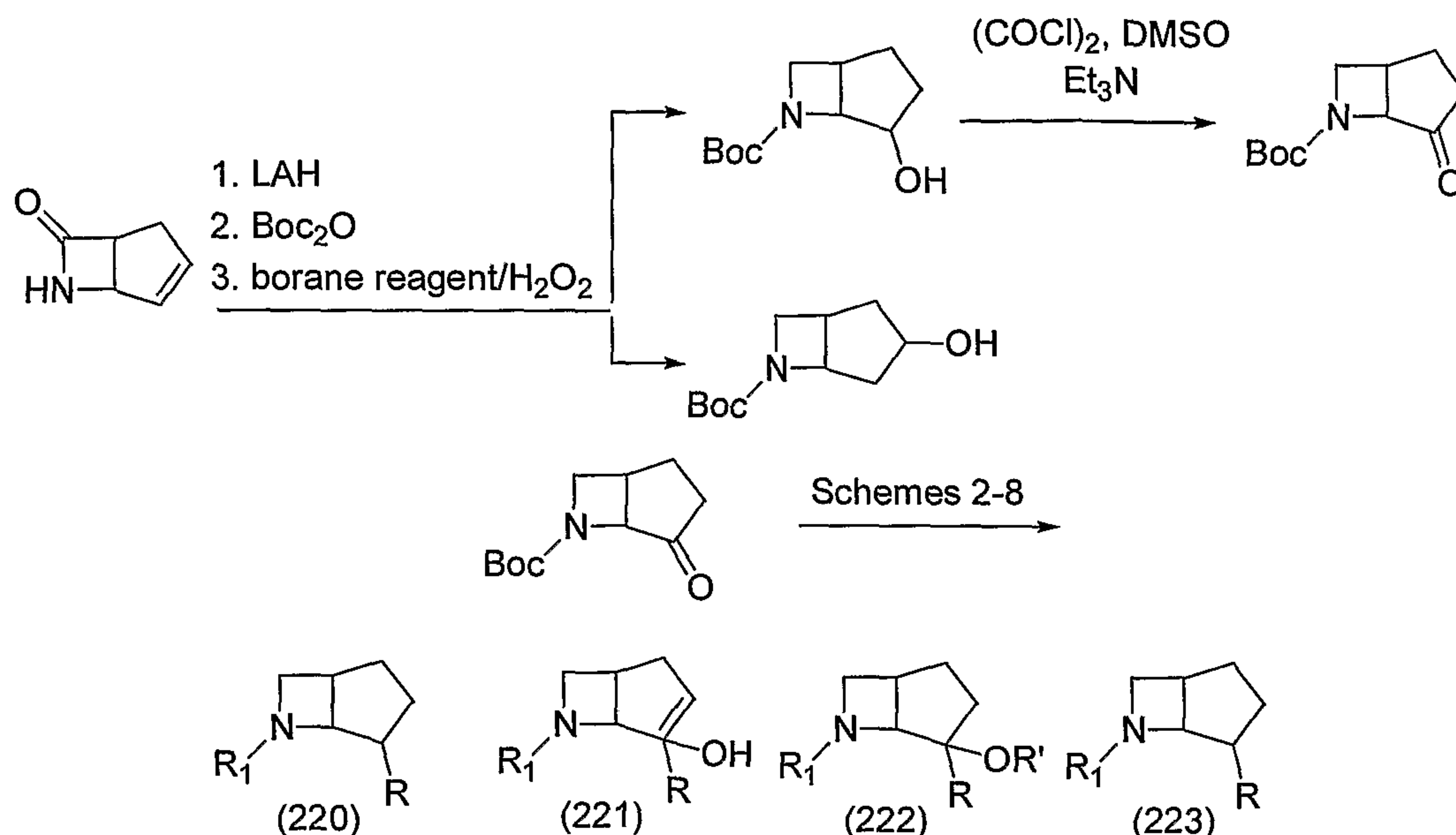
Scheme 45
