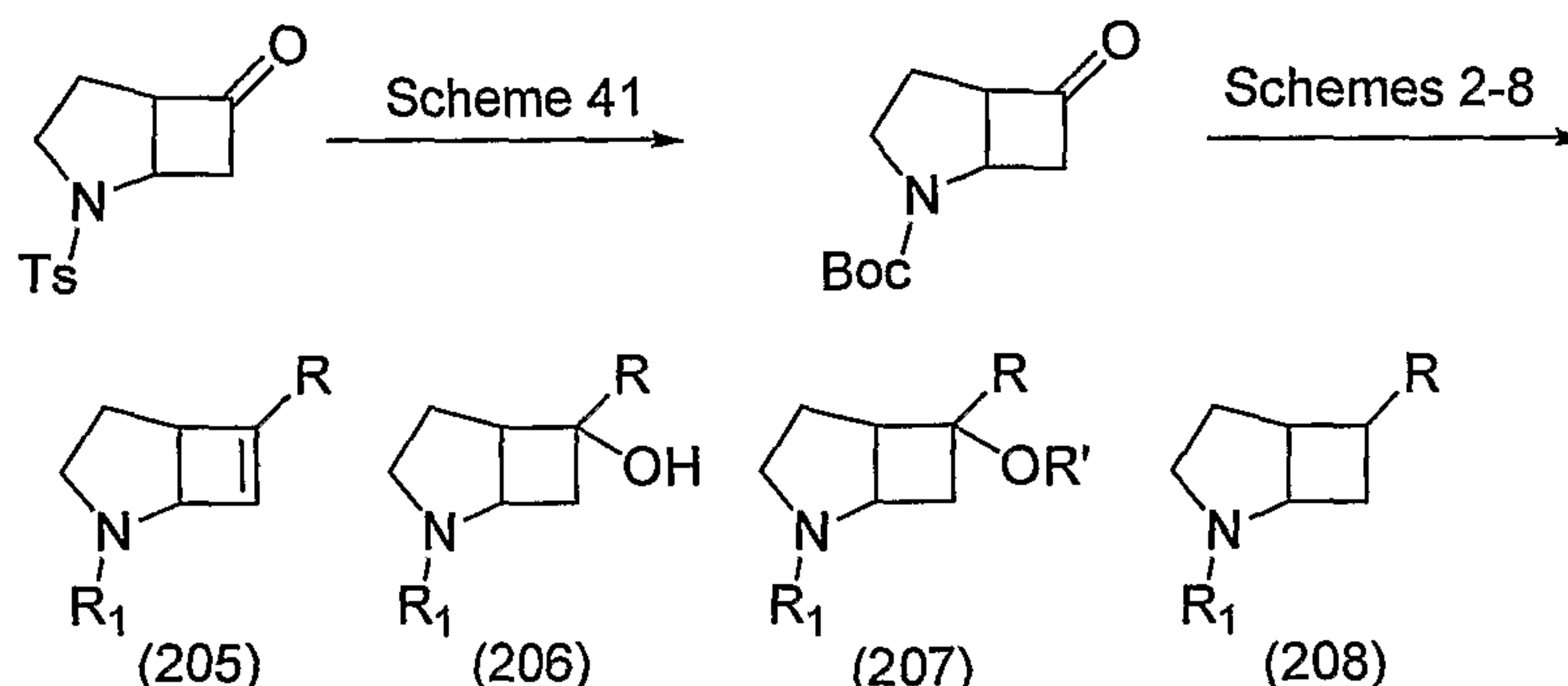
Scheme 43
