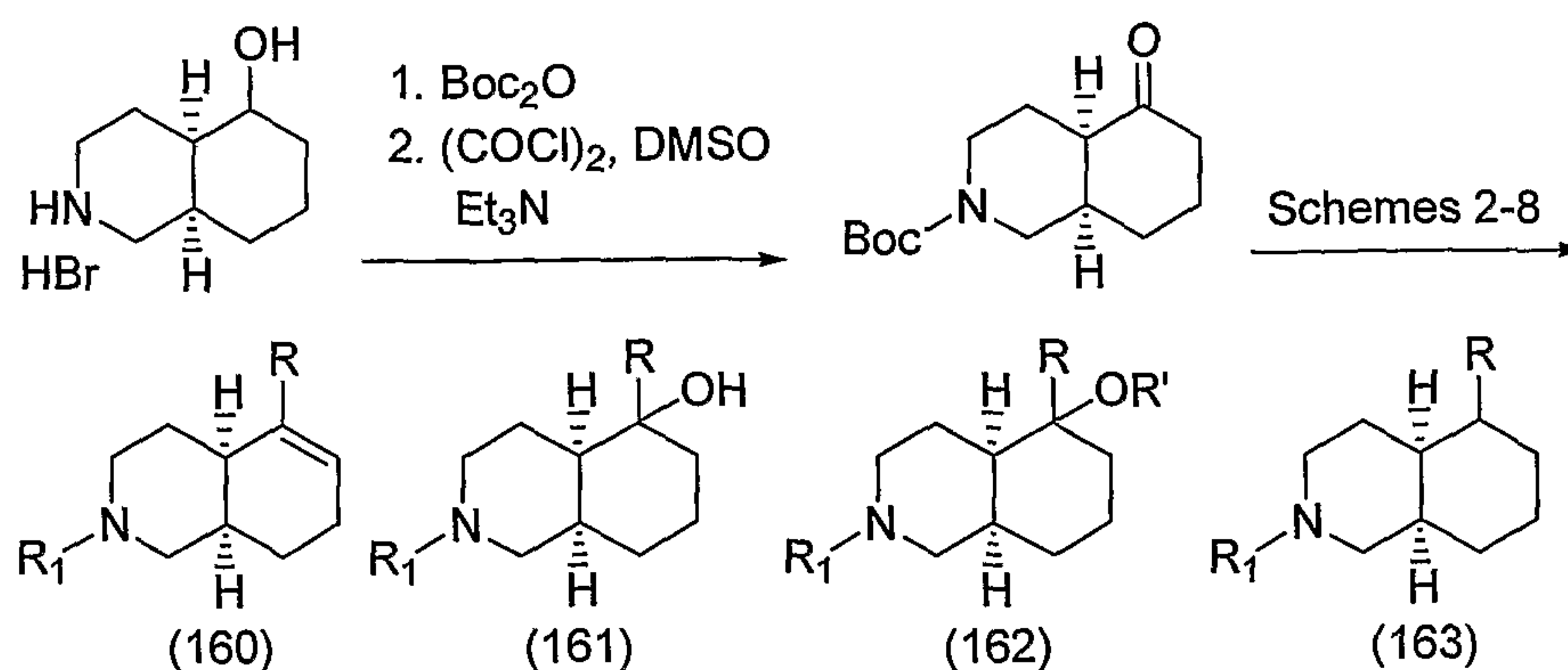
Scheme 34
