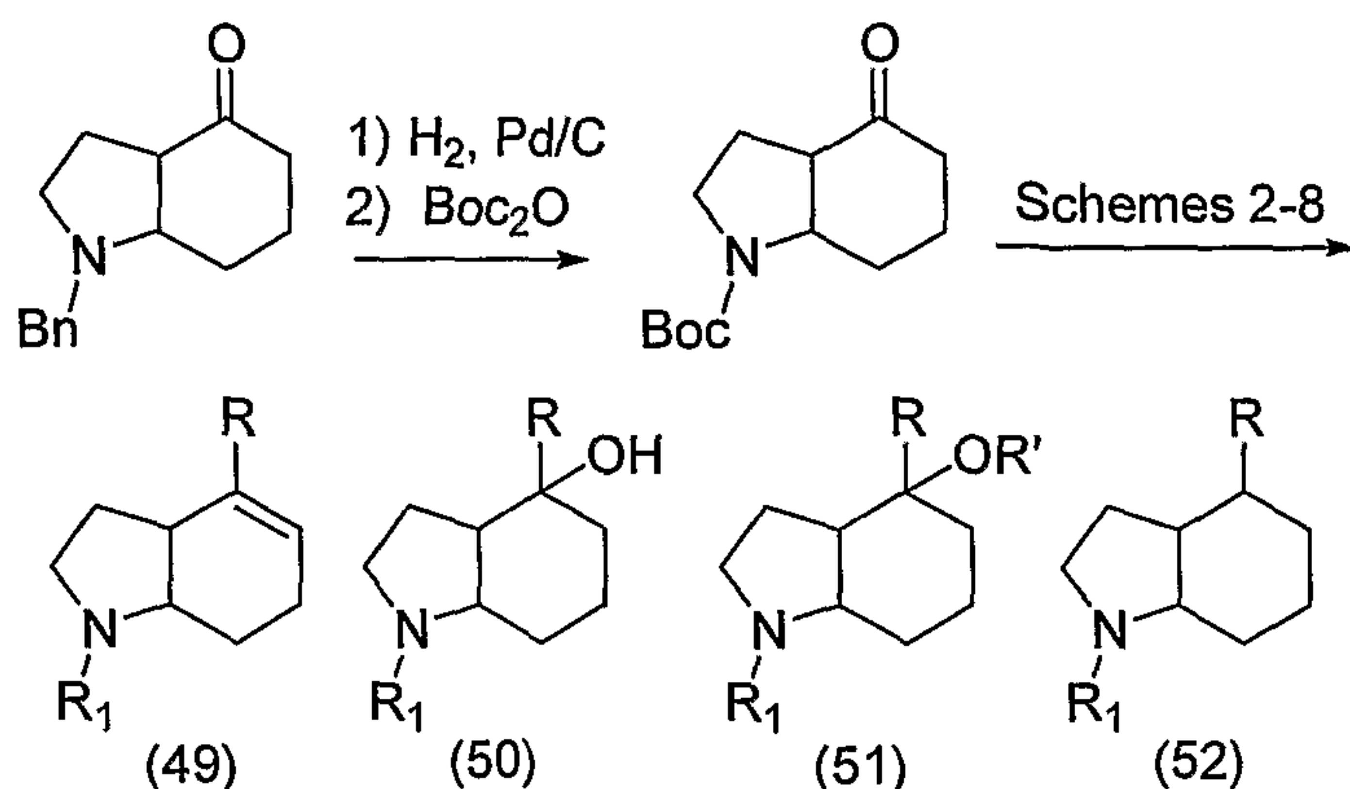
Scheme 13
