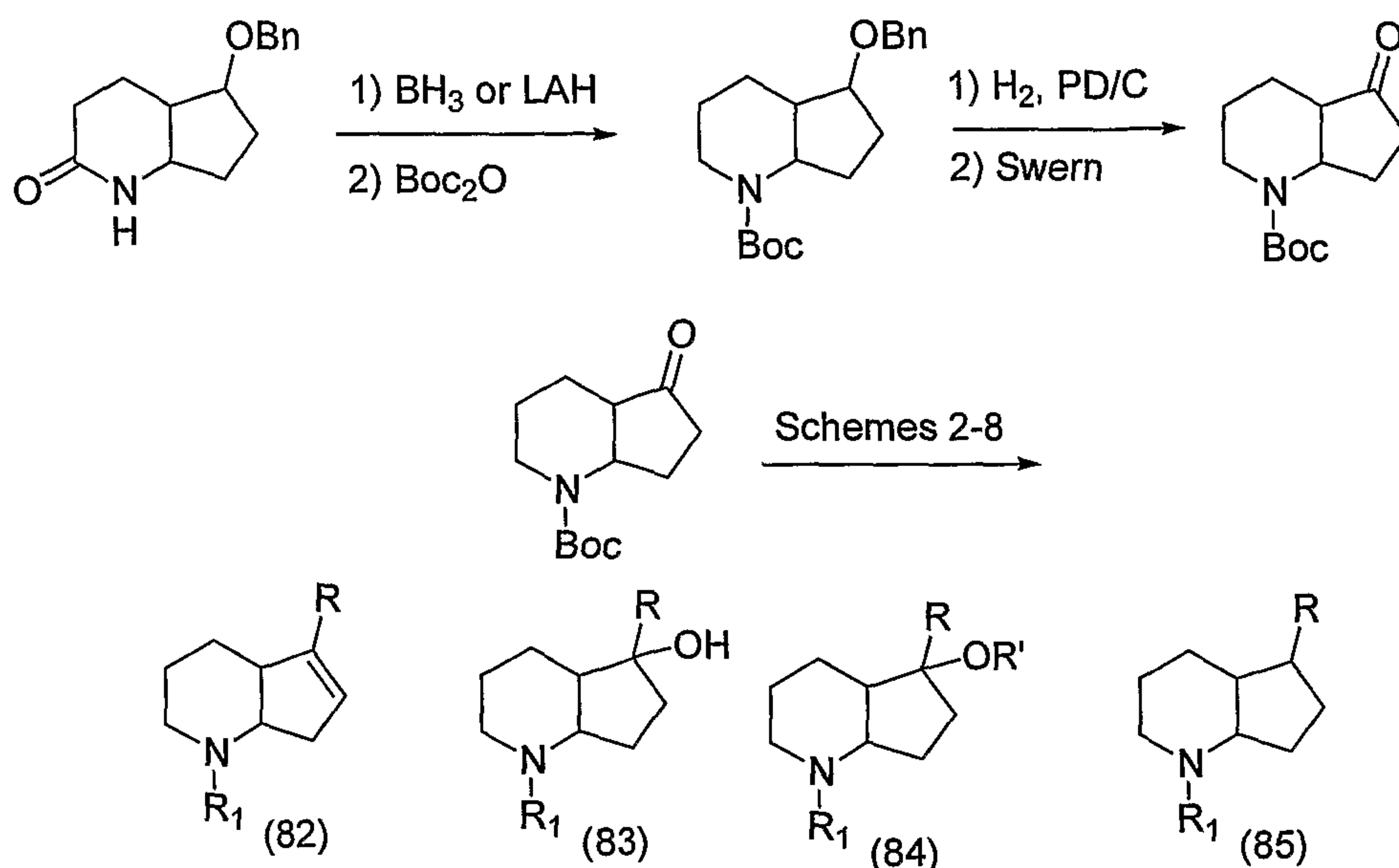
Scheme 19
