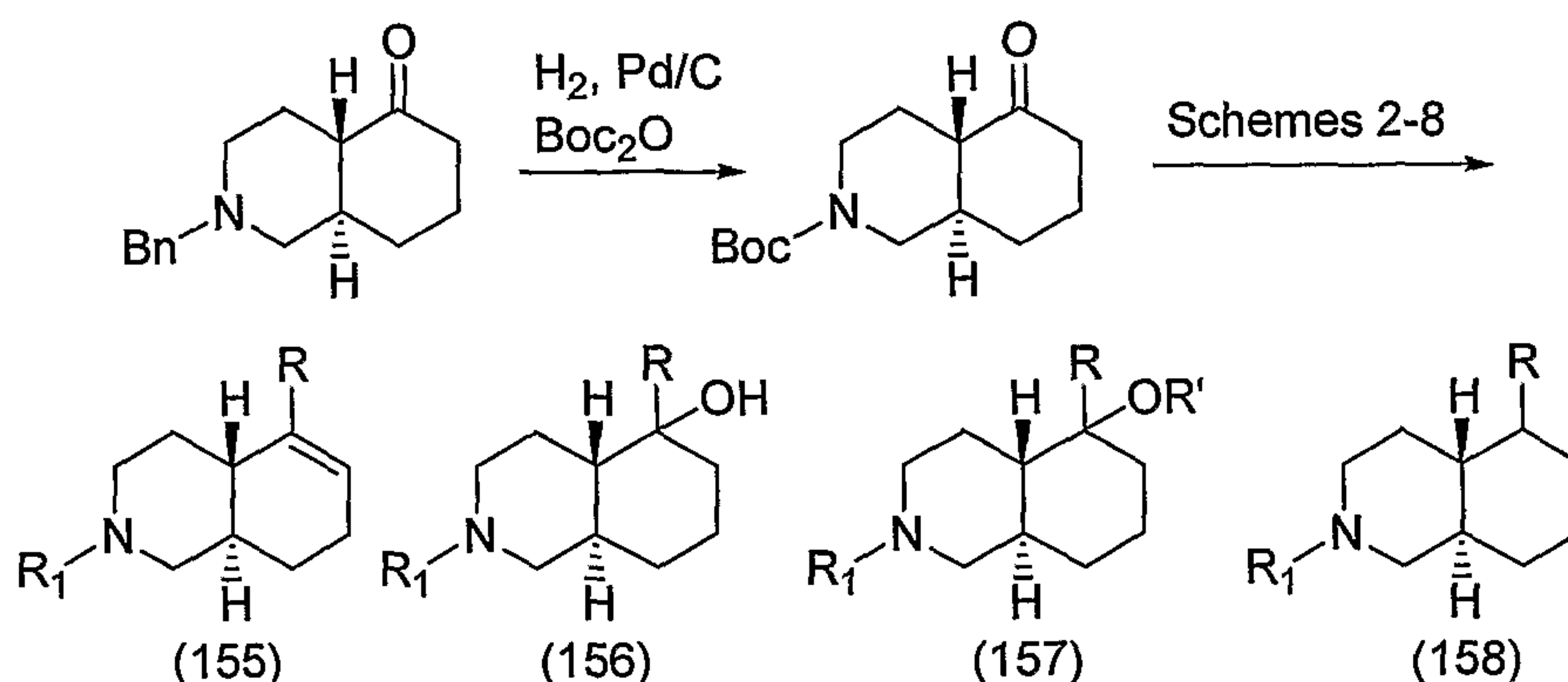
Scheme 33
