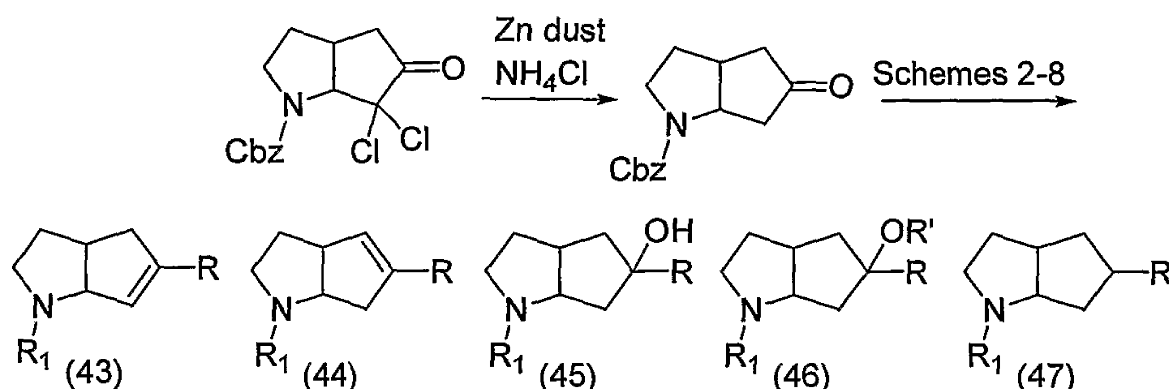
Scheme 12
