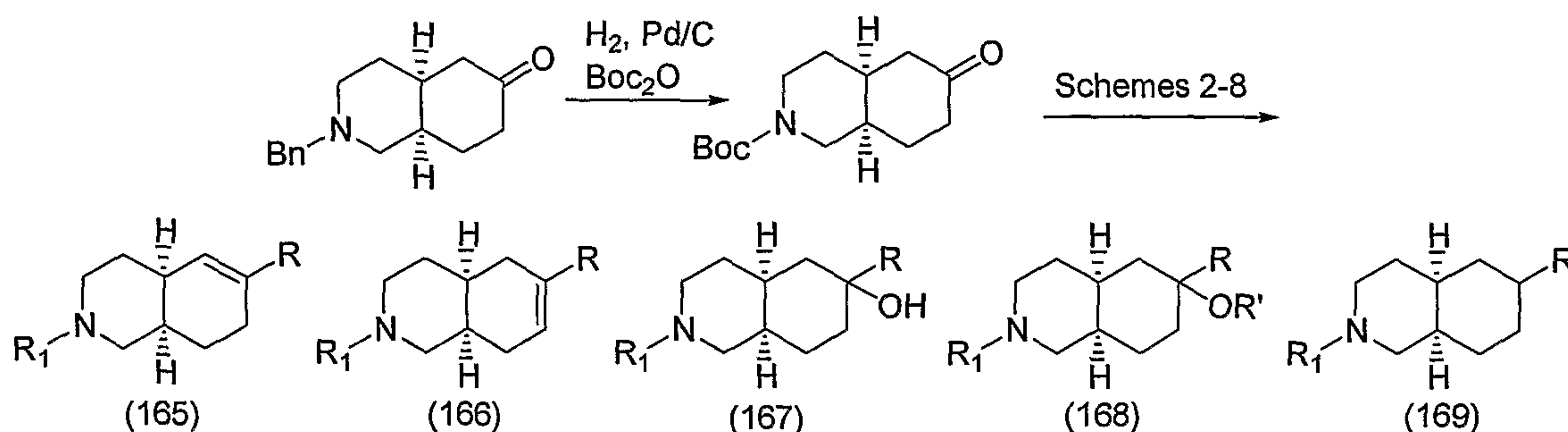
Scheme 35
