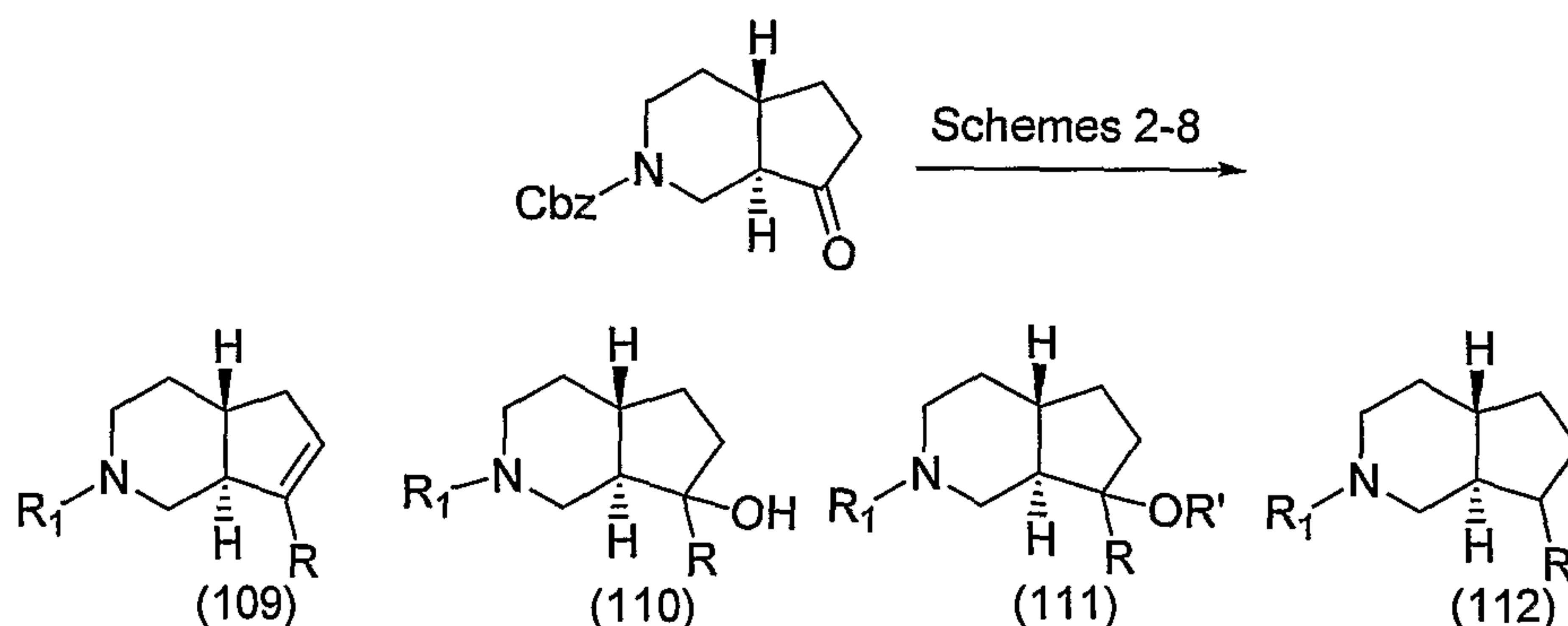
Scheme 26
