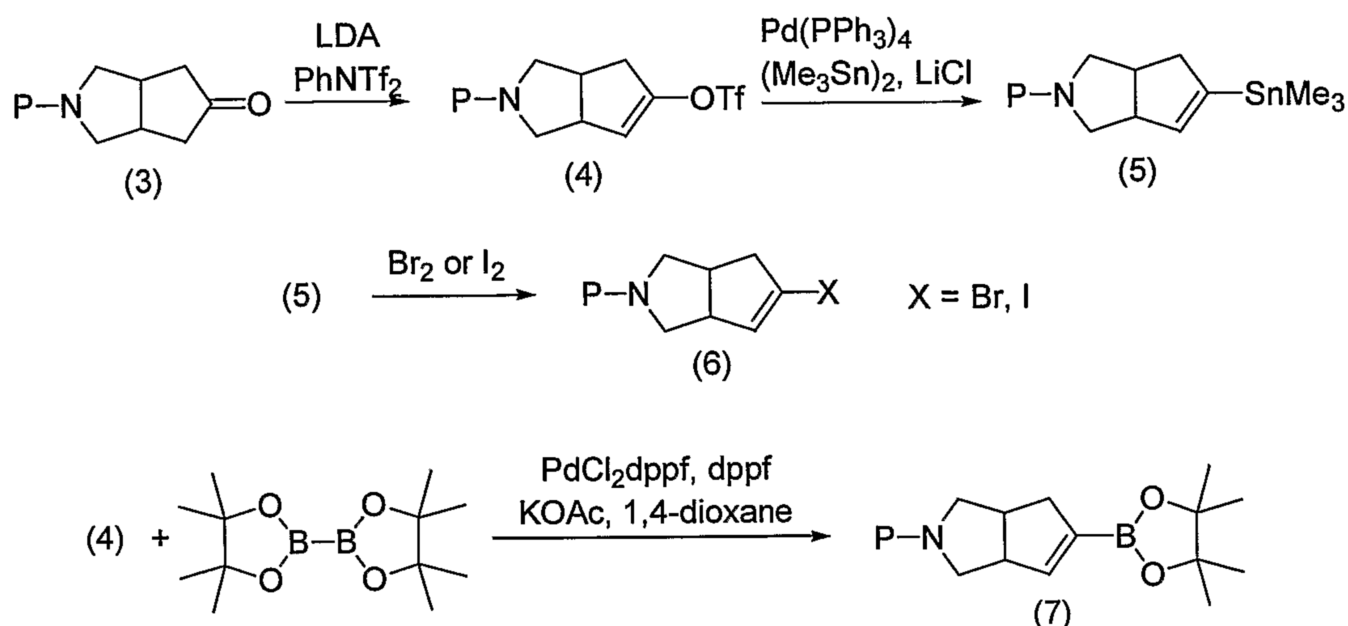
Scheme 2
