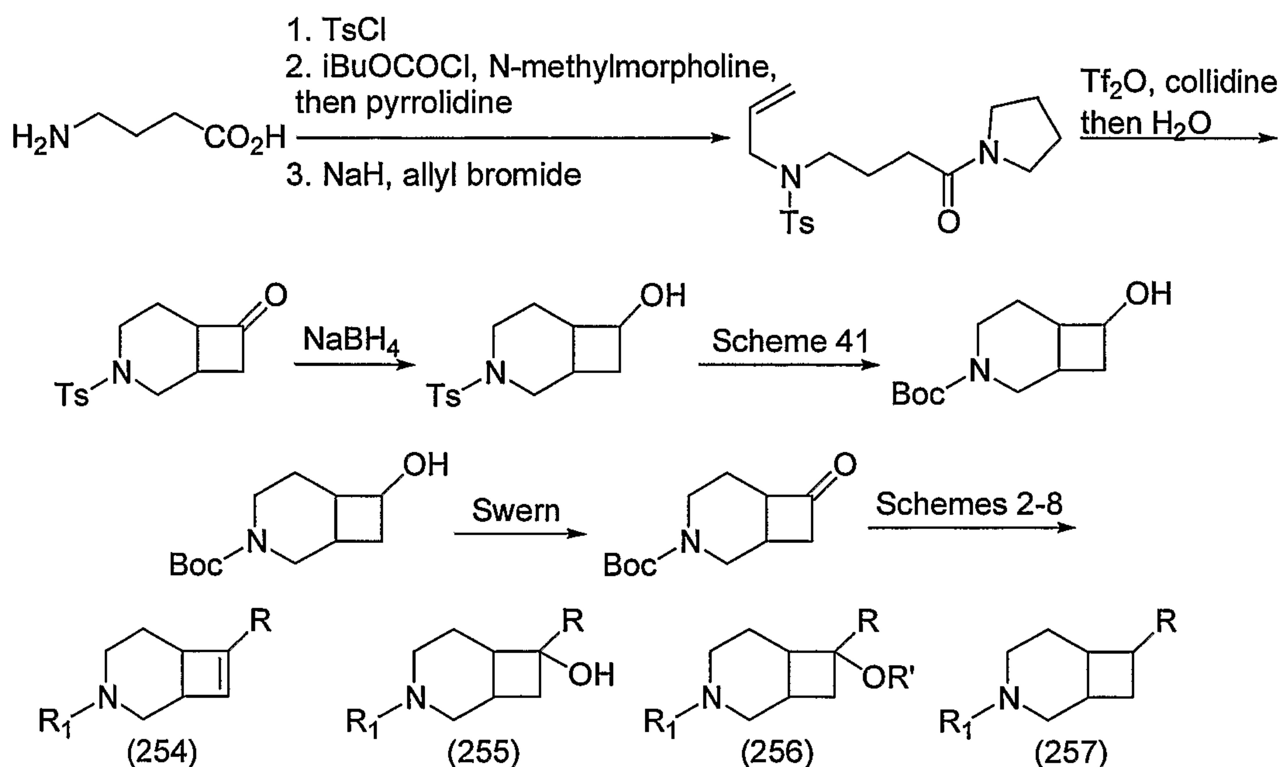
Scheme 51
