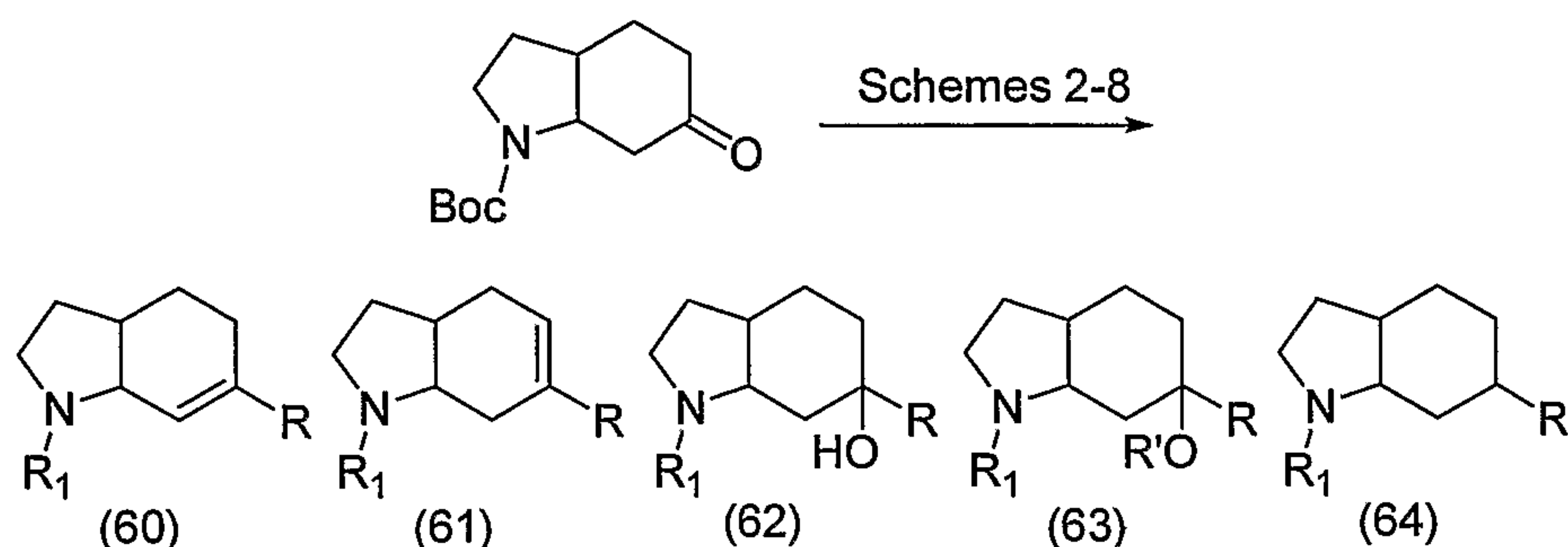
Scheme 15
