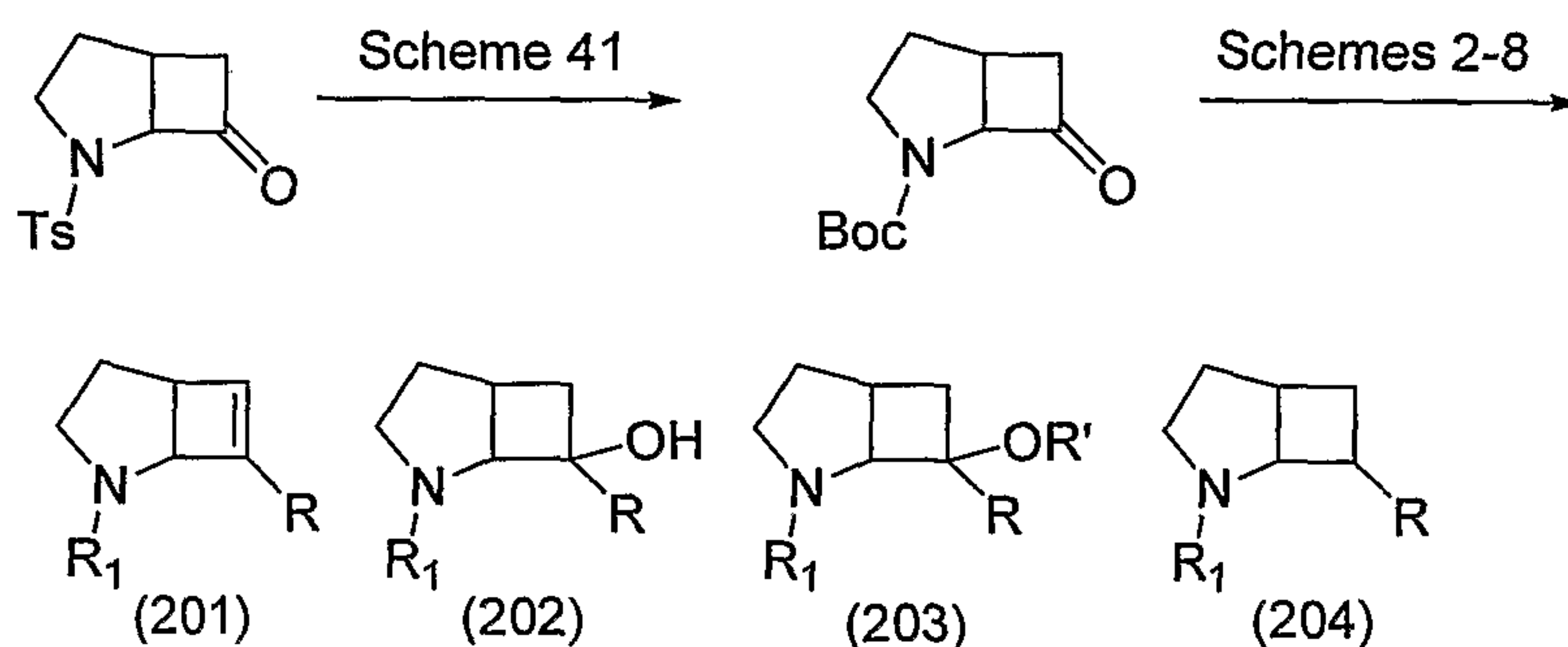
Scheme 42
