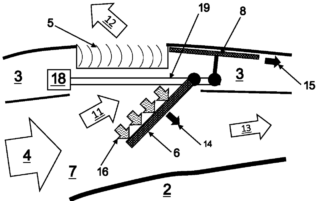
Detail A
