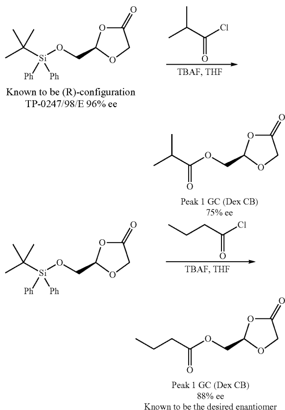
Scheme 13: Determination of configuration for Compound 13
