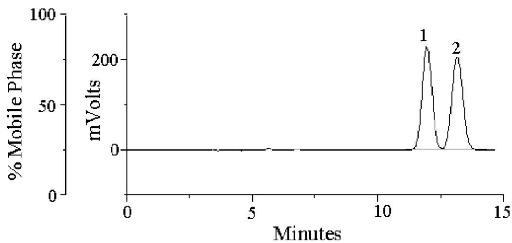
Figure 1C: HPLC method, Compound 11
