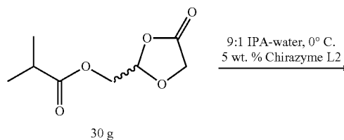
Scheme 8: Conditions identified for the bioresolution of compound 13
