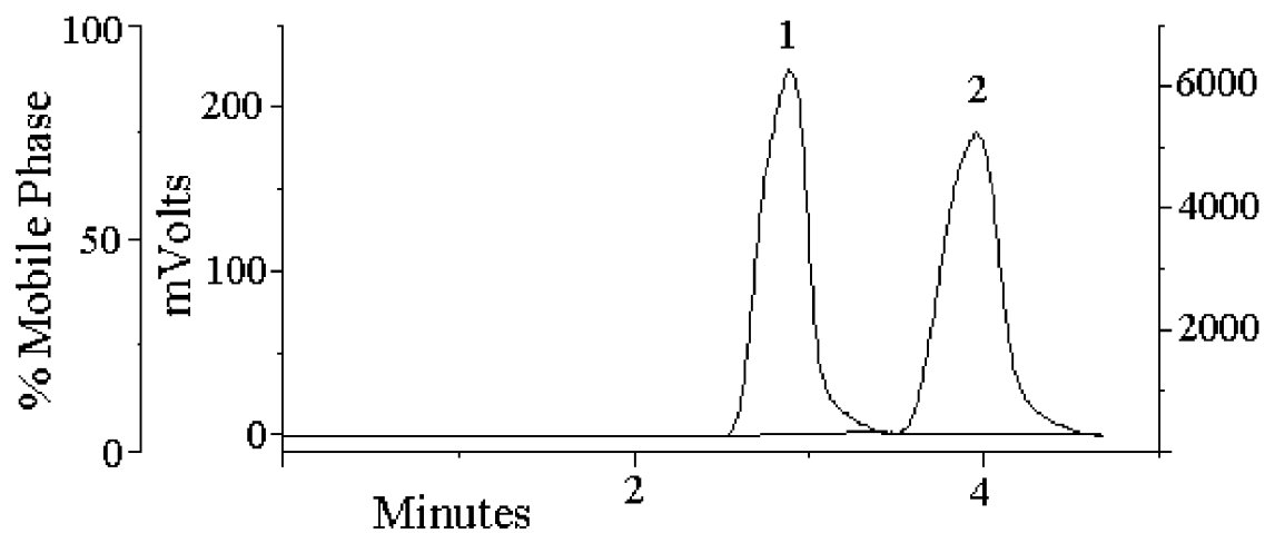
Figure 1D: SFC method, Compound 11
