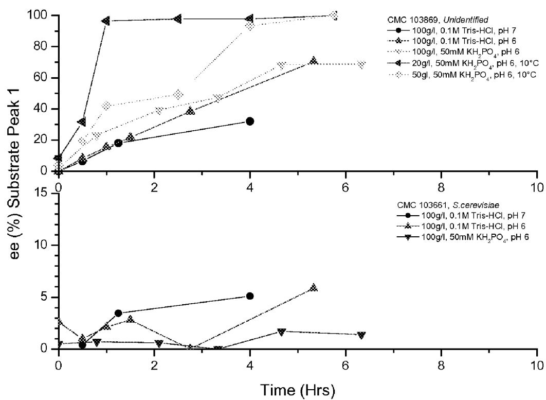
Figure 4: Microbial resolution of Compound 13
