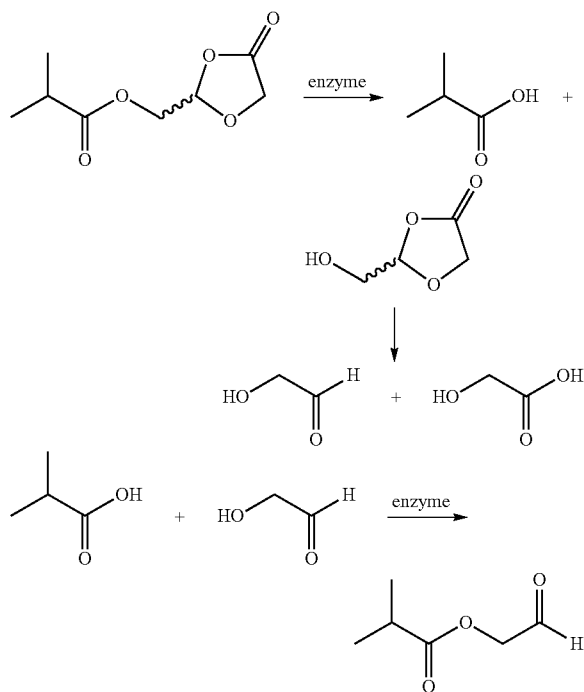
Scheme 16: Possible reaction mechanism
