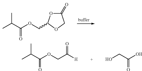
Scheme 15: Ring-opening of lactone
