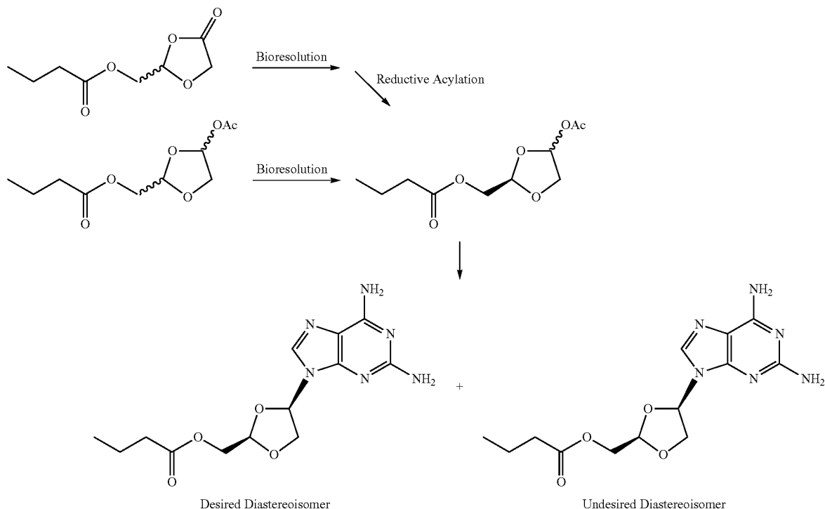
Scheme 7: Exemplary Routes to DAPD
