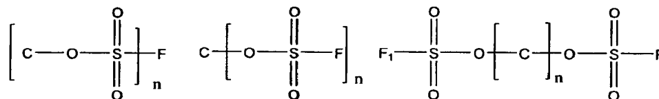
Scheme 5-1. Generic structures of environmentally friendly Nonionic PAGs.
