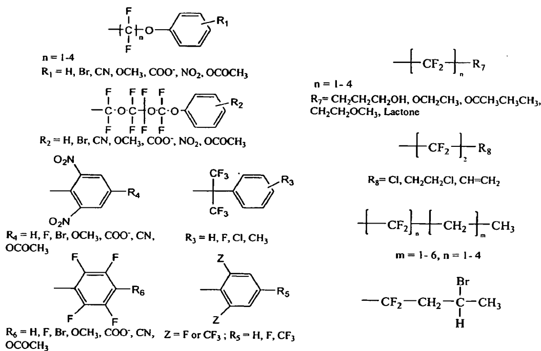
Scheme 5-3. Fluoroorganic (F) groups and their derivatives for nonionic PAGs
