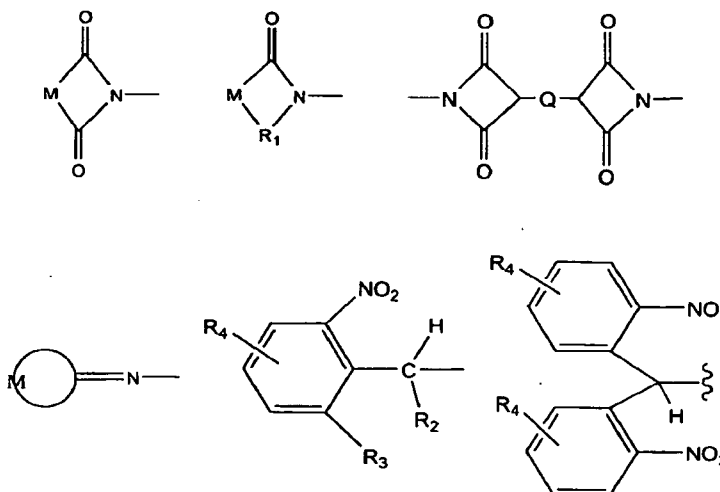
Scheme 5-2. Photosensitive chromophores (C) and their derivatives
