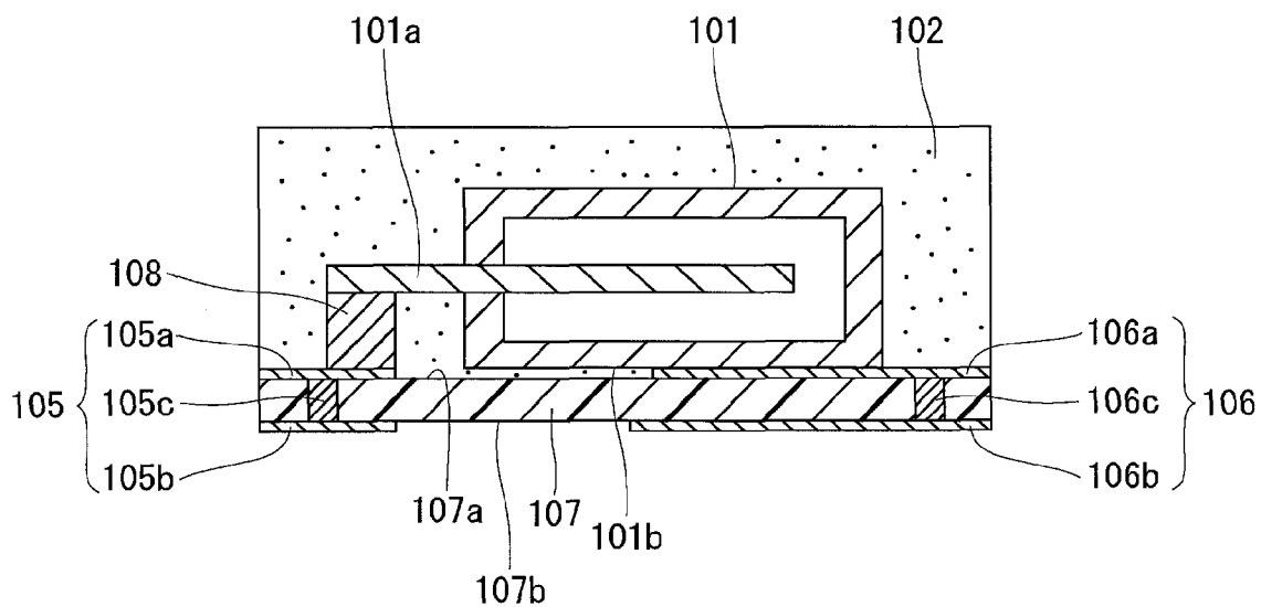
FIG. 13 PRIOR ART
