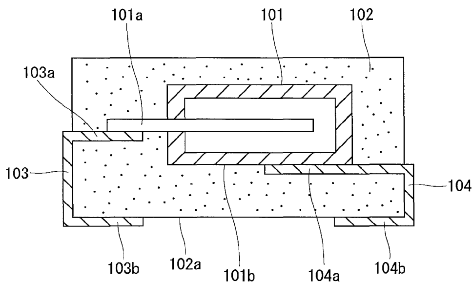
FIG. 12 PRIOR ART
