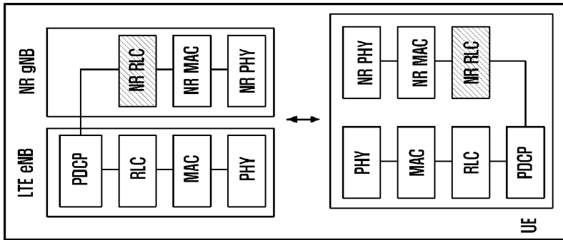
3C type LTE-NR Interworking : 1f-02 LTE (MeNB), NR (SeNB)
