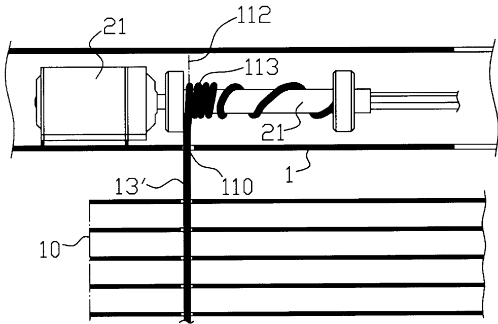
PRIOR ART FIG. 10
