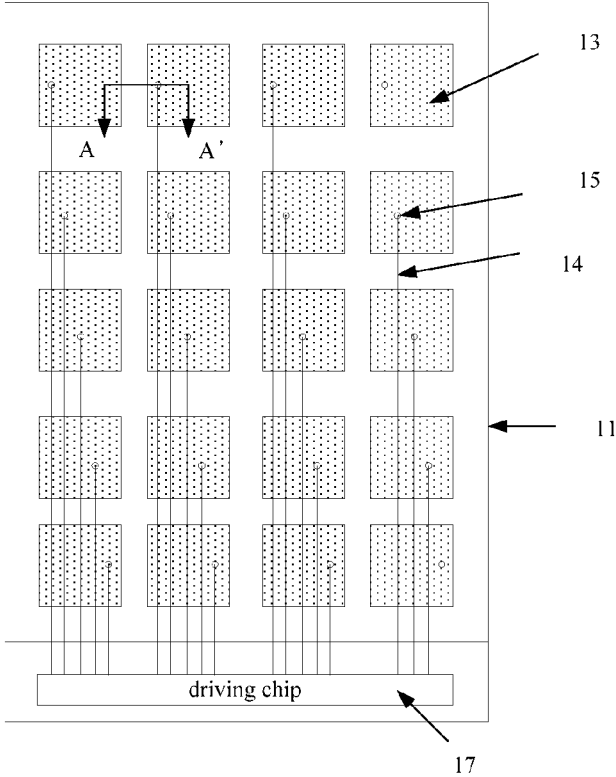
Figure 1 (PRIOR ART)
