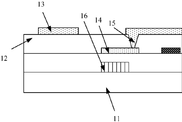
Figure 2 (PRIOR ART)
