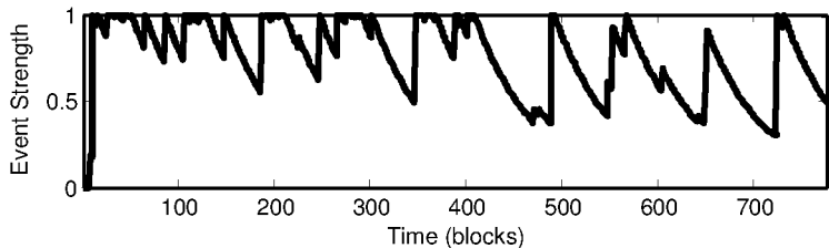
FIG. 10d d) Event control signal
