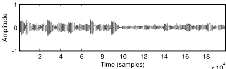
FIG. 10c c) Signal modified with DRC gain
