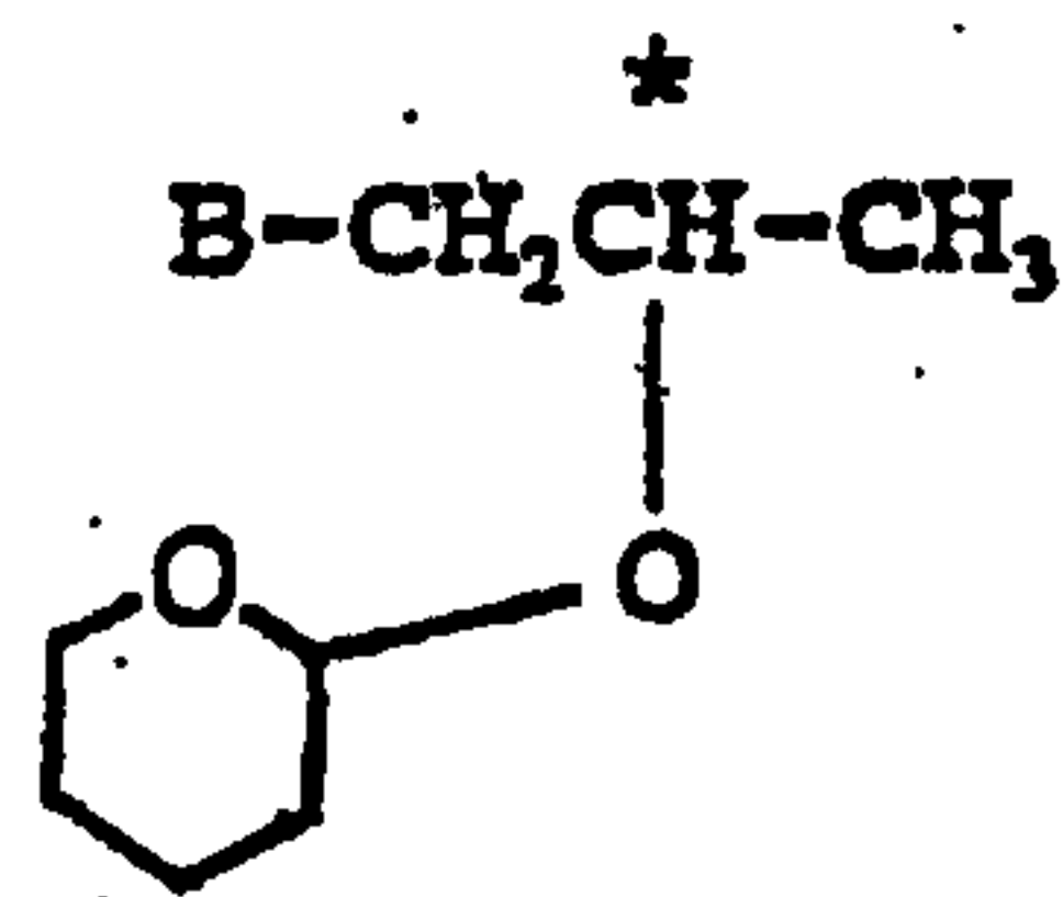
(II) A
