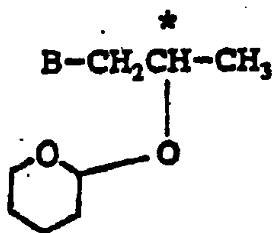
(II) A
