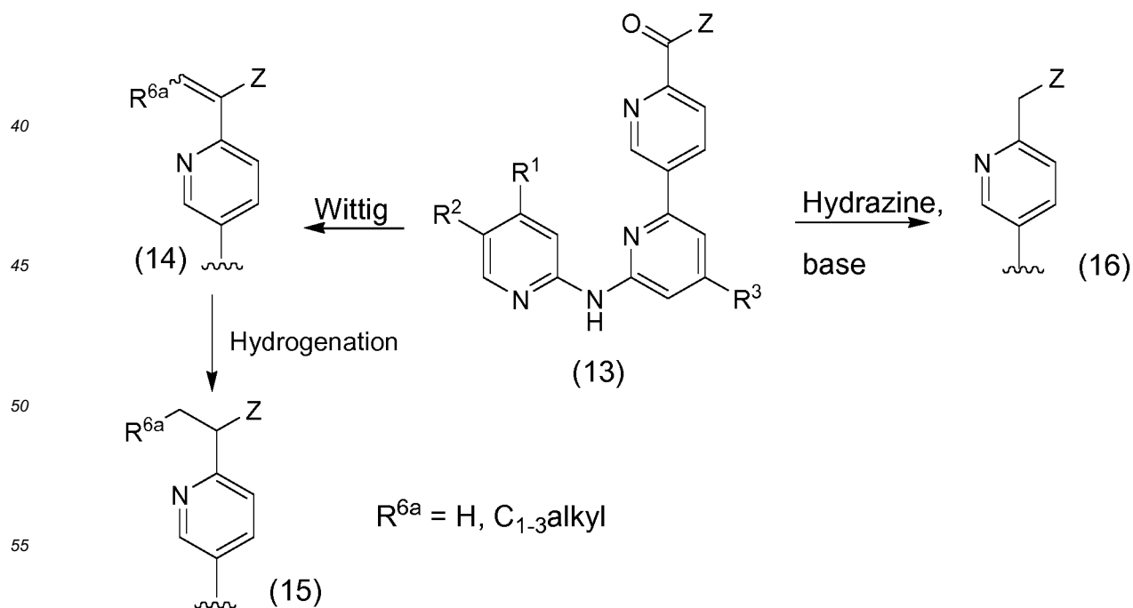
SCHEME 3
