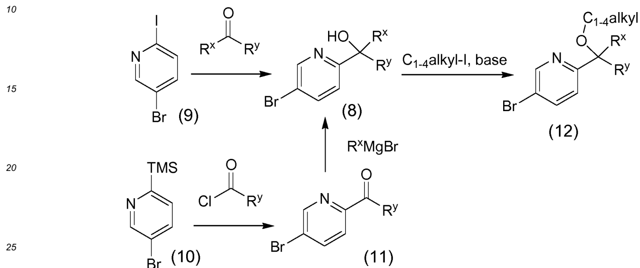
SCHEME 2
