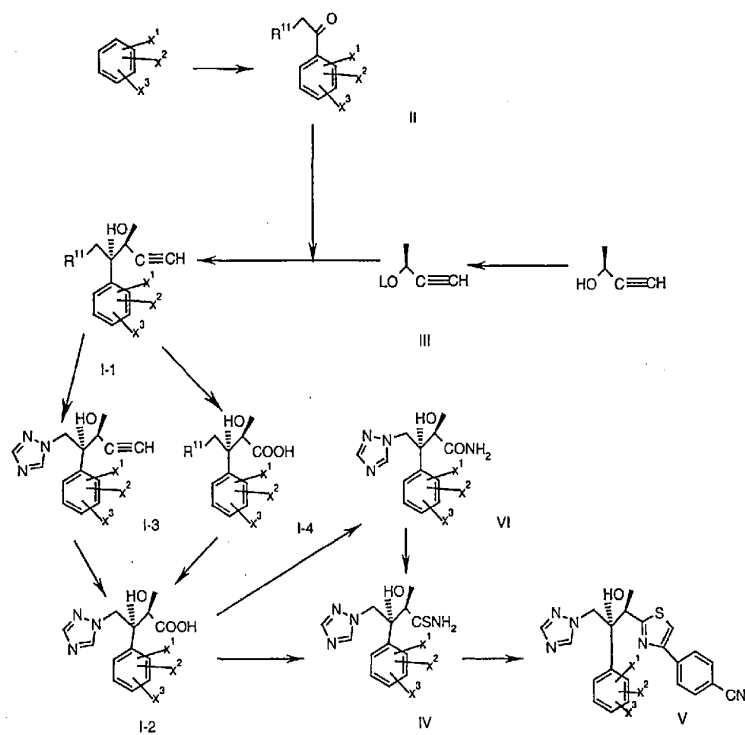
Scheme 1
