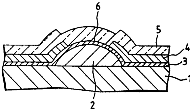
FIG. 20 PRIOR ART
