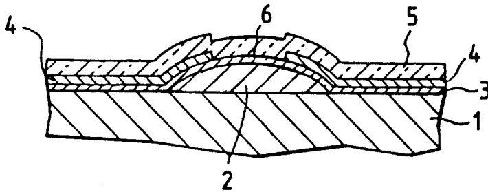
FIG. 18 PRIOR ART
