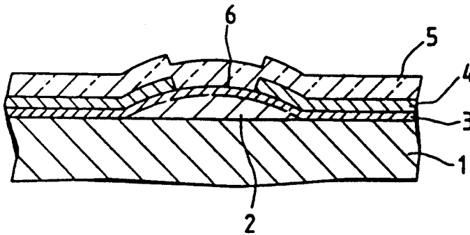
FIG. 19 PRIOR ART
