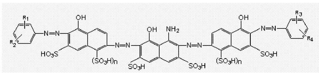
General formula (7)
