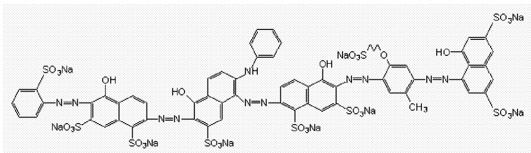
General formula (8)
