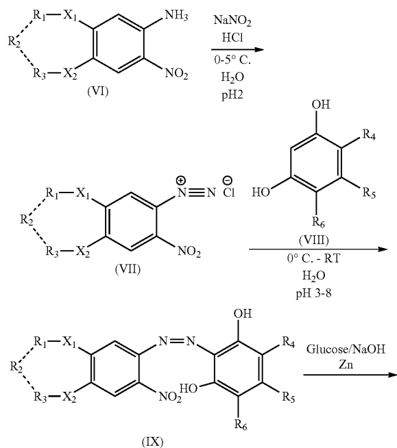
Scheme 1. Generic 2,6-dihydroxyphenyl-2H-benzotriazole synthesis
