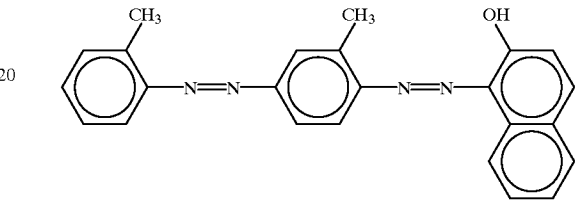
Formula (IV)
