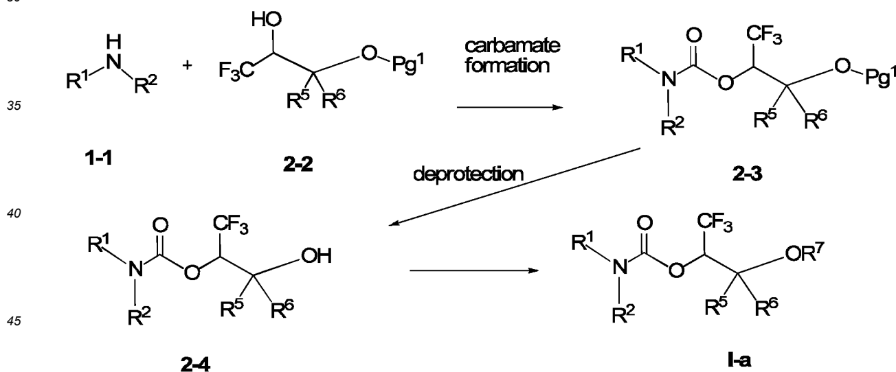
Scheme 2
