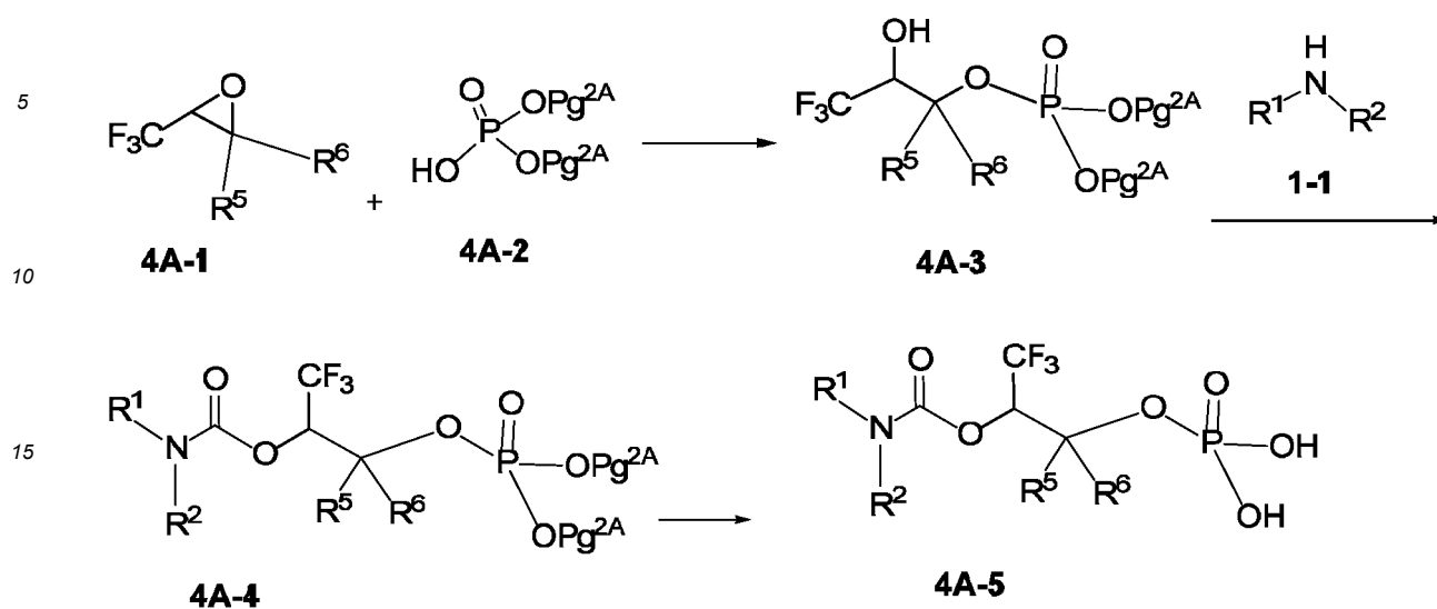
Scheme 4A
