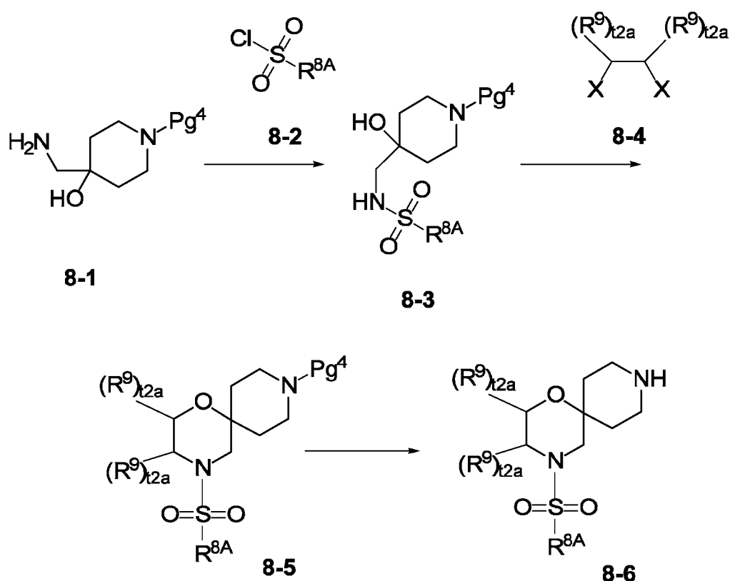
Scheme 8
