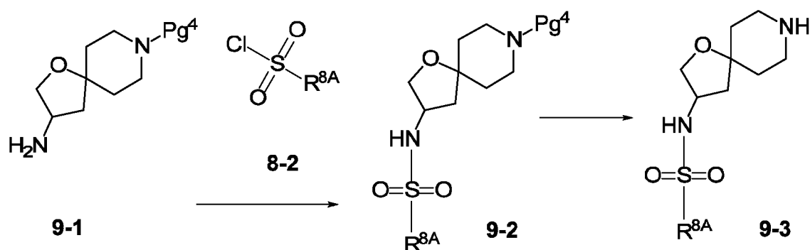
Scheme 9
