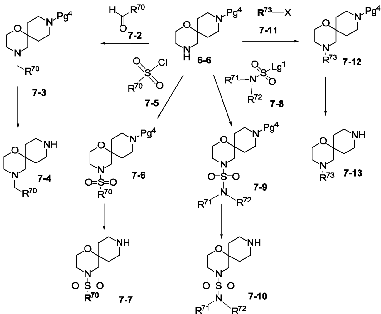
Scheme 7
