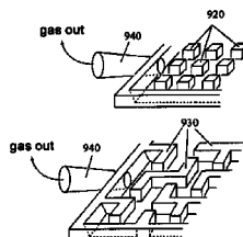
Example: Microfluidic Plumbing with In-Built Spacer (Gas only)
