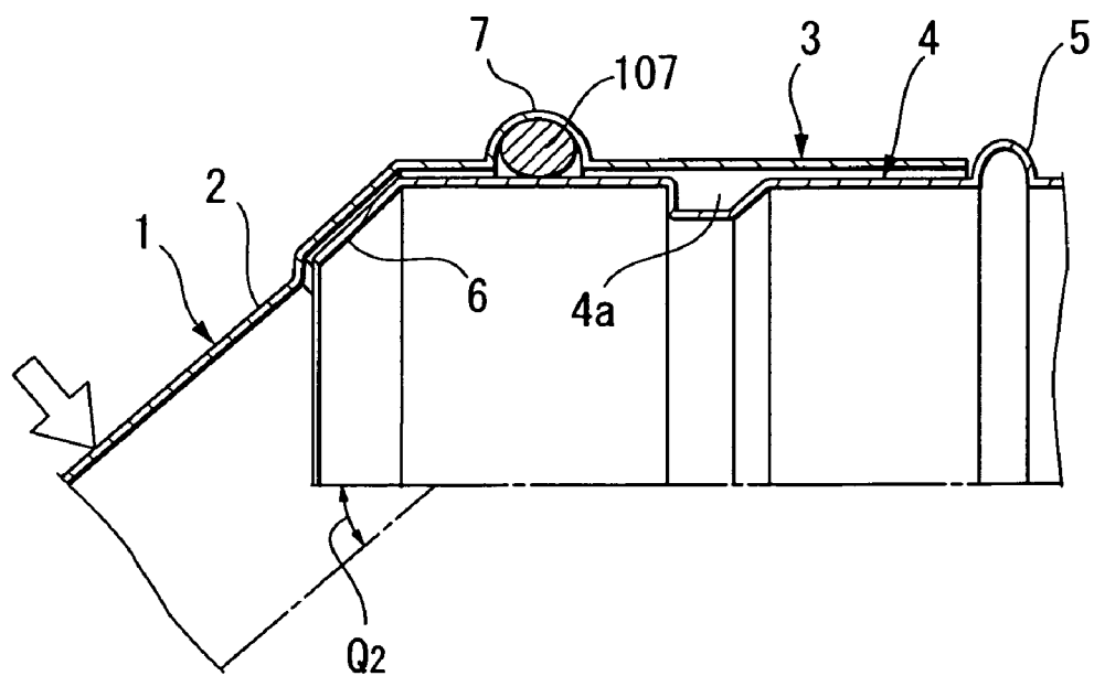
FIG. 6 PRIOR ART
