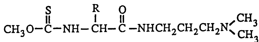
Derivatized N-Terminal Amino Acid
