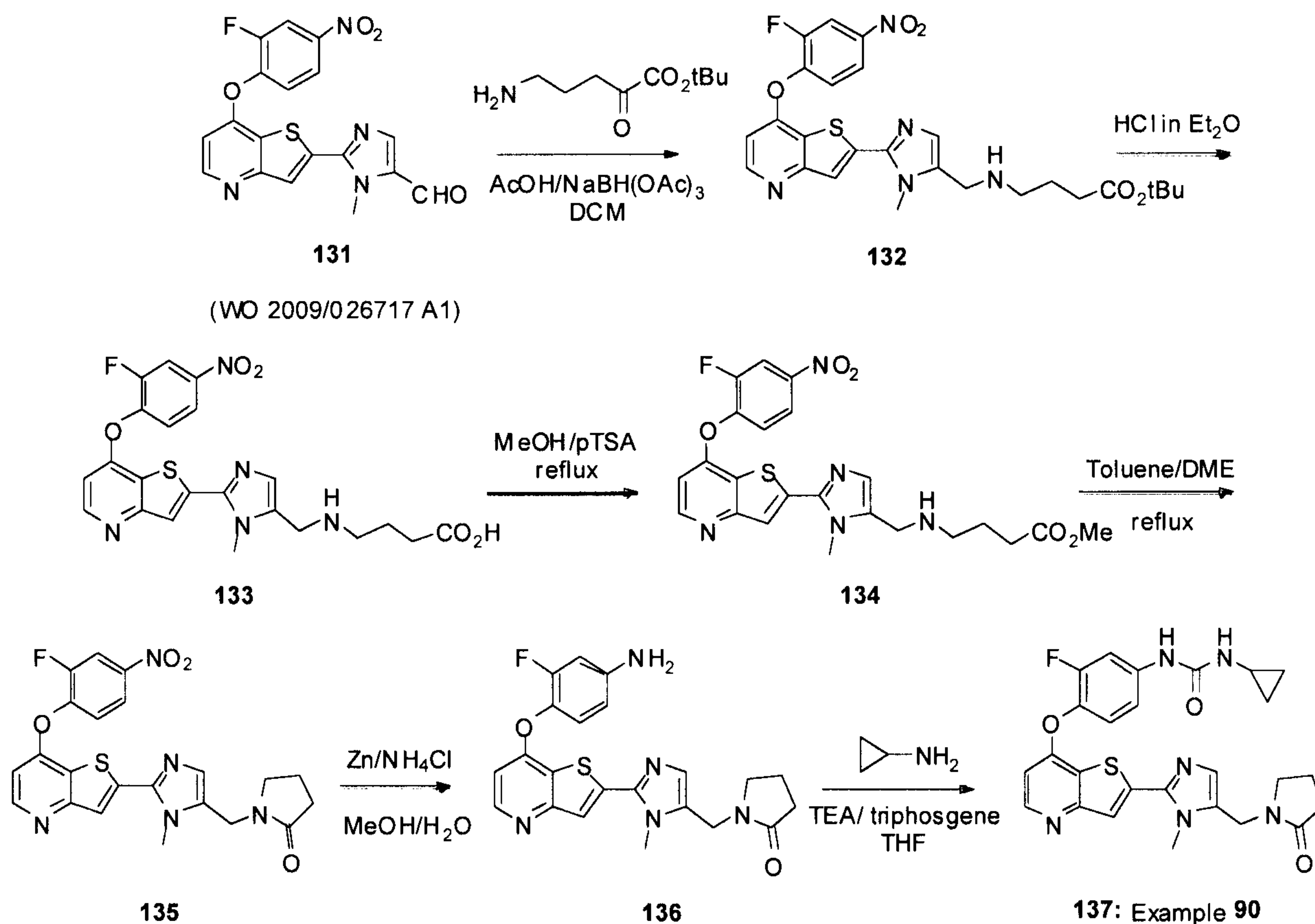
Scheme 33
