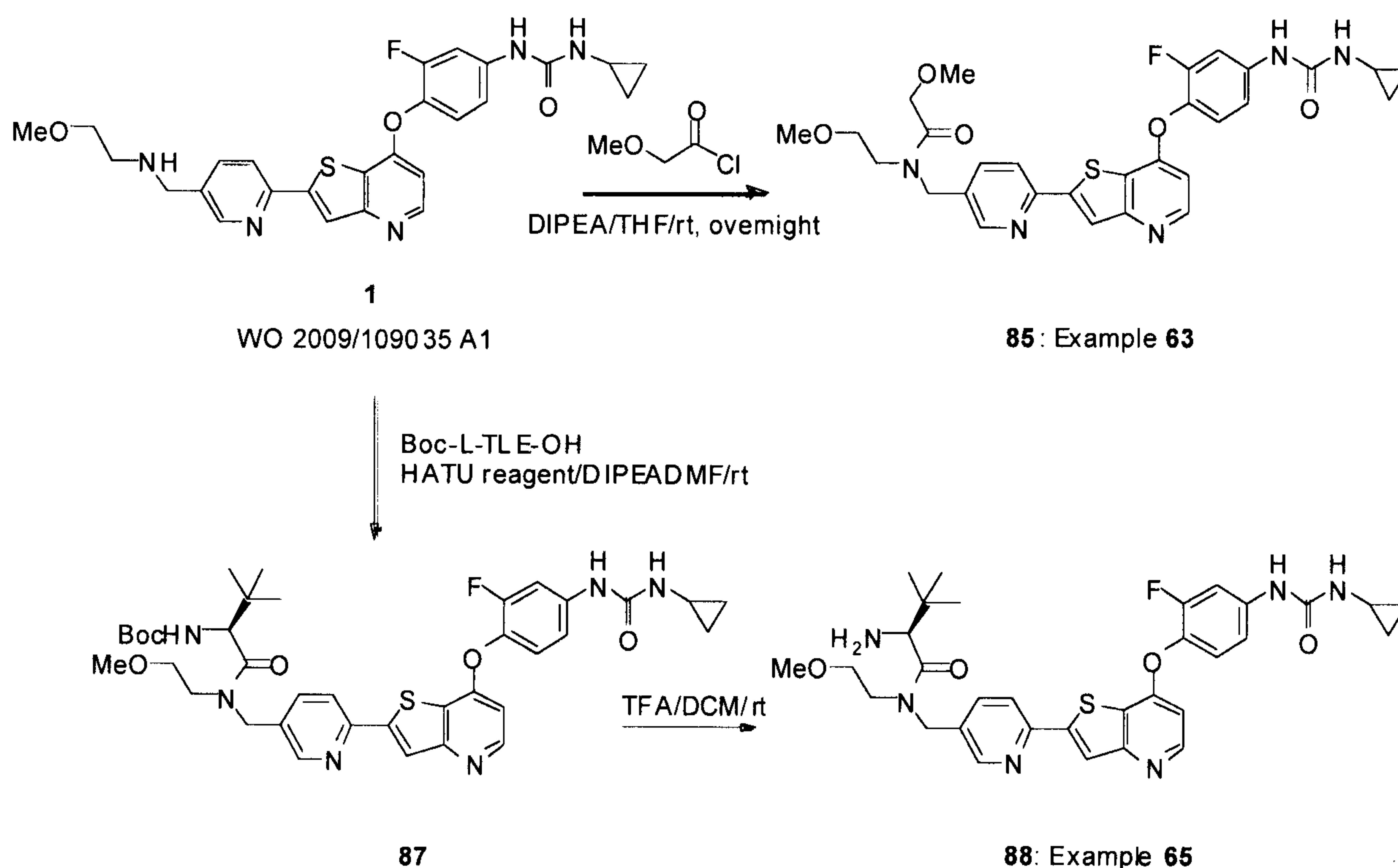
Scheme 23
