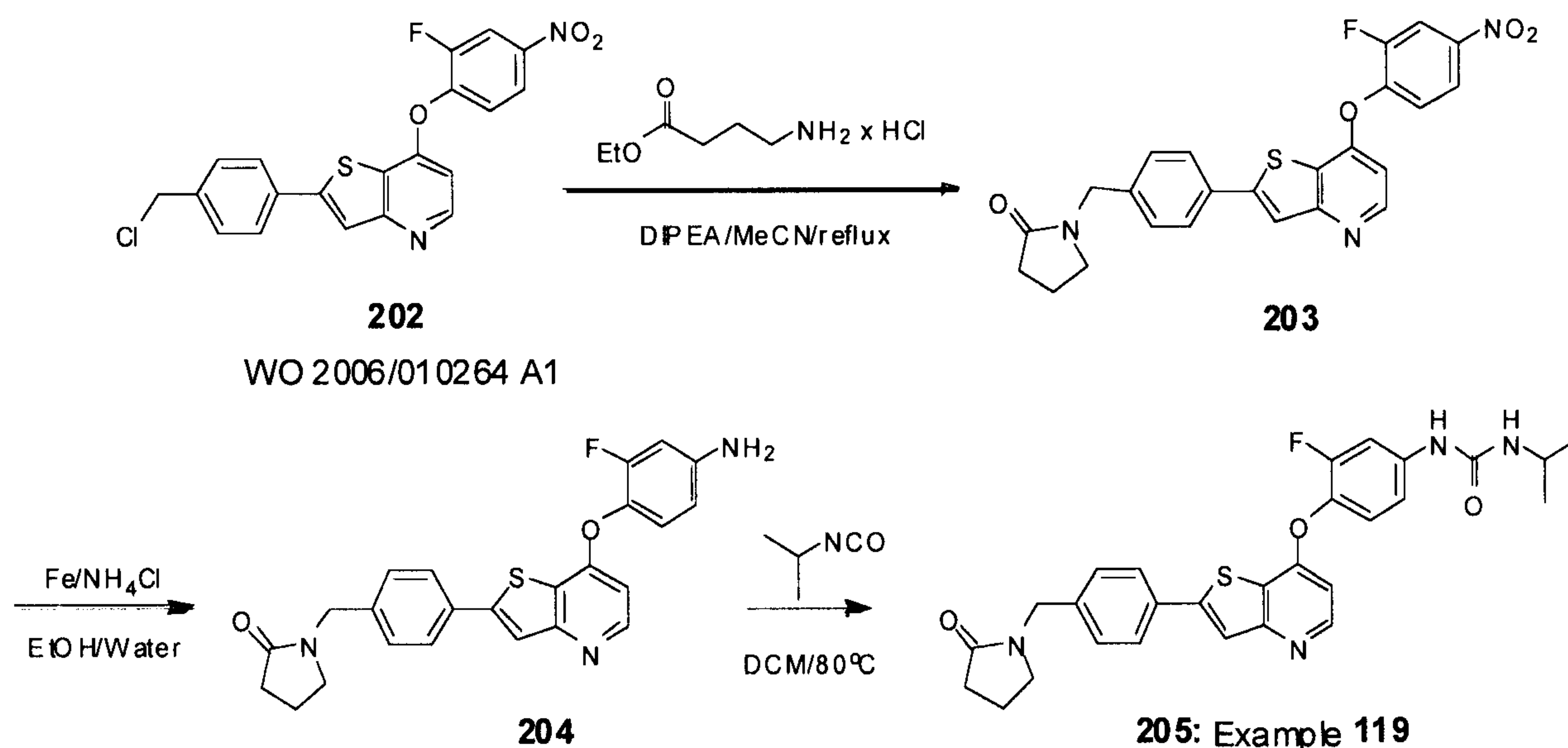
Scheme 49
