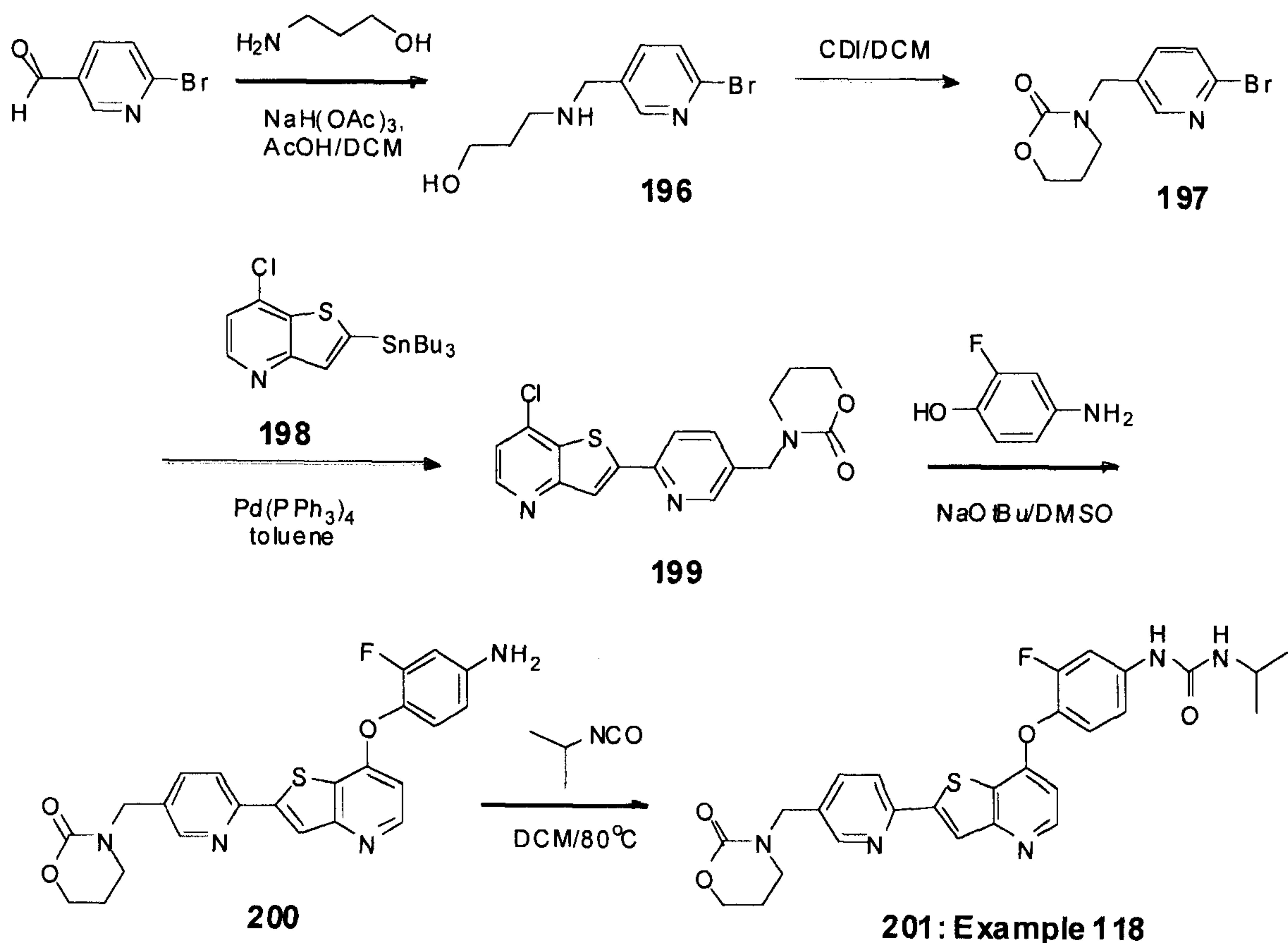
Scheme 48
