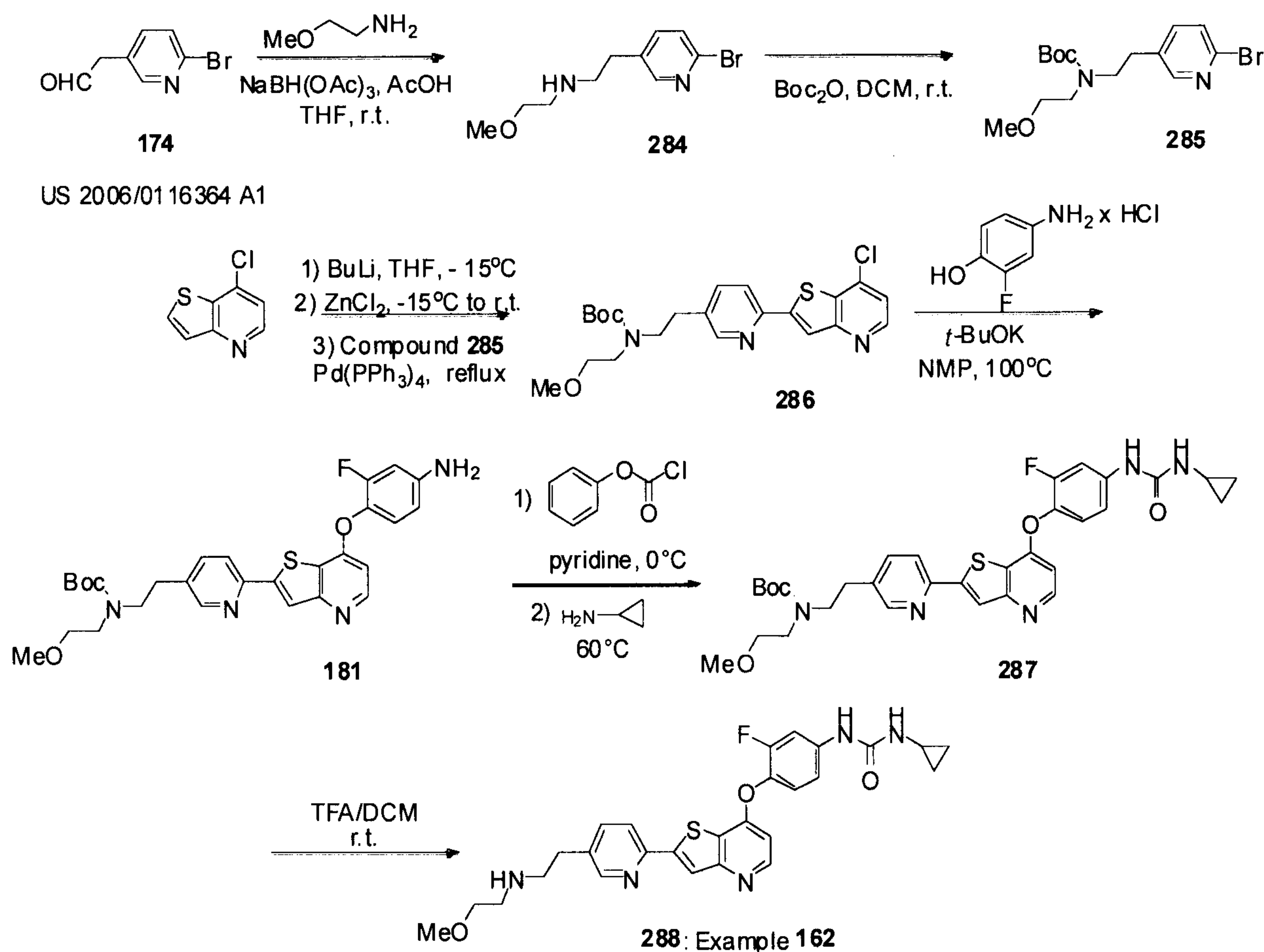
Scheme 64
