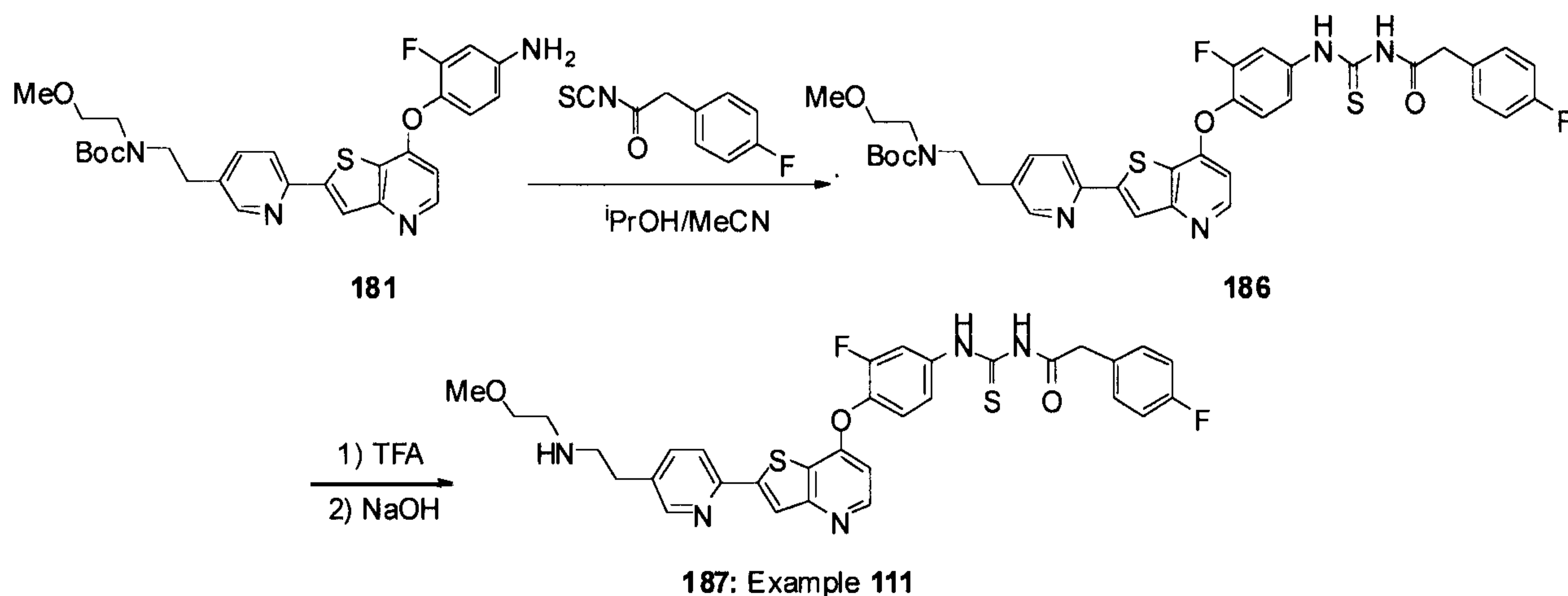
Scheme 46
