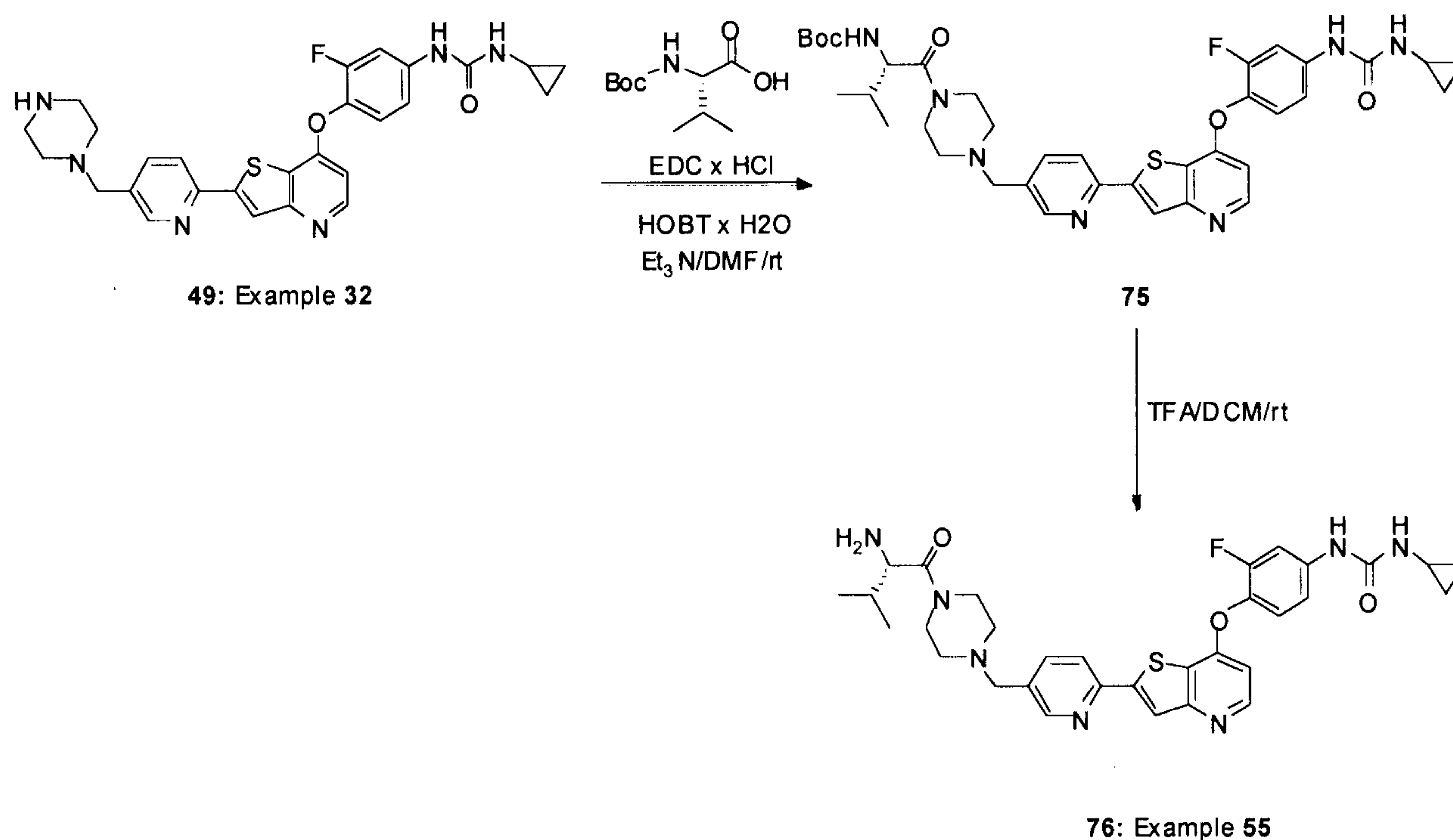
Scheme 20
