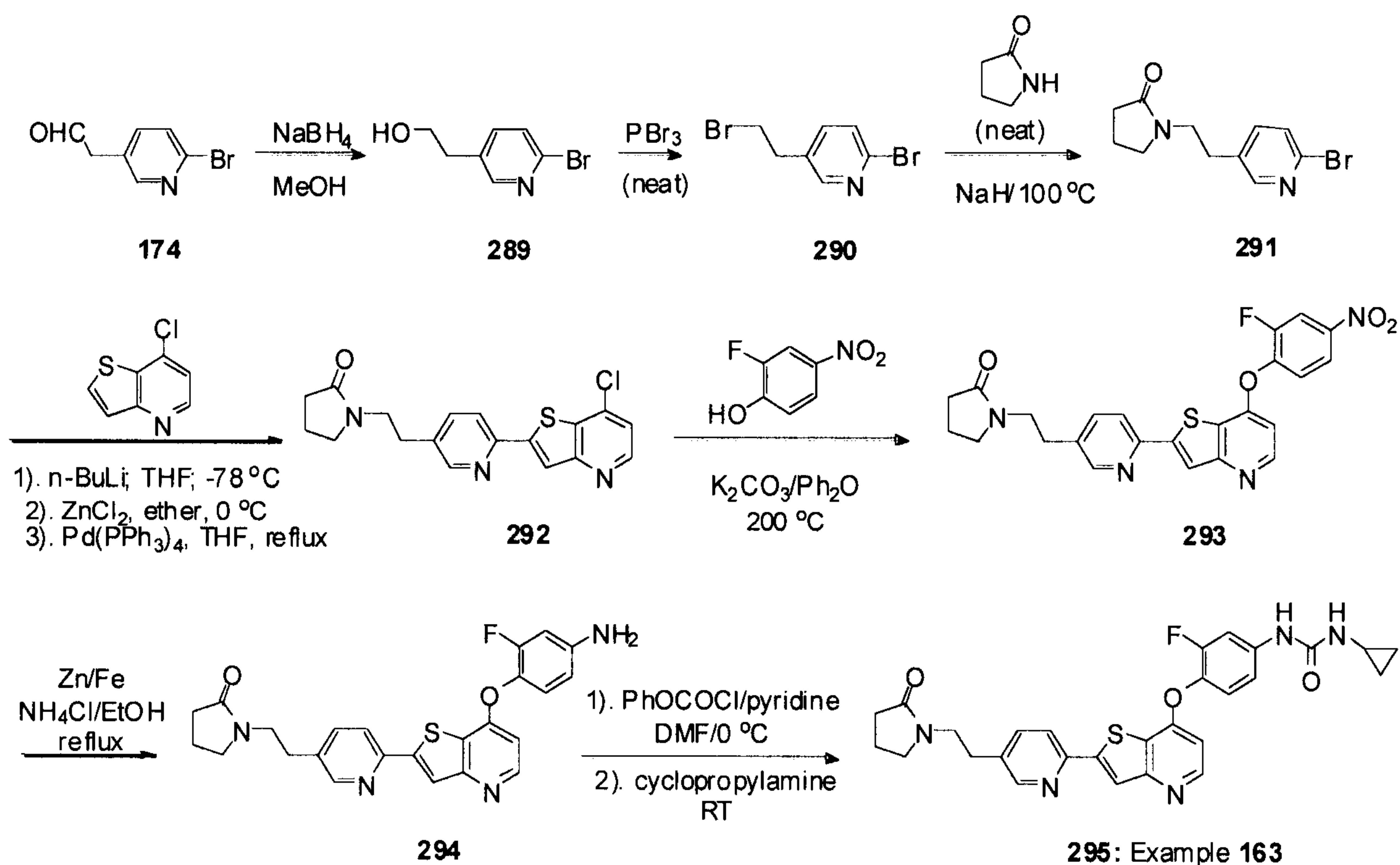
Scheme 65
