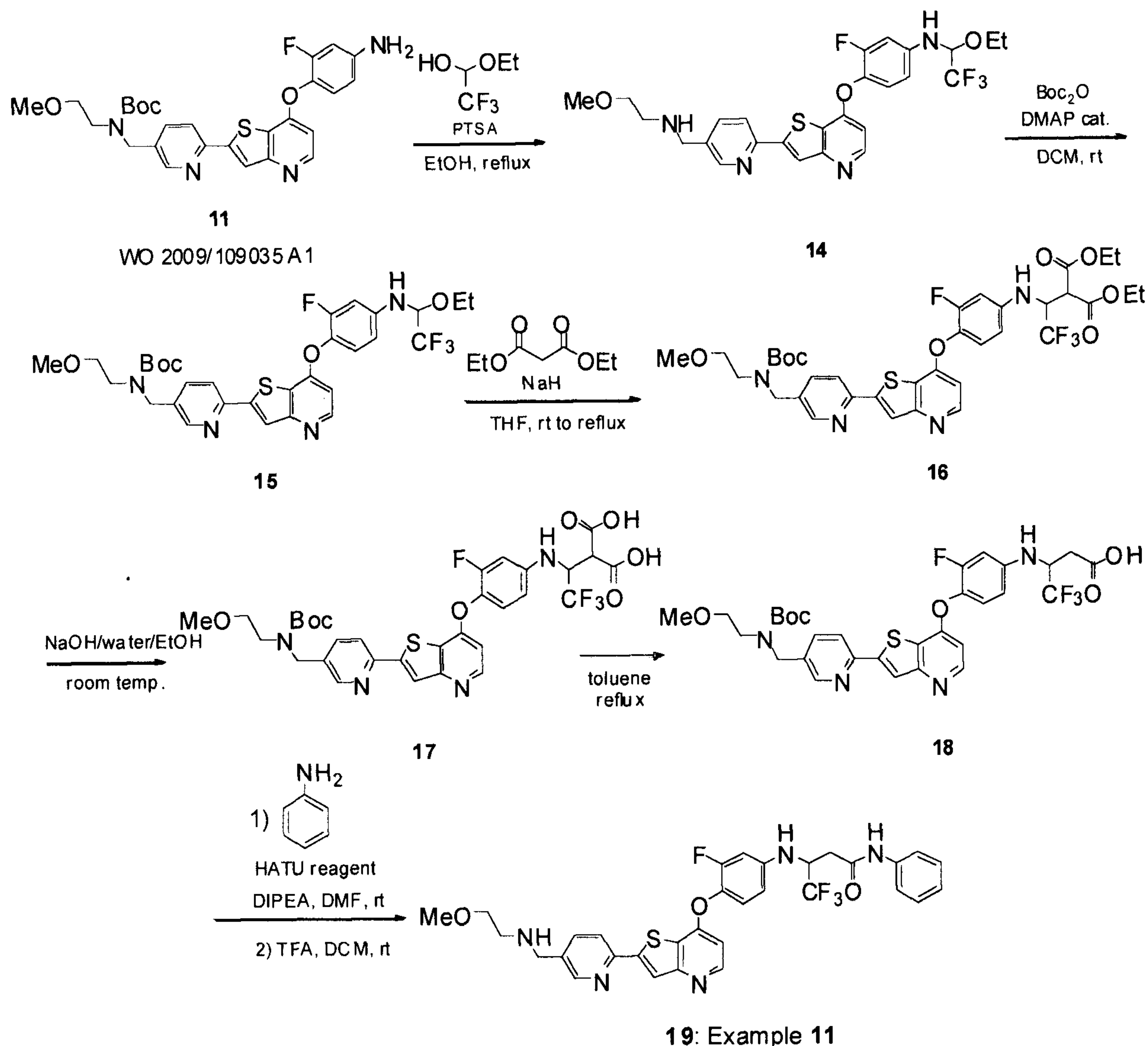
Scheme 10
