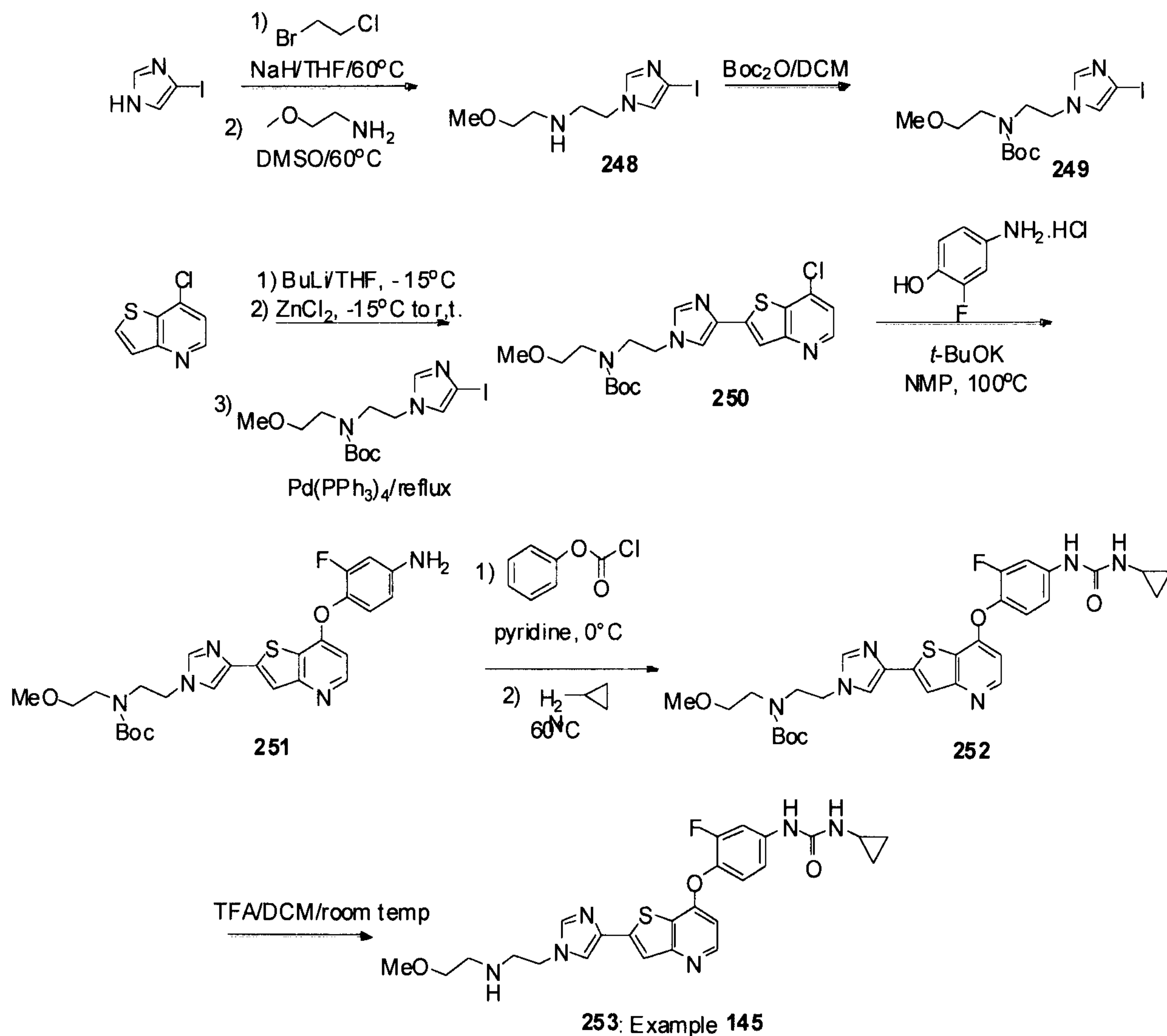
Scheme 57
