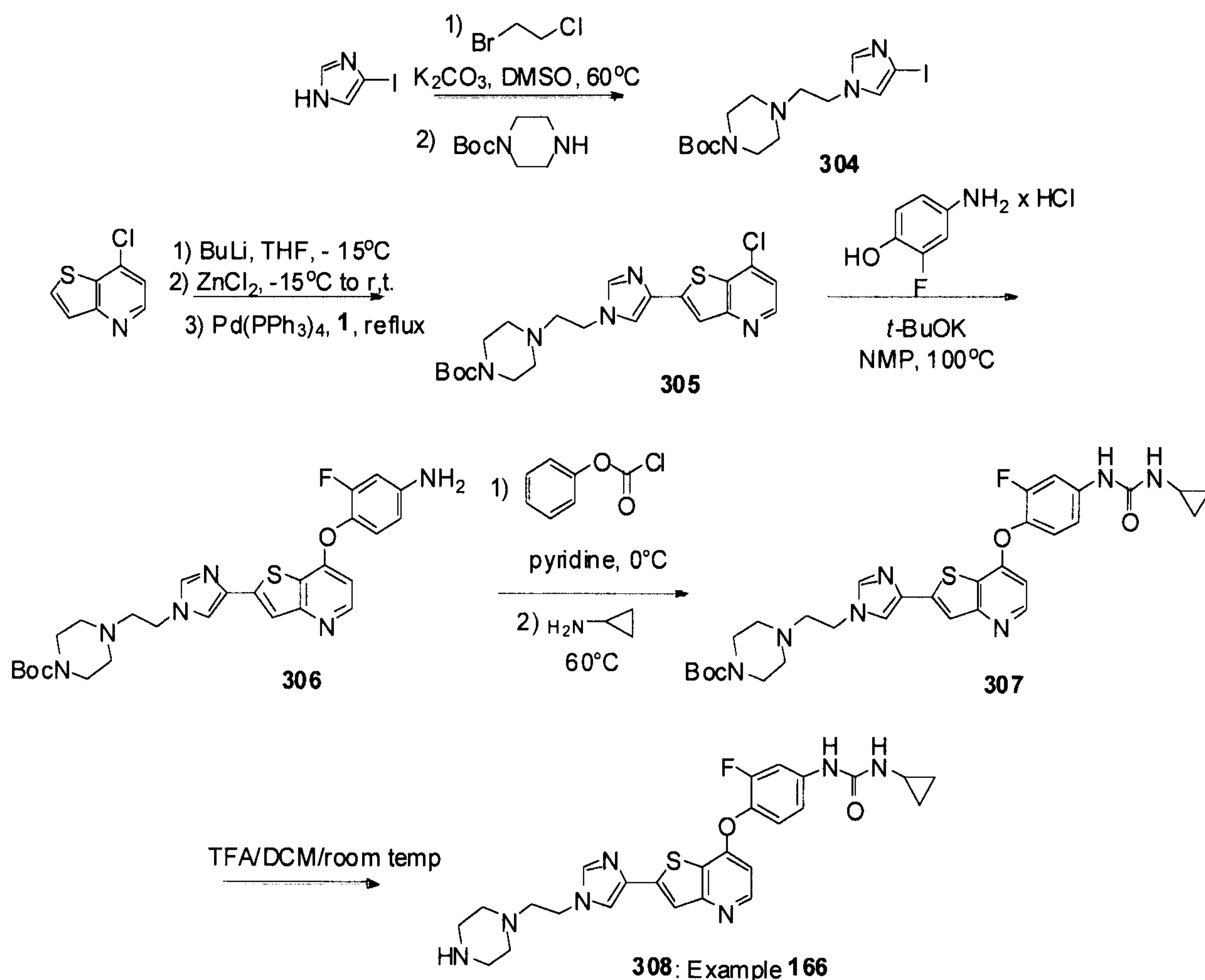
Scheme 68
