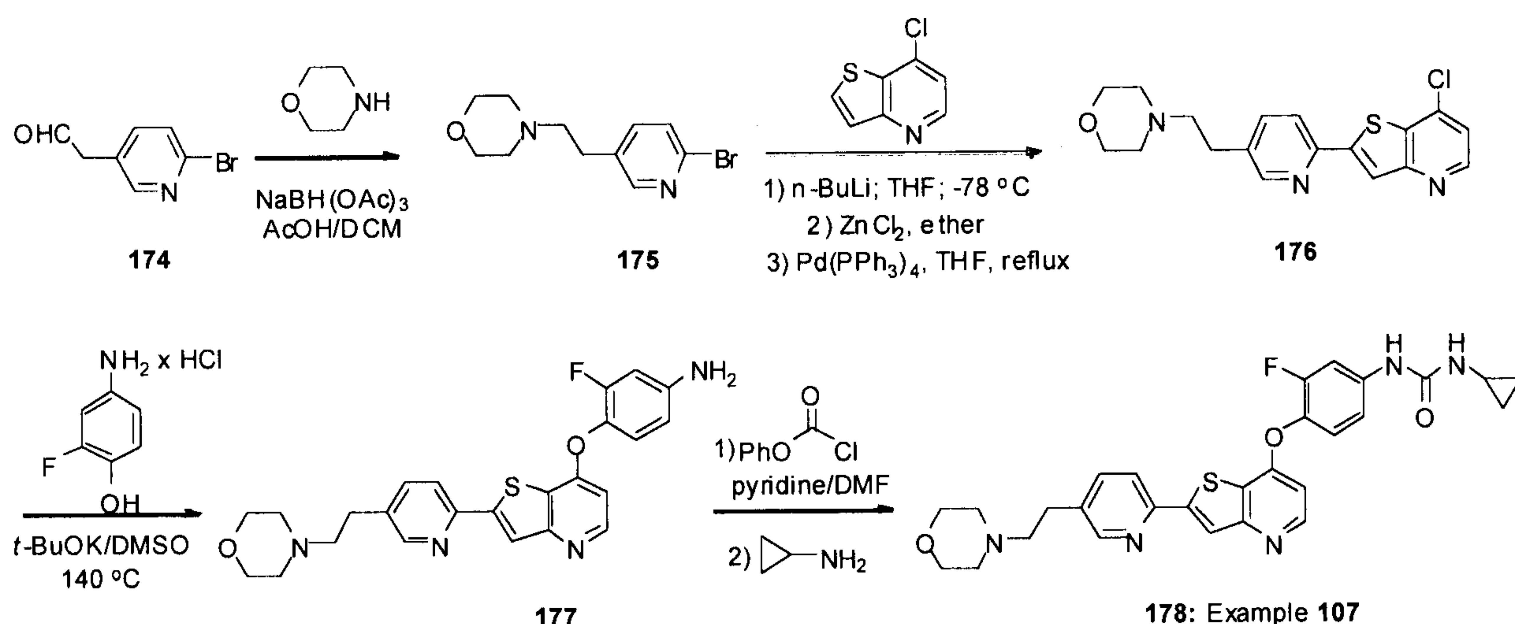
Scheme 42
