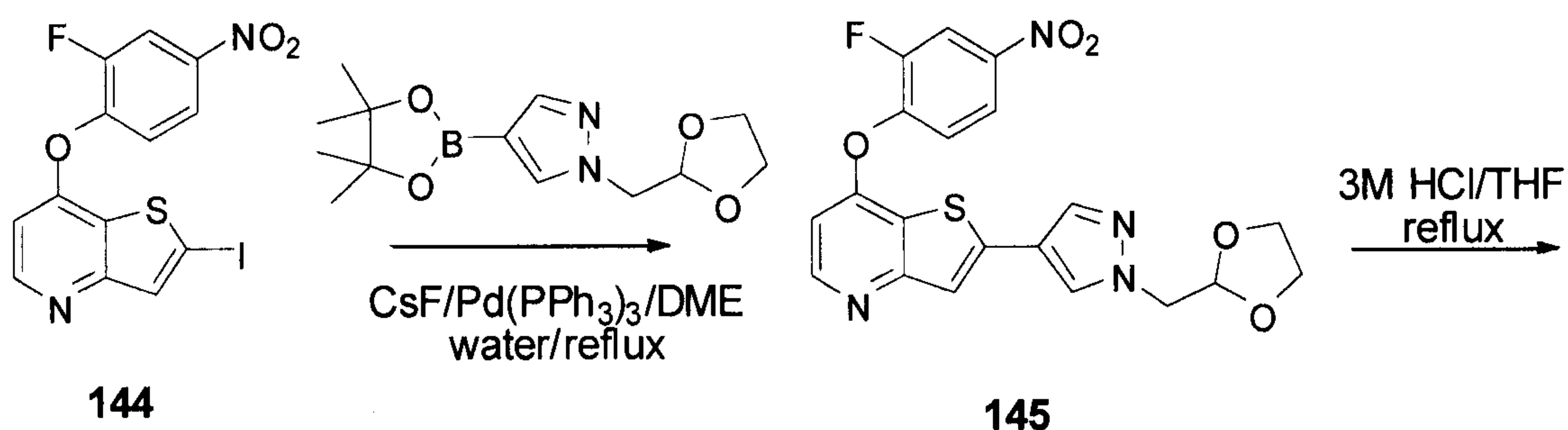
Scheme 37
