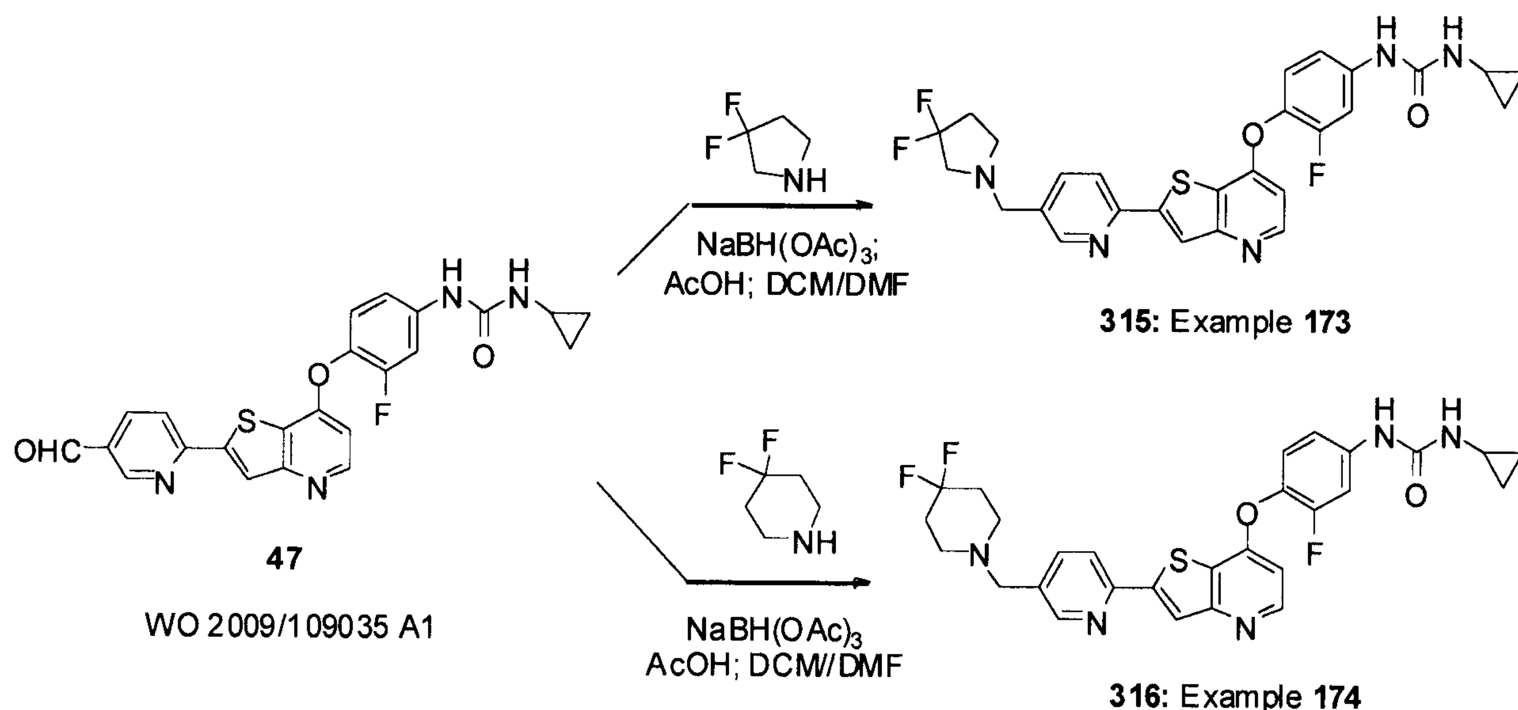
Scheme 69
