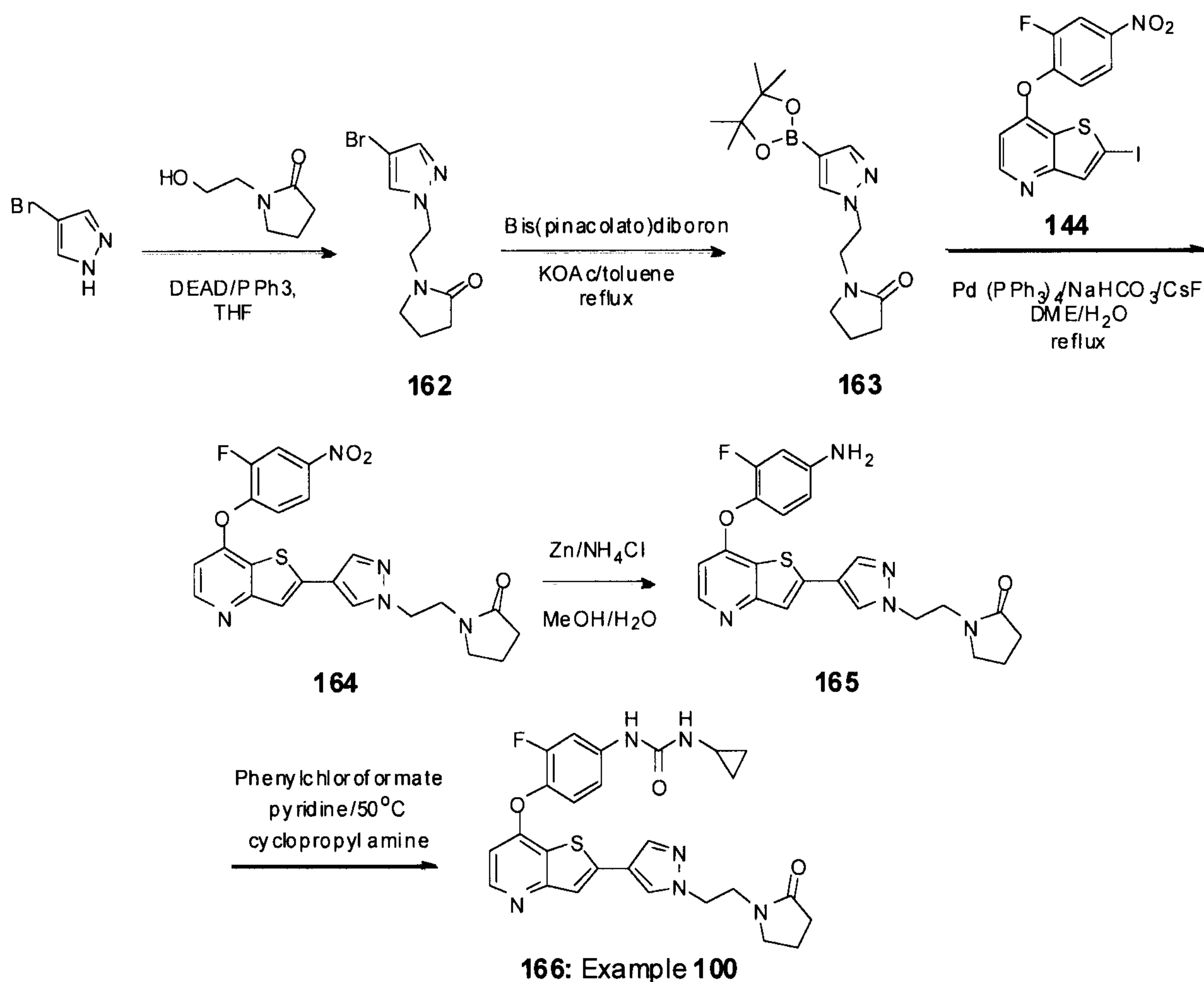
Scheme 40
