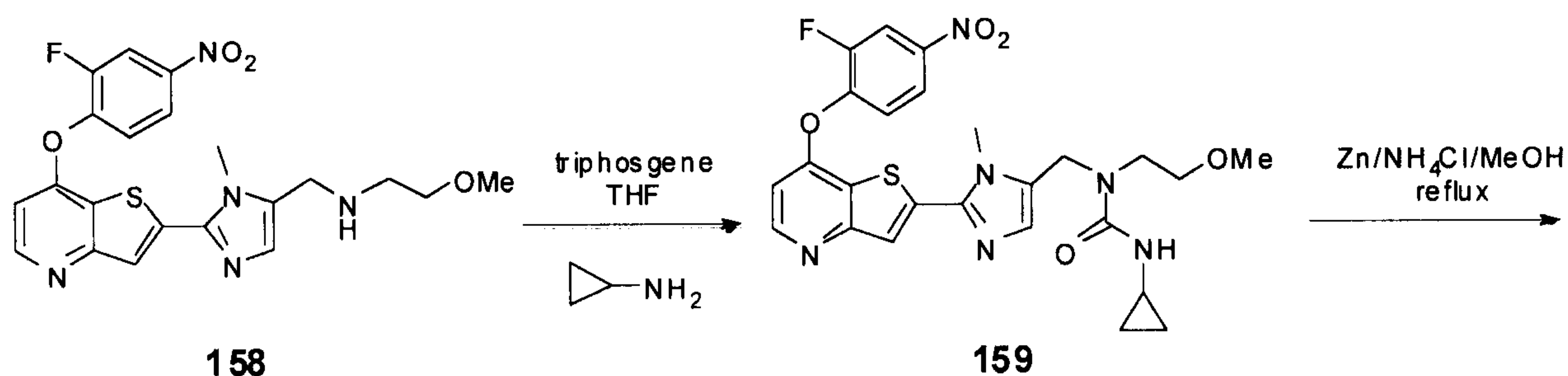
Scheme 39
