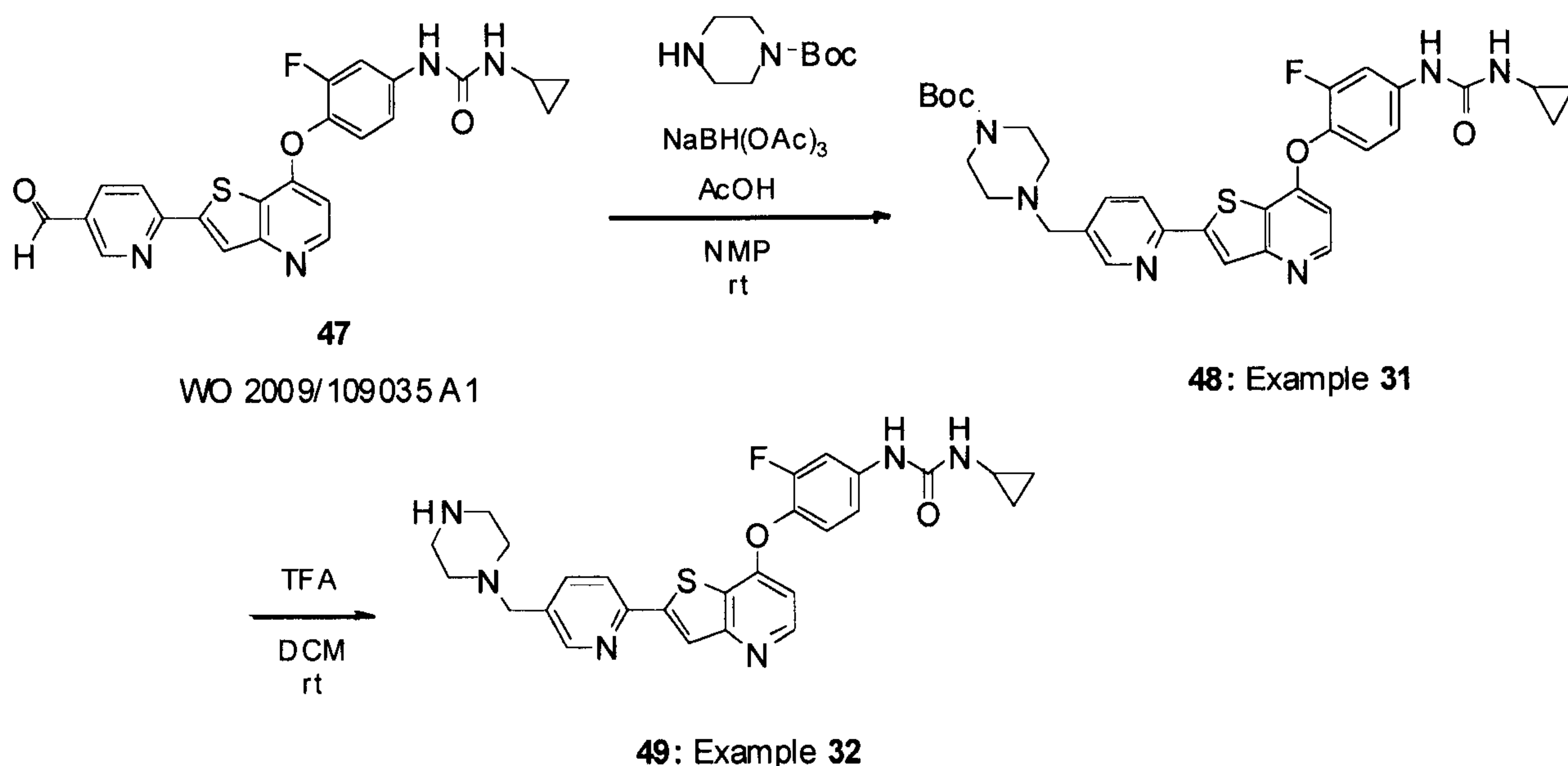
Scheme 15
