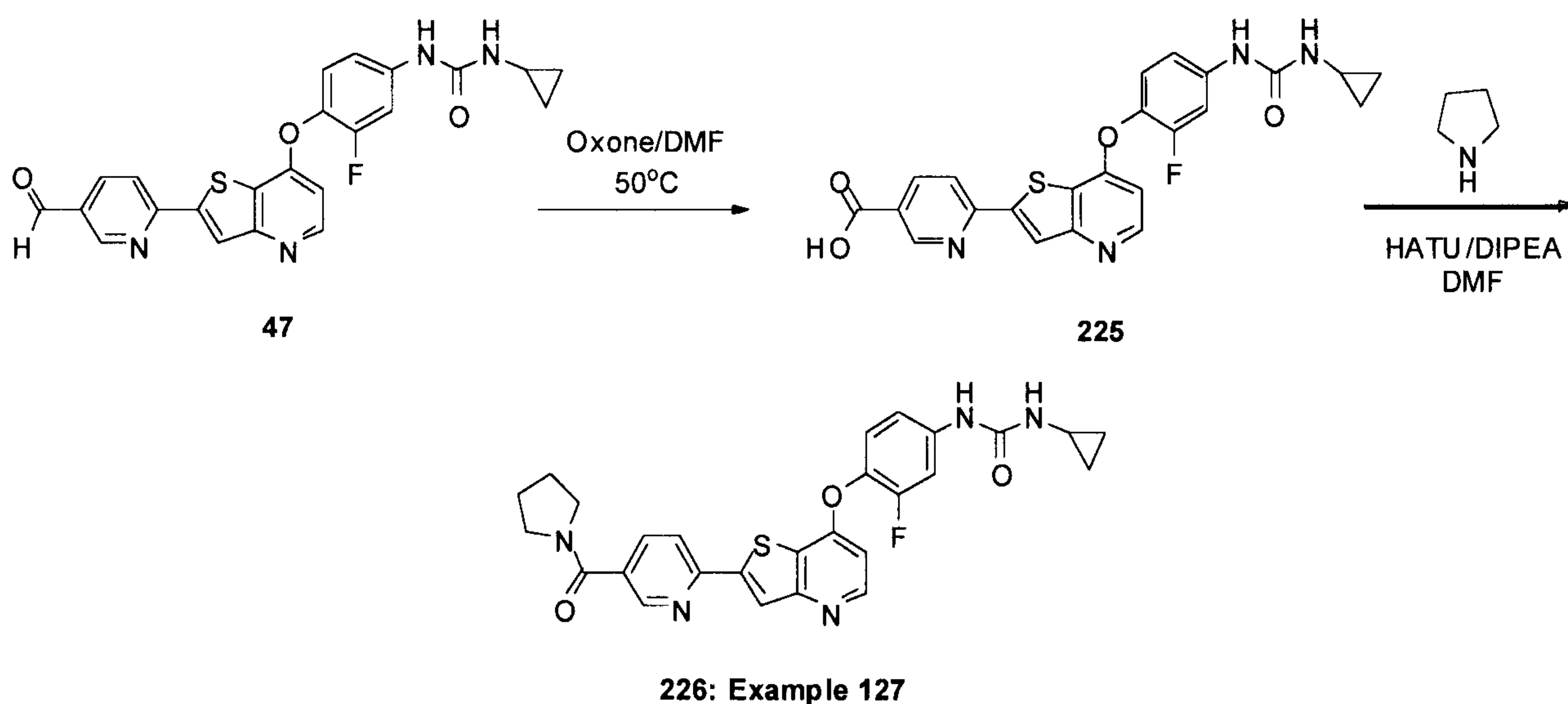
Scheme 54
