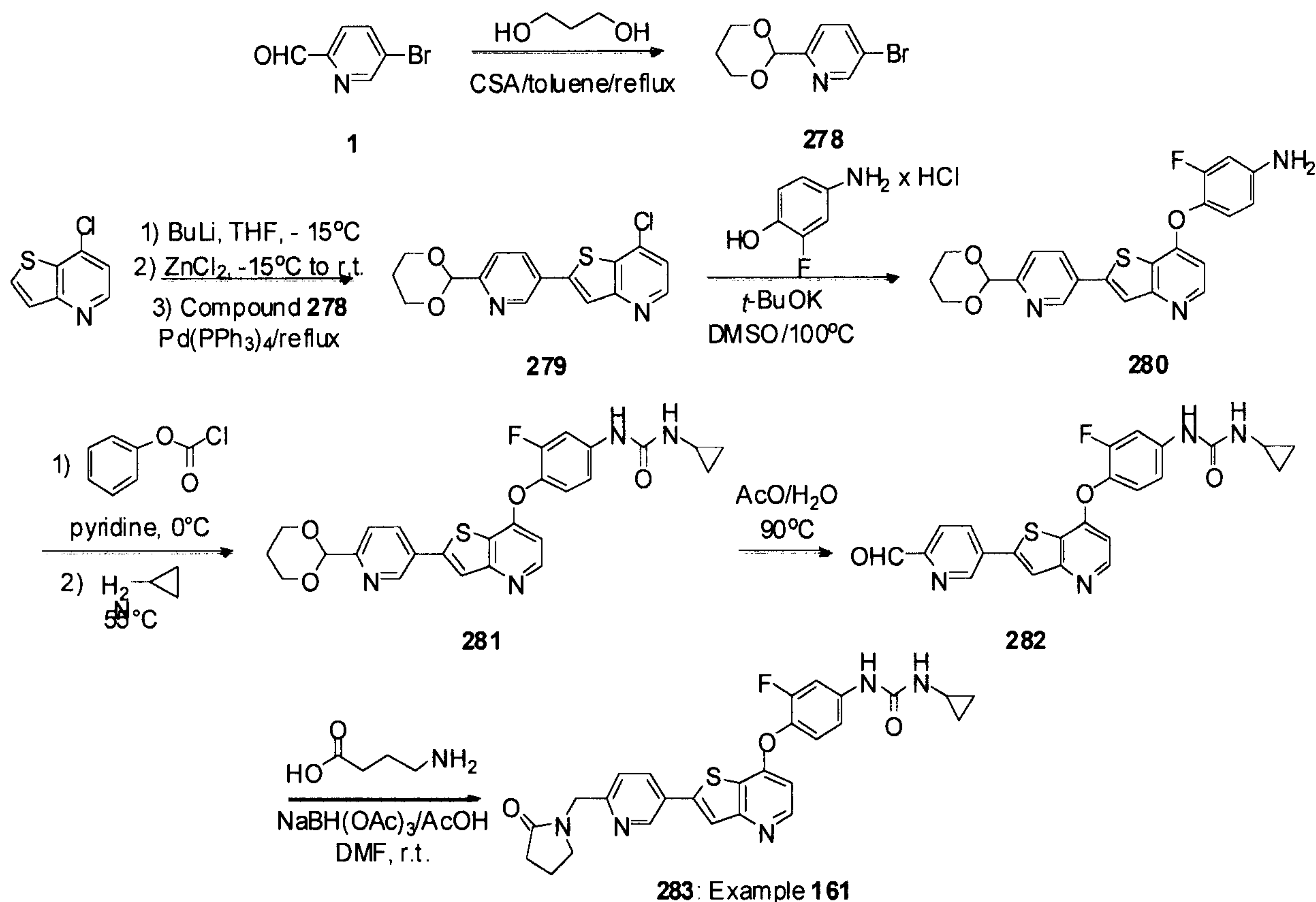
Scheme 63
