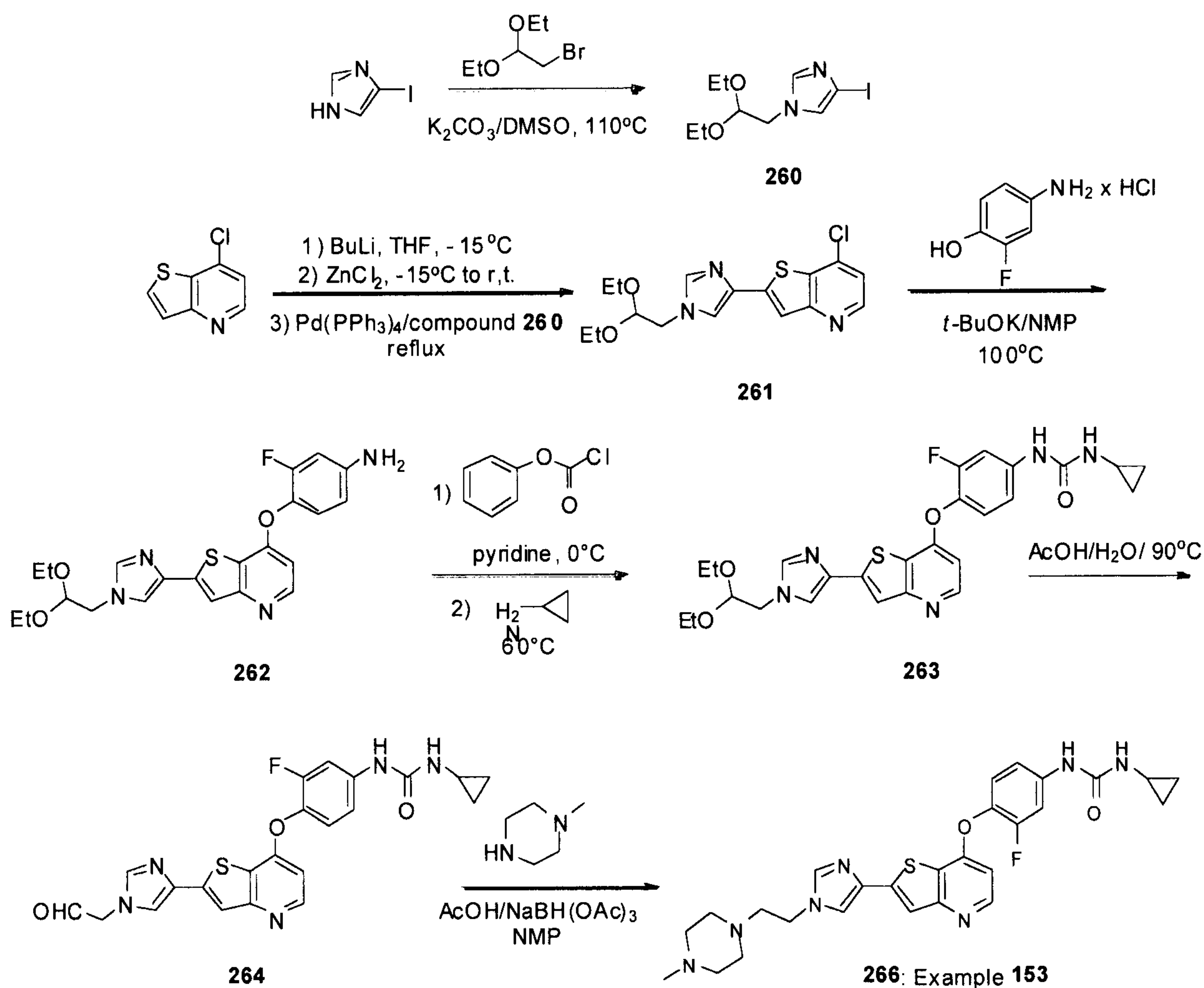
Scheme 58
