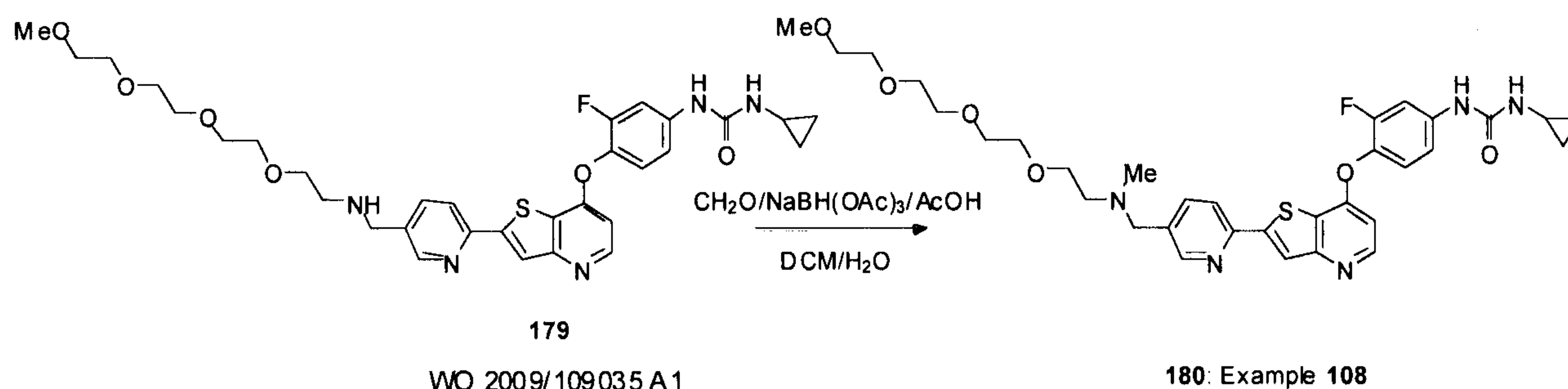
Scheme 43
