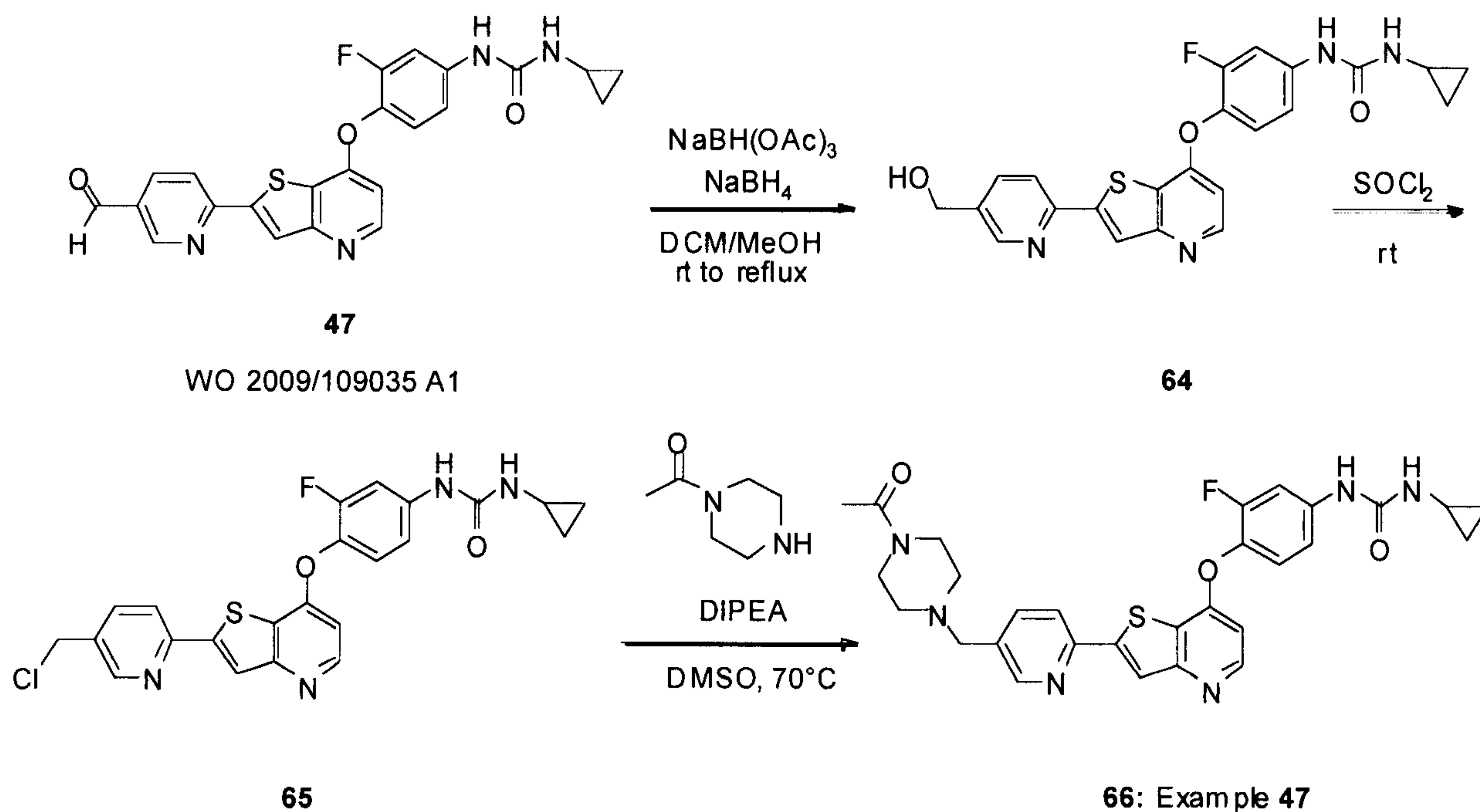
Scheme 17
