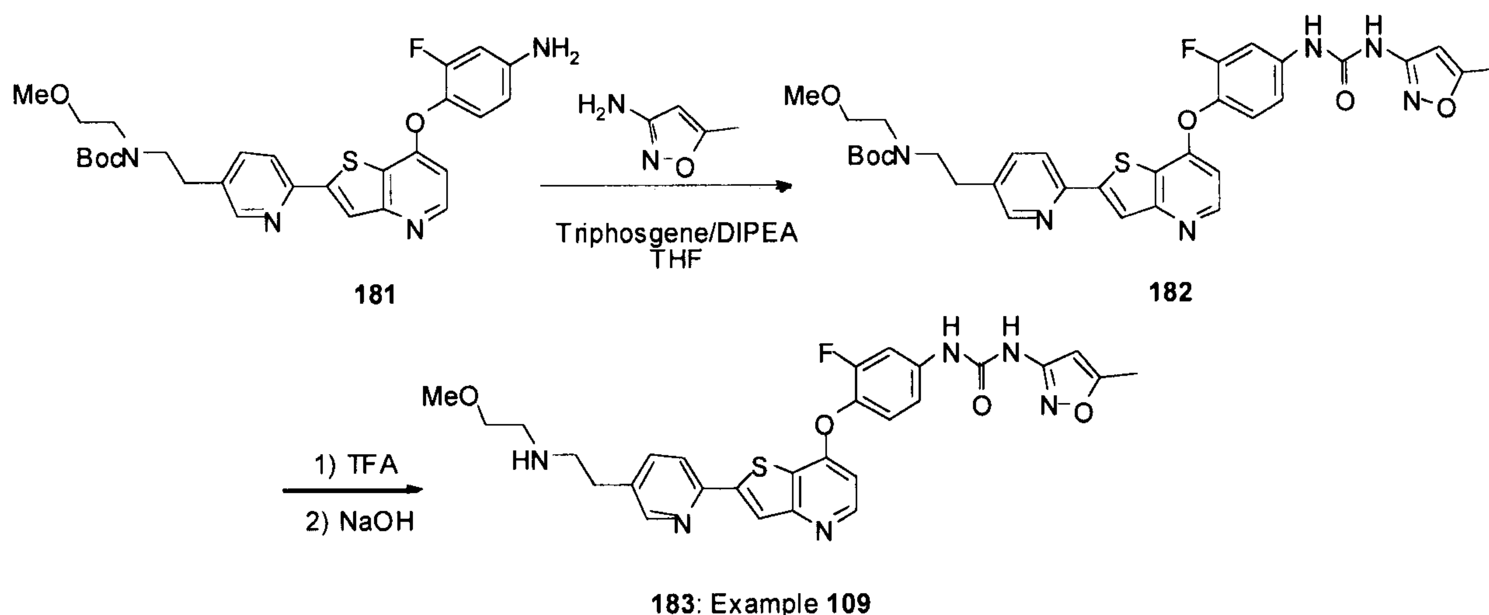
Scheme 44
