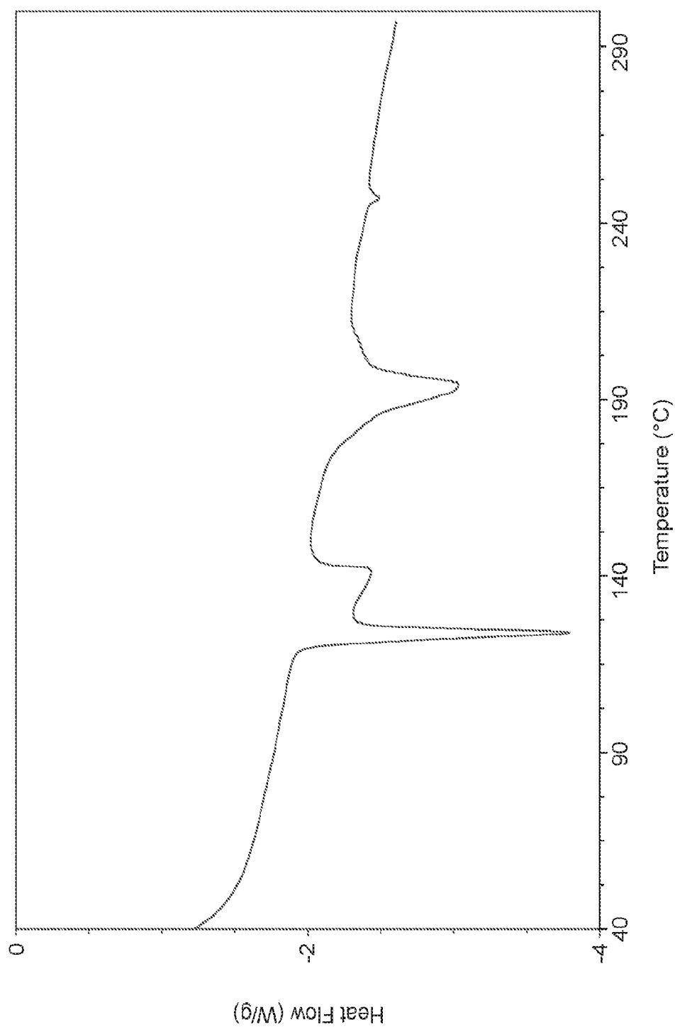
Figure 20 DSC thermogram of Compound 1:triacetin
