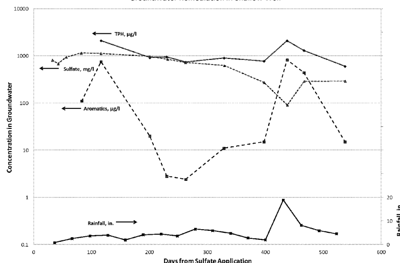
Fig. 1 Groundwater Remediation in Shallow Well
